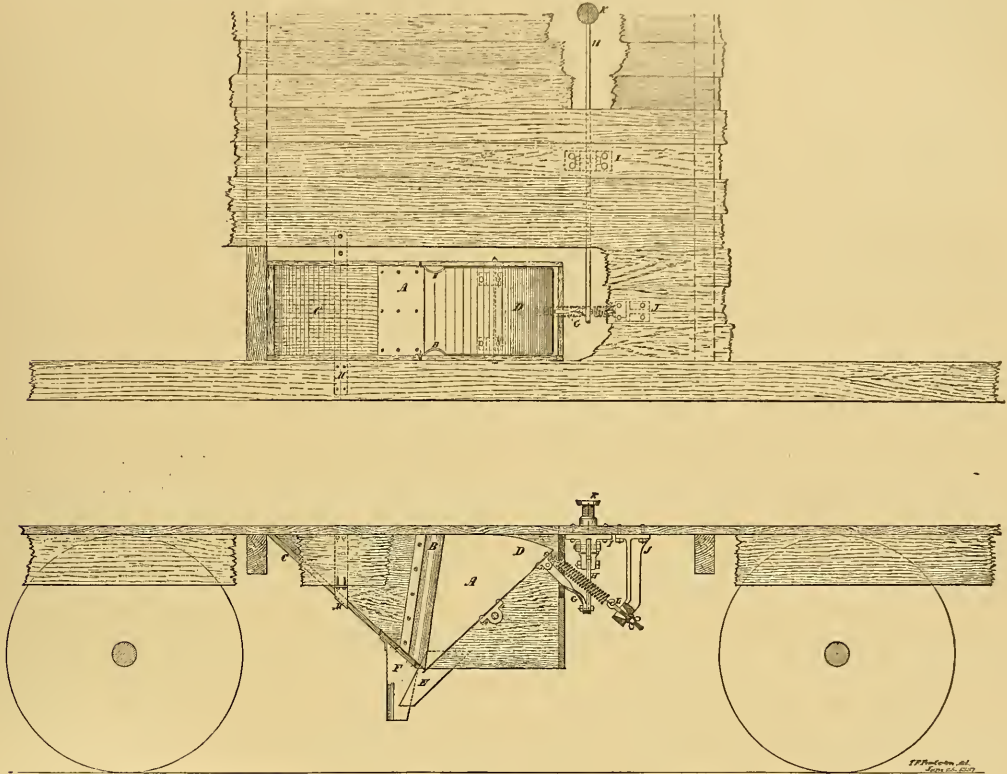
“THE RELIABLE” SAND BOX.
