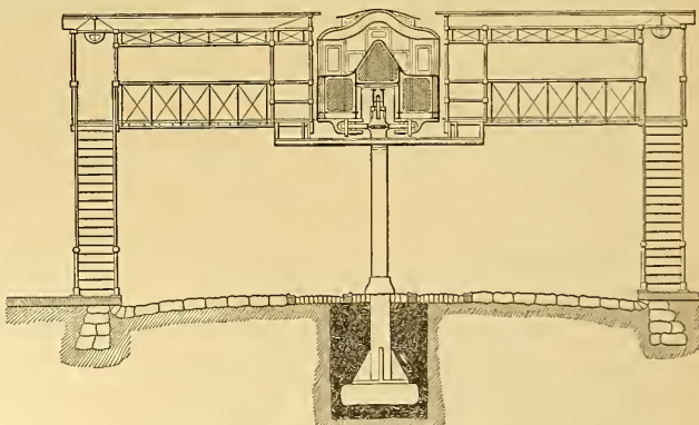
FIG. 3.—ADAMS’ ELEVATED RAILWAY.
