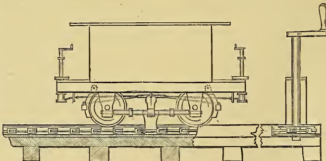
FIG. 2. A. C. BEACH'S STREET RAILWAY, 1864.
