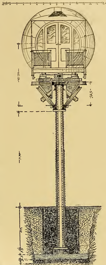
The above cut is an end representation of the car upon the track—its trucks, the post, and its setting; showing the trucks astride of the track 48 inches.
