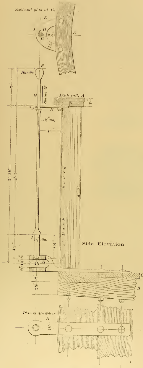
IMPROVED COUPLING DEVICE.
