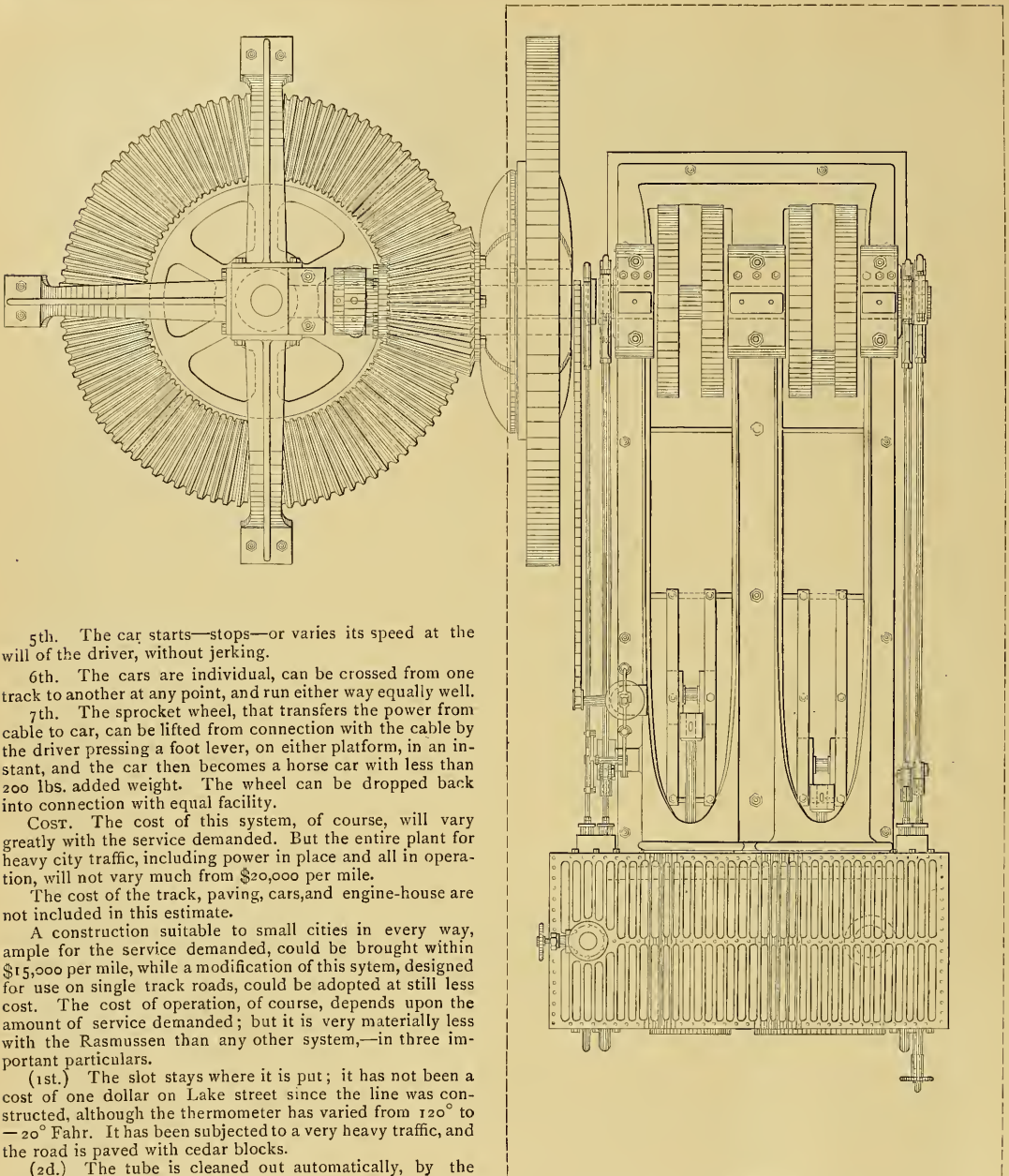
FIG. 7.—PLAN ENGINE DRIVING DRUM.
