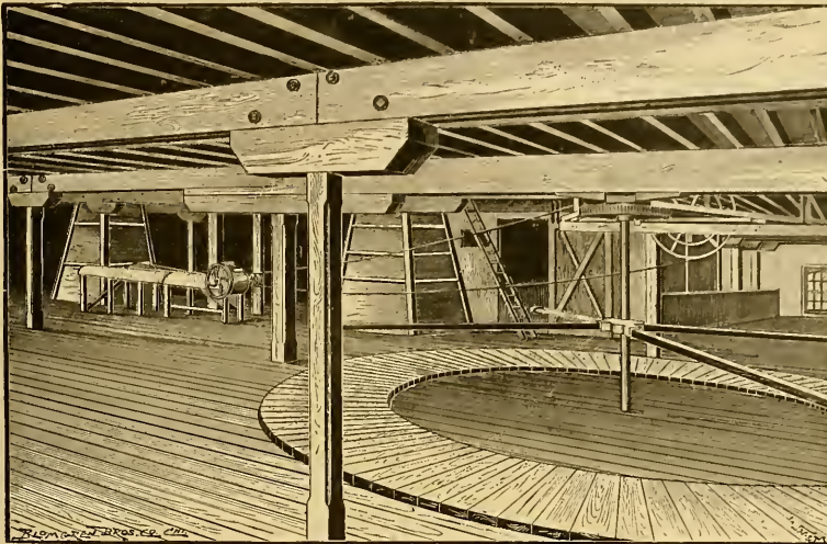
FIG. 59.—ELEVATION OF FEEDING DEPARTMENT.
