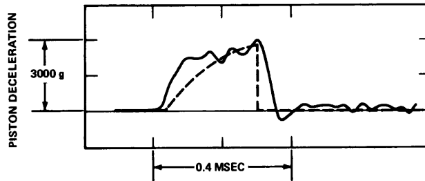
Figure 11 – Piston Acceleration versus Time
