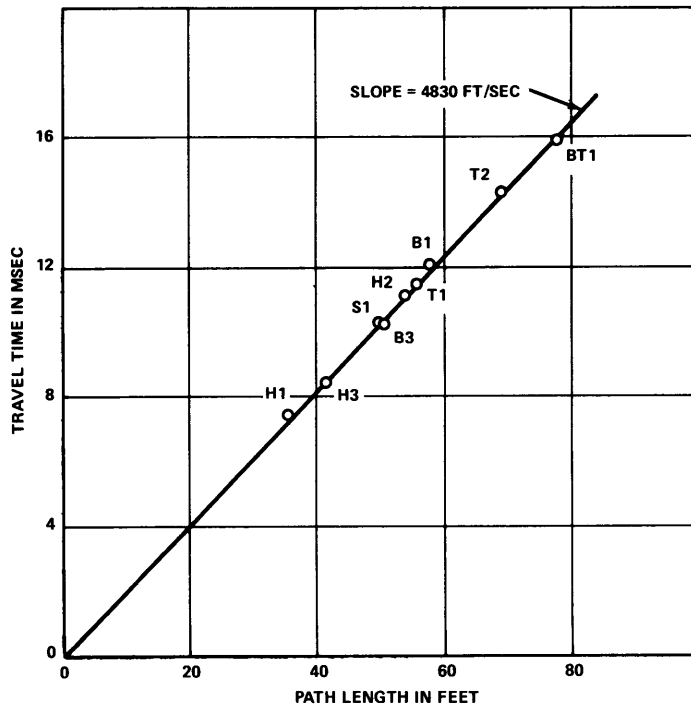
Figure 10 – Path Length versus Travel Time for Hydrophone Pulses
