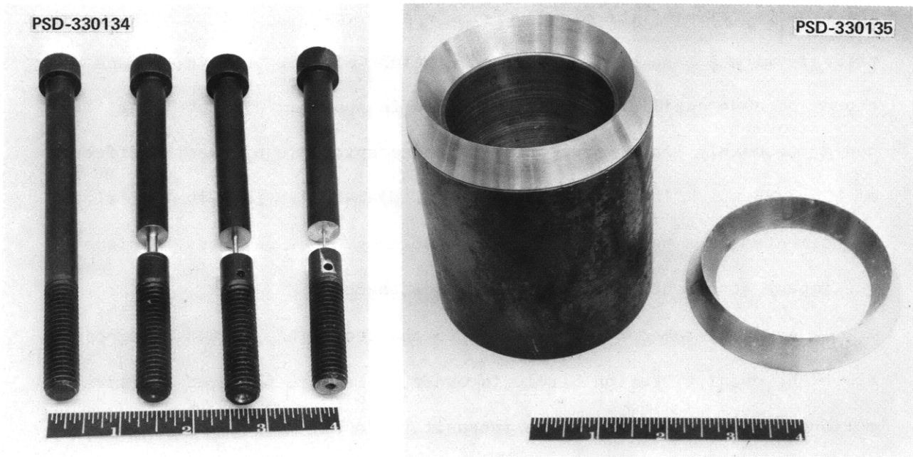
Figure 4 – Breakbolts and Aluminum Rings
