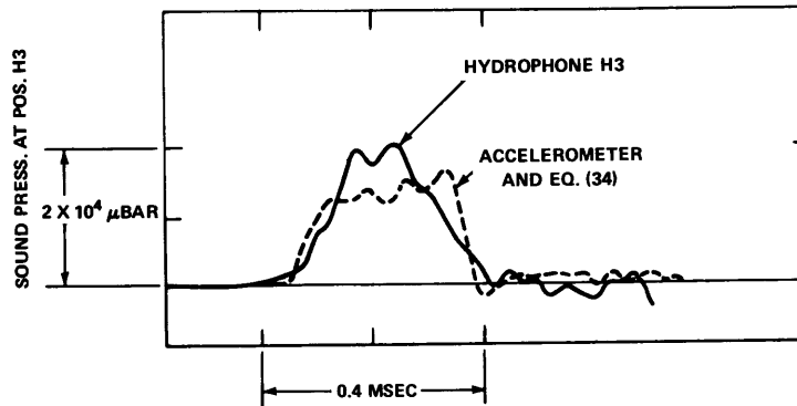
Figure 13 – Comparison of Sound Pressure Measured at Off-Side Hydrophone with Theoretical Monopole Component
