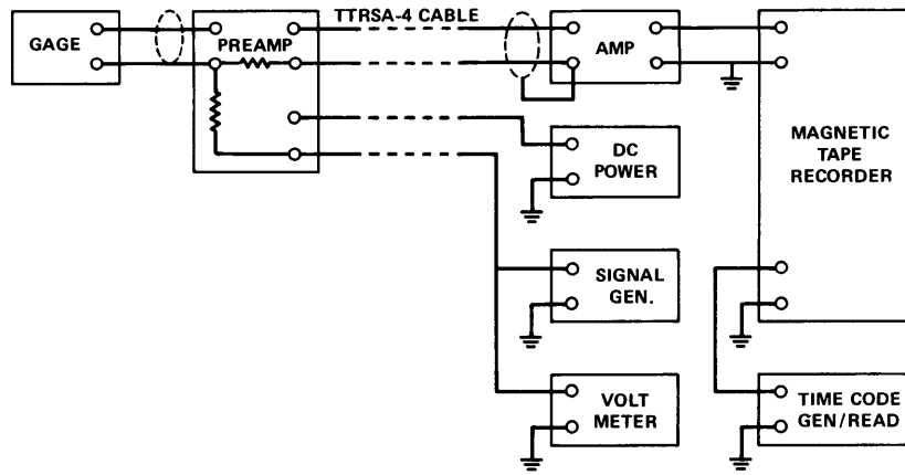
Figure 7 – Block Diagram of Instrumentation
