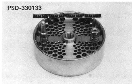
Figure 5 – Piston with Accelerometer and Balance Weight
