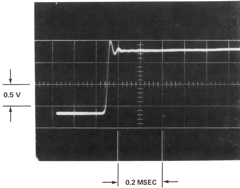
Figure 15 – Voltage Calibration Signals for Acceleration Channel
