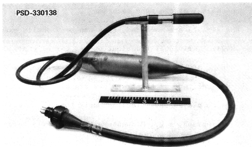
Figure 6 – Hydrophone and Preamplifier
