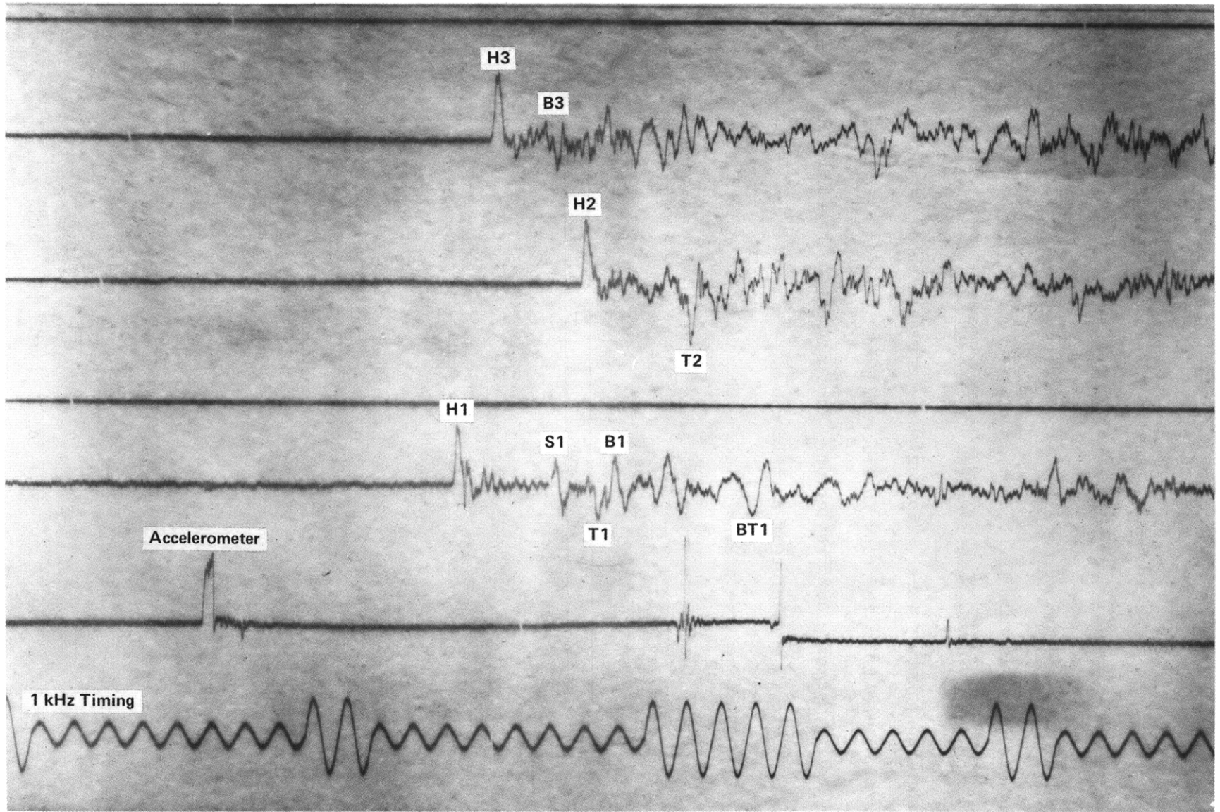
Figure 9 – Accelerometer and Hydrophone Records During Implosion Test
