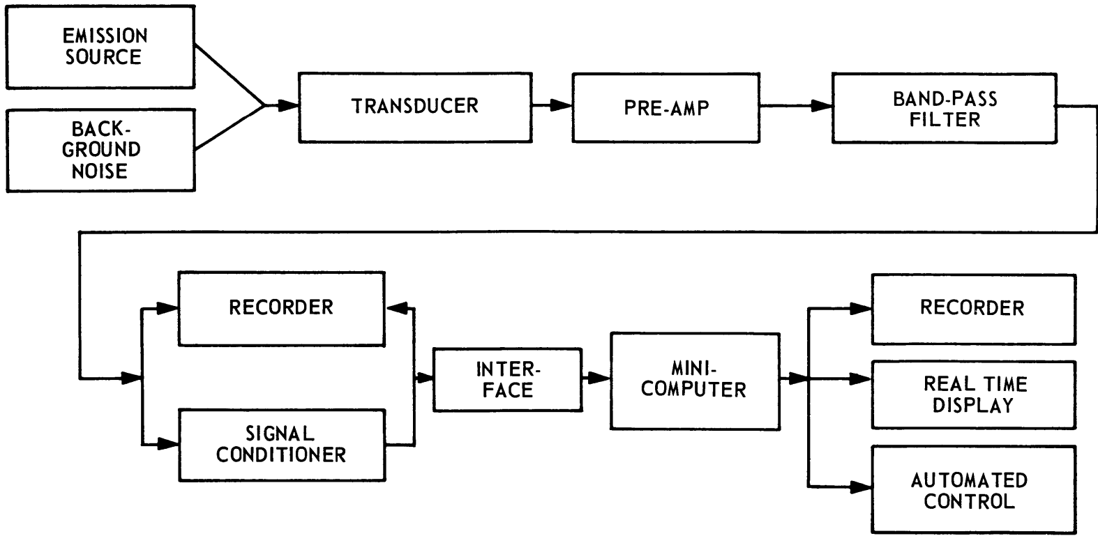
Figure 5 - Schematic of System for Monitoring Stress Wave Emissions
