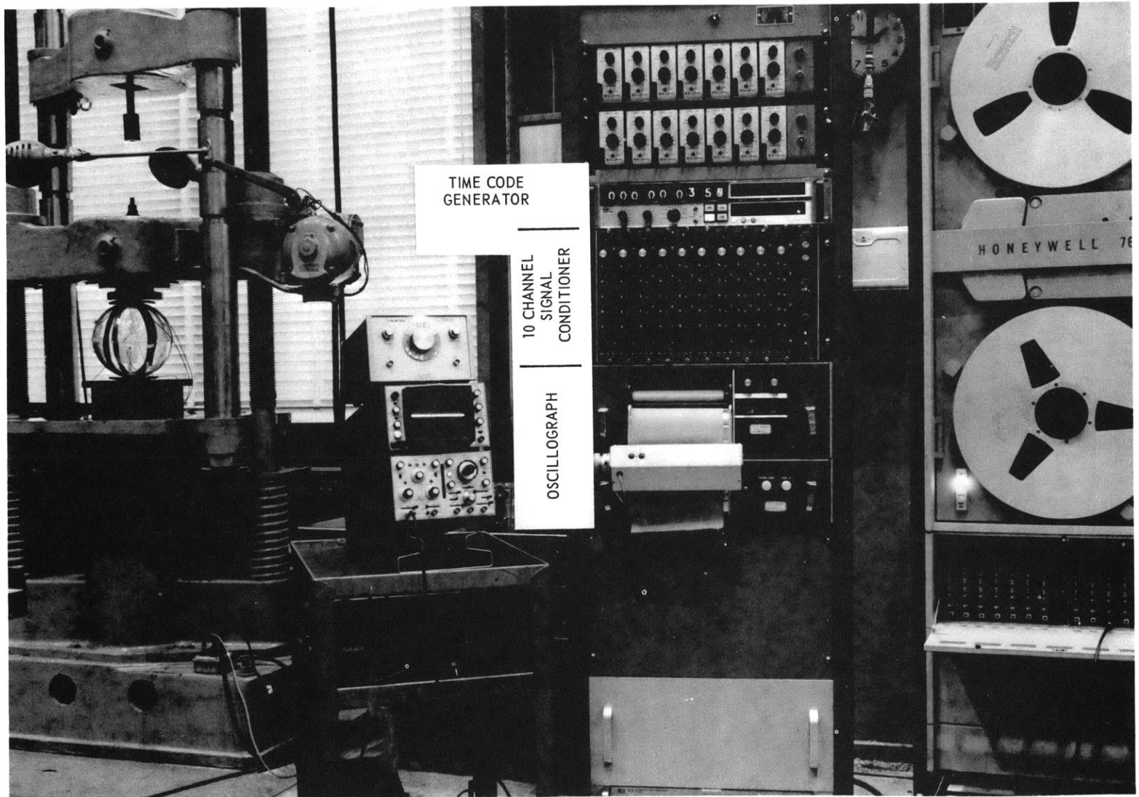
Figure 14 - System for Monitoring Stress Wave Emissions
