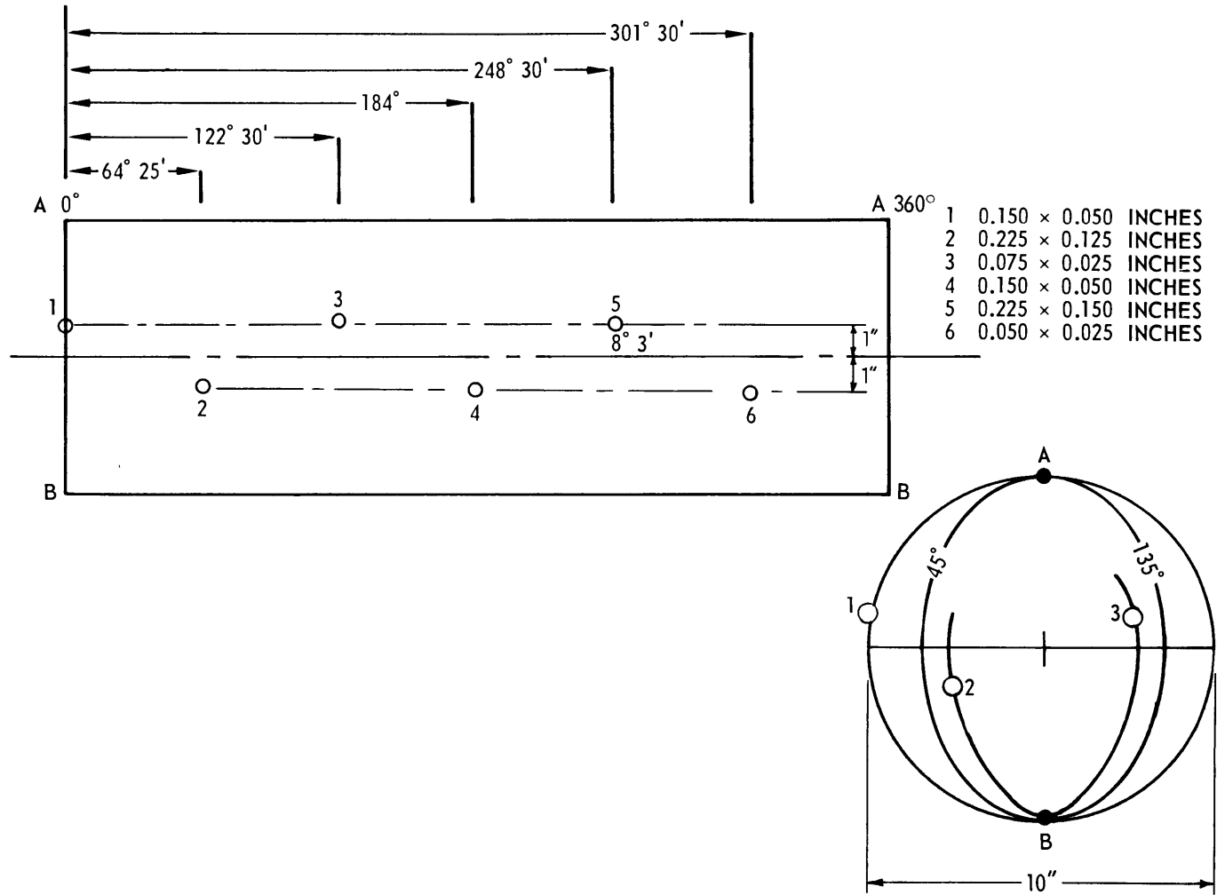
Figure 16 - Transducer Layout on Glass Hemispheres
