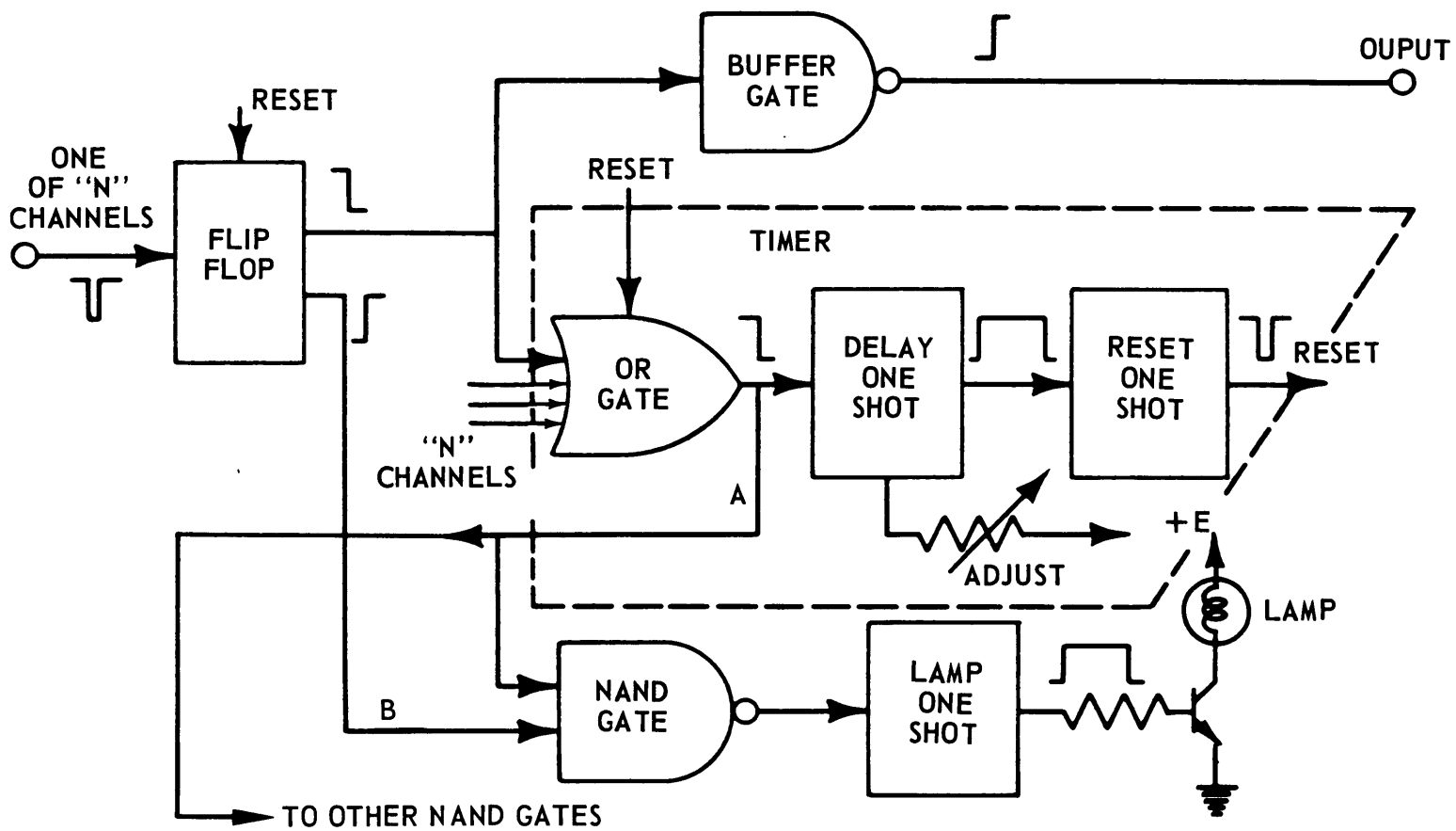
Figure 13 - Schematic of Recycle Timer
