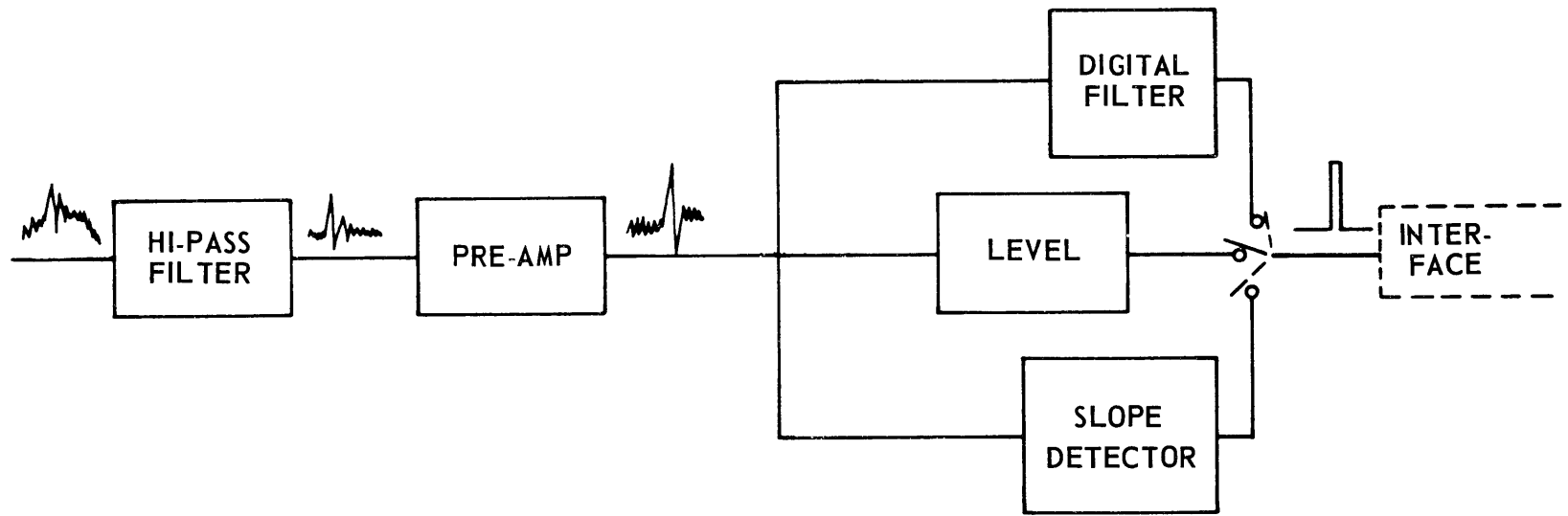
Figure 8 - Schematic of Signal Conditioner
