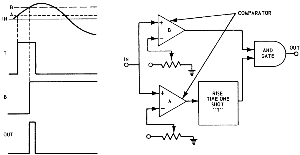
Figure 11a - Principle of Operation Figure 11b - Electronic Schematic
