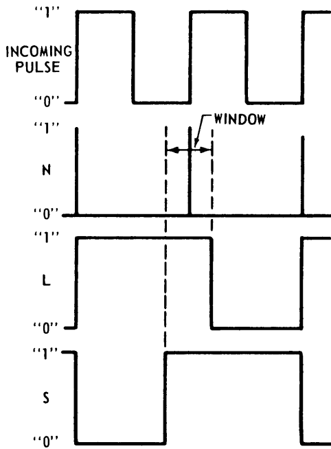
Figure 10a - Principle of Operation
