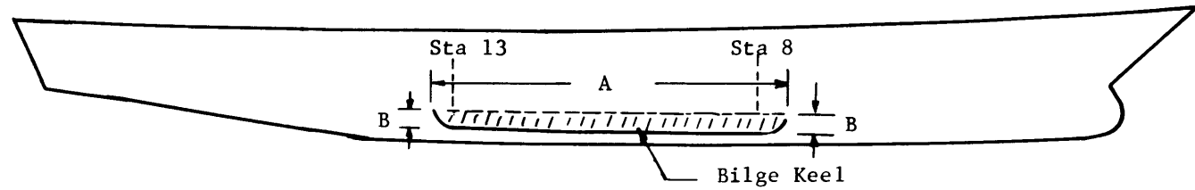
Figure 3a - USS BELKNAP (DLG-26)
