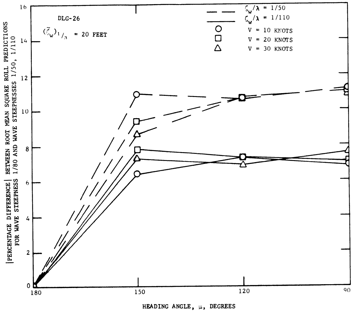
Figure 10 – Percentage Differences Between Roll Predictions at Wave Steepnesses 1/80 and 1/50 and 1/80 and 1/110 for the USS BELKNAP (DLG-26) in Irregular Seas
