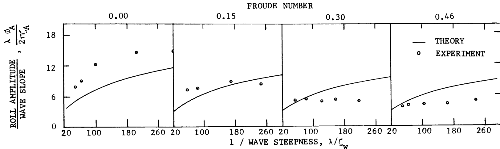
Figure 9a – Nondimensional Roll-Transfer Function versus 1/Wave Steepness at the Natural Roll Frequency
