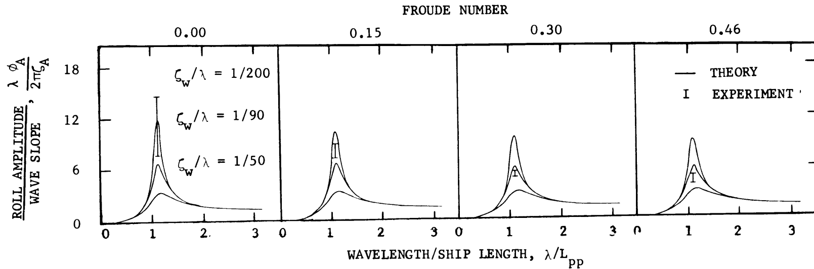
Figure 9b – Nondimensional Roll-Transfer Function versus Wave/Ship Lengths
