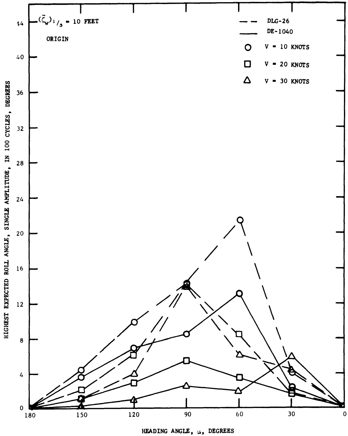
Figure 16 – Comparison of Highest Expected Roll, Single Amplitudes, in 100 Cycles for BELKNAP and GARCIA with Significant Wave Height of 10 Feet
