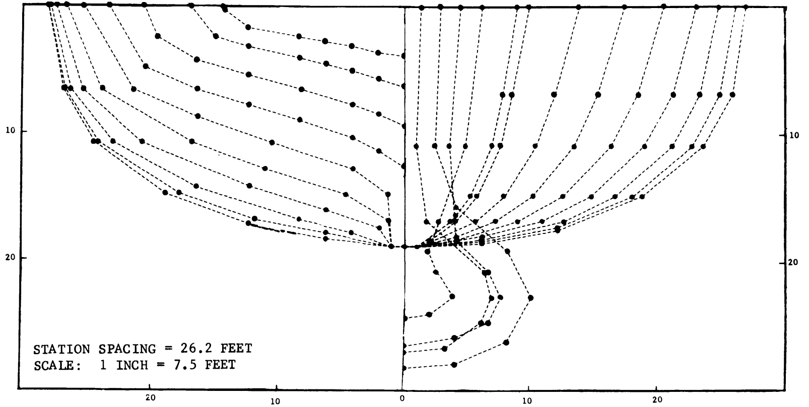
Figure 1 – Computer Fit of USS BELKNAP (DLG-26) Body Plan
