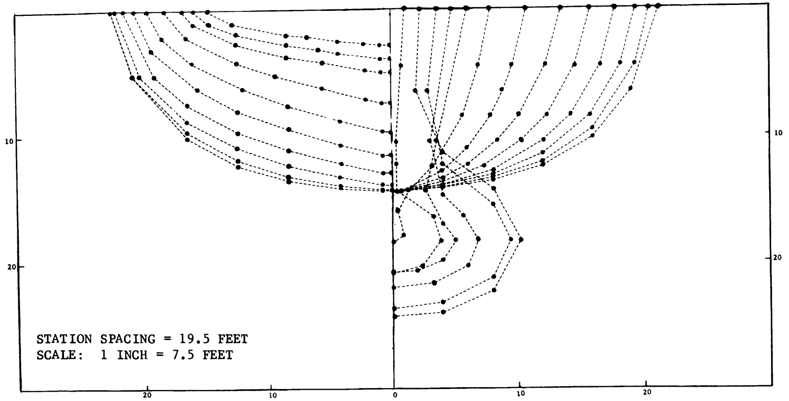
Figure 2 – Computer Fit of USS GARCIA (DE-1040) Body Plan
