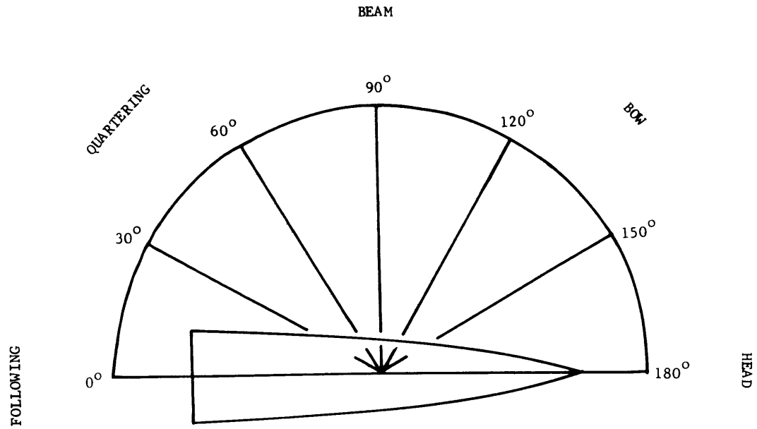
Figure 8 – Incident-Wave Directions with Respect to Ship
