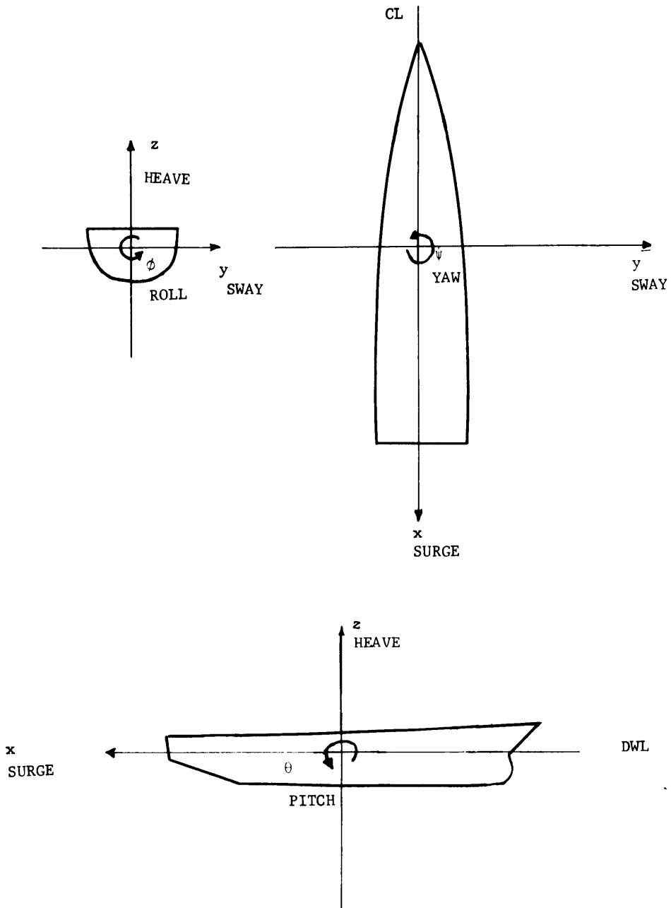
Figure 7 – Right-Handed Coordinate System for Response Predictions
