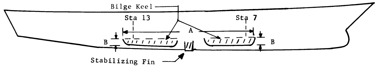
Figure 3b - USS GARCIA (DE-1040)
