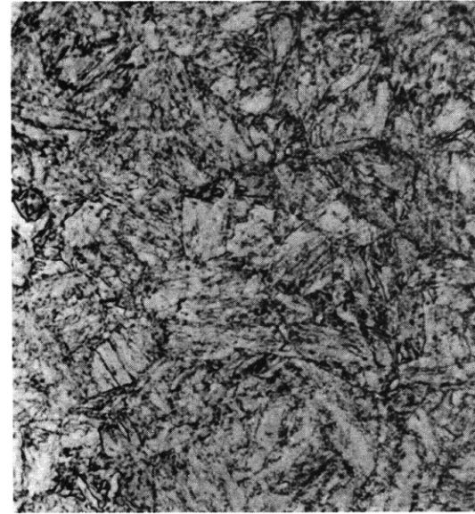
Figure C11d – 100 Percent Martensite 1200 F – 8500 Sec
