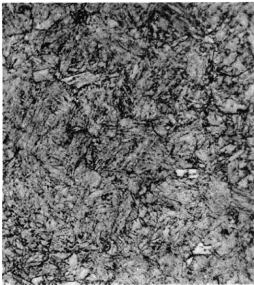
Figure C6c – 100 Percent Martensite 875 F – 152 Sec
