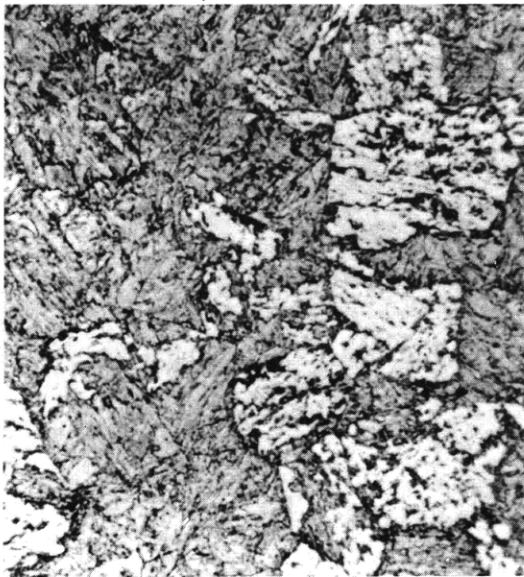
Figure C10c – 27 Percent Bainite – 73 Percent Martensite 875 F – 1600 Sec
