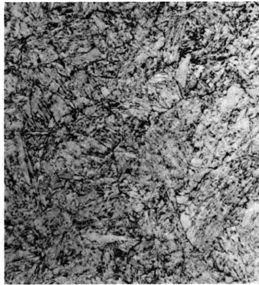
Figure C4b – 100 Percent Martensite 1220 F – 3350 Sec
