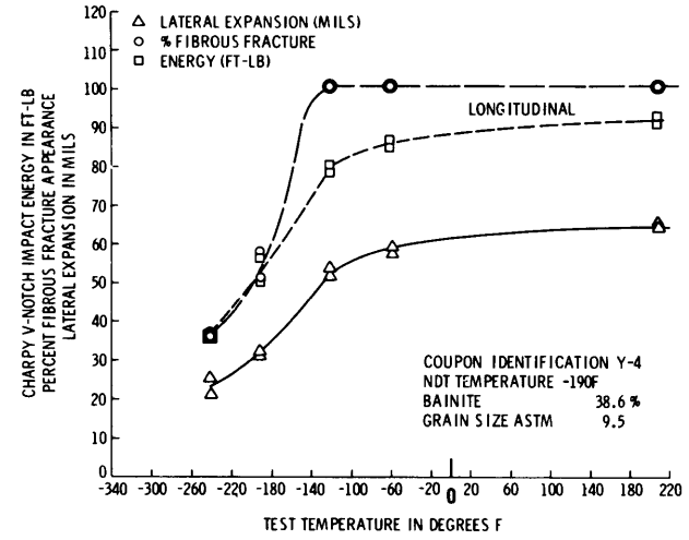
Figure D3 (Continued)
