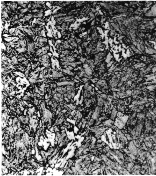
Figure C21c – 4 Percent Bainite – 96 Percent Martensite 875 F – 152 Sec
