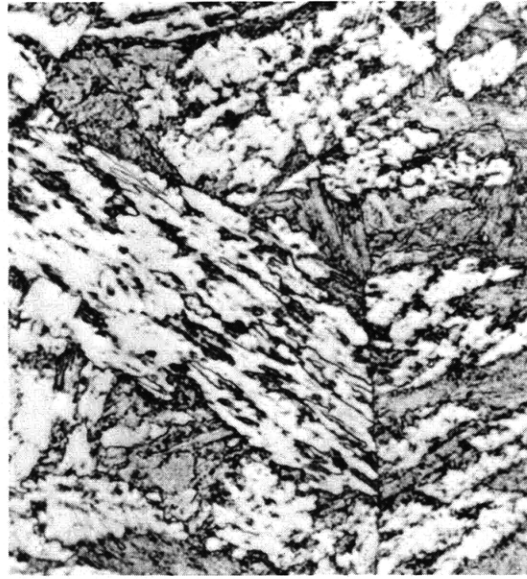
Figure C8b – 63 Percent Bainite – 37 Percent Martensite 875 F – 1600 Sec
