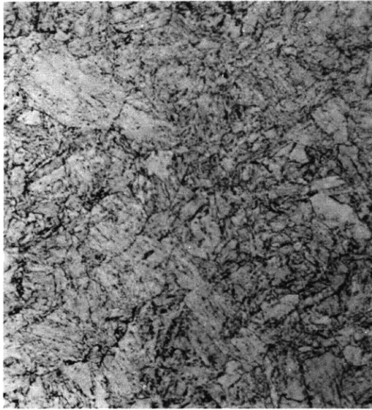
Figure C12a – 100 Percent Martensite 875 F – 152 Sec
