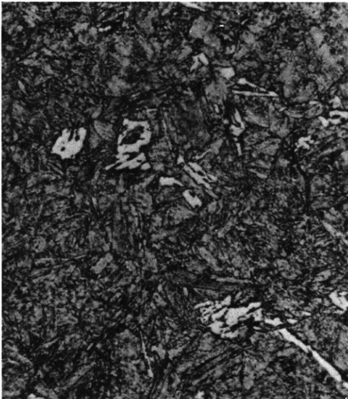
Figure C19c – 1 Percent Bainite – 99 Percent Martensite 875 F – 152 Sec
