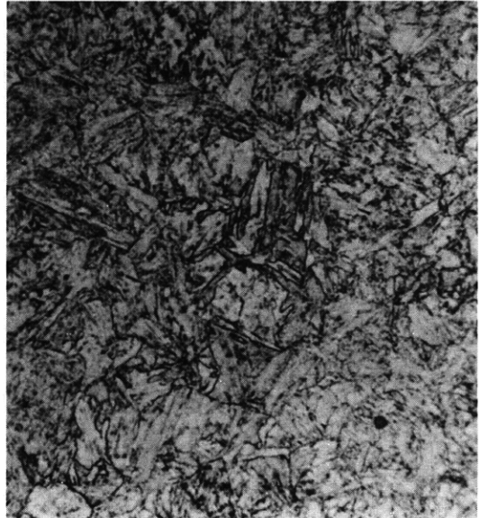
Figure C15d – 100 Percent Martensite 1200 F – 8500 Sec
