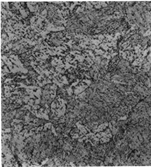
Figure C18c – 39 Percent Bainite – 61 Percent Martensite 875 F – 1600 Sec
