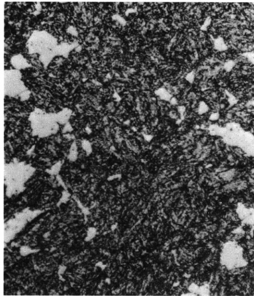
Figure C19b – 17 Percent Ferrite – 83 Percent Martensite 1200 F – 3350 Sec
