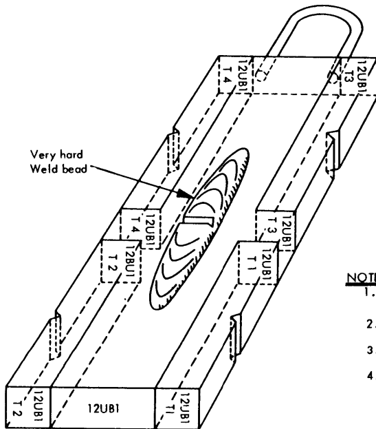
Figure 3b – Details of Layout of Charpy V-Notch Specimens
