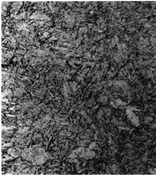
Figure C14a – 100 Percent Martensite 875 F – 152 Sec
