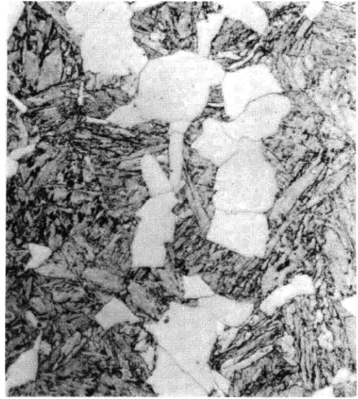
Figure C3b – 31 Percent Ferrite – 60 Percent Martensite 1200 F – 3350 Sec
