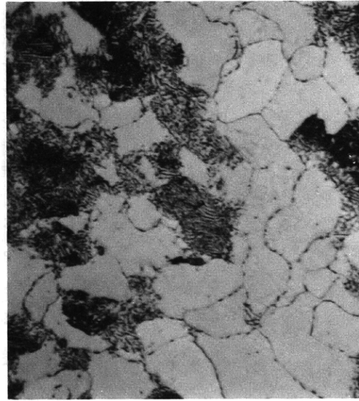
Figure C16d – 69 Percent Ferrite – 23 Percent Pearlite 8 Percent Martensite 1200 F – 3350 Sec
