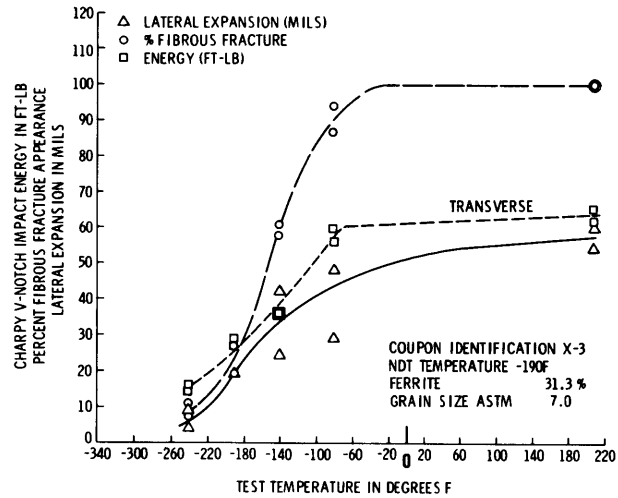
Figure D1 – Transverse and Longitudinal Charpy V-Notch Impact Data for Specimens Austenitized at 1640 F for 1/2 Hour, Water Quenched and Tempered at 1150 F for 1 Hour
