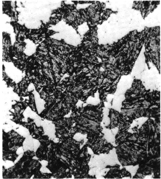
Figure C1b – 31 Percent Ferrite – 69 Percent Martensite 1200 F – 3350 Sec
