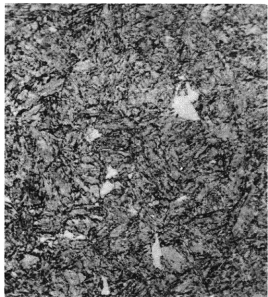
Figure C9b – Trace Ferrite – 100 Percent Martensite 1200 F – 3350 Sec
