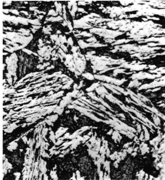
Figure C8d – 67 Percent Bainite – 33 Percent Martensite 875 F – 1600 Sec
