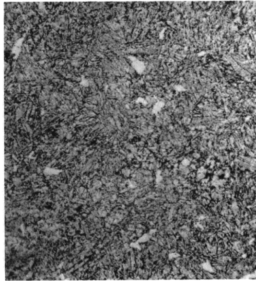
Figure C18b – 7 Percent Ferrite – 93 Percent Martensite 1200 F – 3350 Sec
