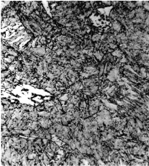
Figure C3c – 2 Percent Bainite – 98 Percent Martensite 875 F – 152 Sec
