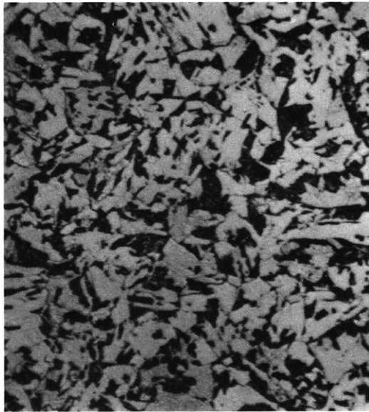
Figure C16c – 76 Percent Bainite – 24 Percent Martensite 875 F – 152 Sec
