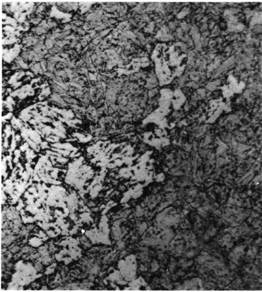
Figure C13a – 16 Percent Bainite – 84 Percent Martensite 875 F – 1600 Sec
