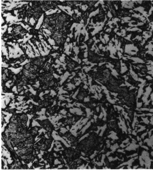
Figure C16a – 53 Percent Bainite – 47 Percent Martensite 875 F – 152 Sec
