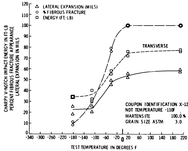
Figure D6 – Transverse Charpy V-Notch Impact Data for Specimens Austenitized at 2000 F for 1 Hour, Transferred to 1640 F for 5 Minutes Minimum, Water Quenched and Tempered at 1100 F for 1 Hour
