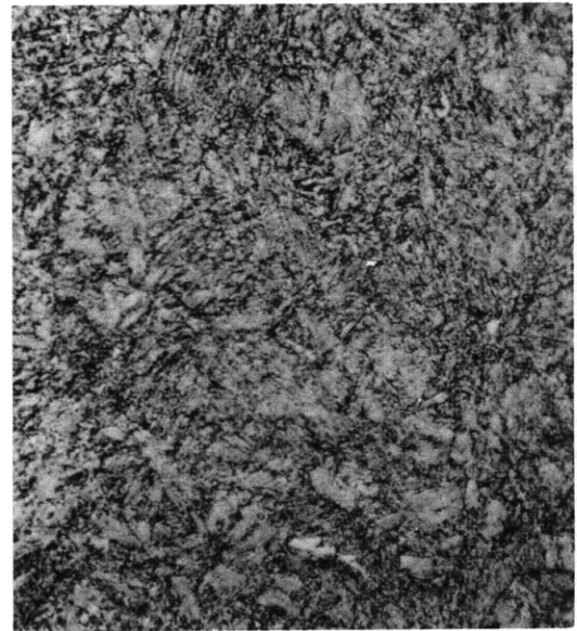
Figure C7b – Trace Ferrite – 100 Percent Martensite 1200 F – 3550 Sec
