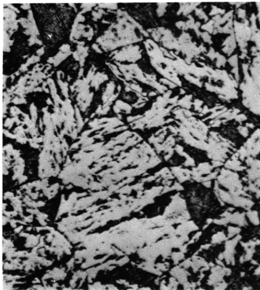
Figure C22c – 63 Percent Bainite – 37 Percent Martensite 875 F – 1600 Sec
