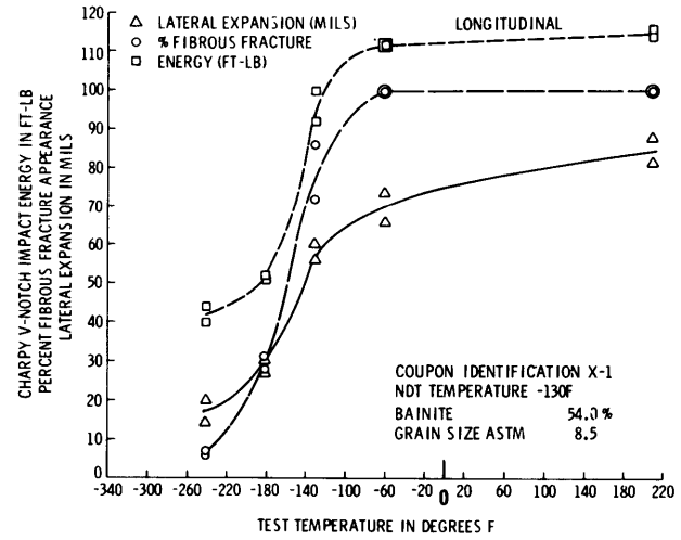
Figure D3 – Transverse and Longitudinal Charpy V-Notch Impact Data for Specimens Austenitized at 1640 F for 1/2 Hour, Isothermally Treated at 875 F for 1600 Seconds, Water Quenched and Tempered at 1150 F for 1 Hour
