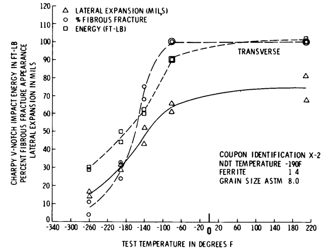
Figure D5 – Transverse Charpy V-Notch Impact Data for Specimens Austenitized at 1640 F for 1/2 Hour, Isothermally Treated at 1200 F for 8500 Seconds, Water Quenched and Tempered at 1150 F for 1 Hour
