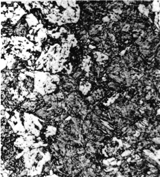
Figure C15c – 21 Percent Bainite – 79 Percent Martensite 875 F – 1600 Sec
