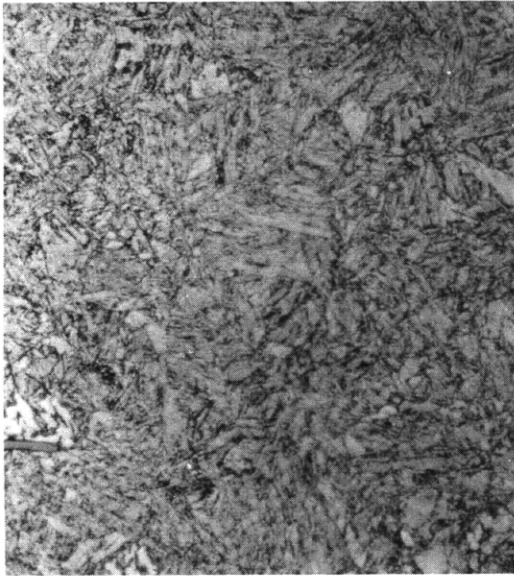
Figure C18a – 1 Percent Bainite – 99 Percent Martensite 875 F – 152 Sec
