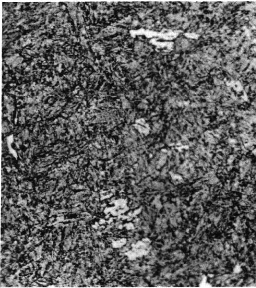
Figure C20a – 1 Percent Bainite – 99 Percent Martensite 875 F – 152 Sec
