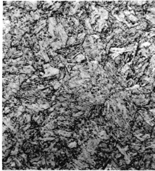
Figure C14b – 100 Percent Martensite 1200 F – 3350 Sec
