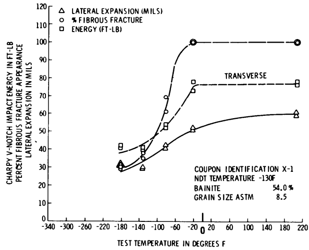
Figure D3 – Transverse and Longitudinal Charpy V-Notch Impact Data for Specimens Austenitized at 1640 F for 1/2 Hour, Isothermally Treated at 875 F for 1600 Seconds, Water Quenched and Tempered at 1150 F for 1 Hour
