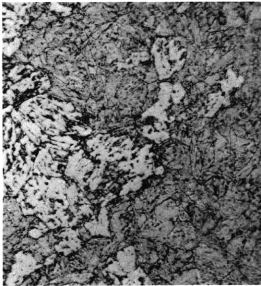
Figure C12c – 16 Percent Bainite – 84 Percent Martensite 875 F – 1600 Sec
