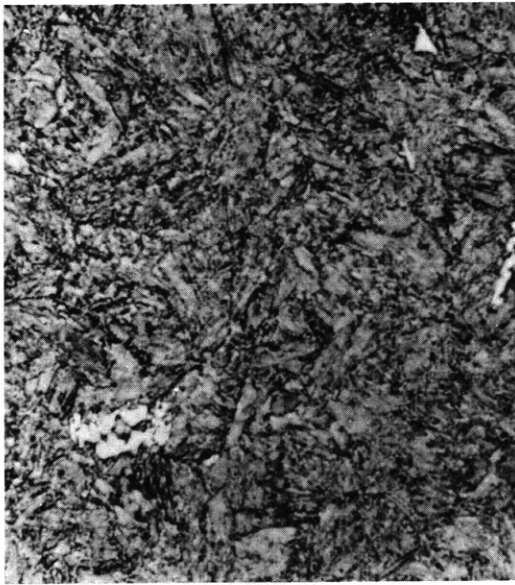
Figure C7a – 1 Percent Bainite – 99 Percent Martensite 875 F – 152 Sec
