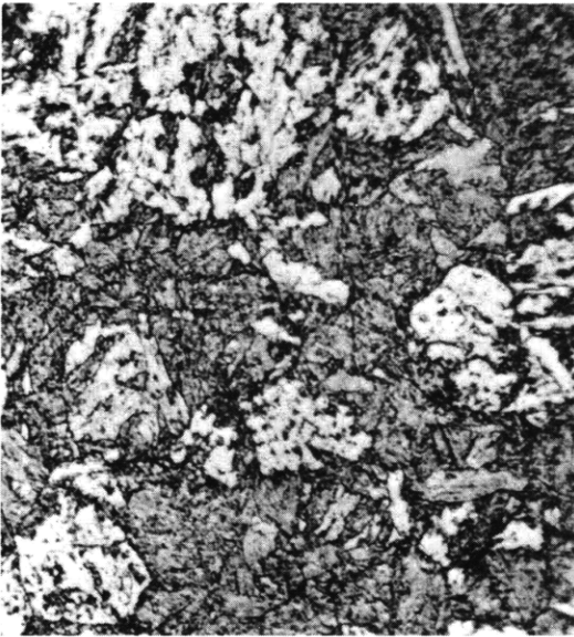
Figure C13c – 32 Percent Bainite – 68 Percent Martensite 875 F – 1600 Sec
