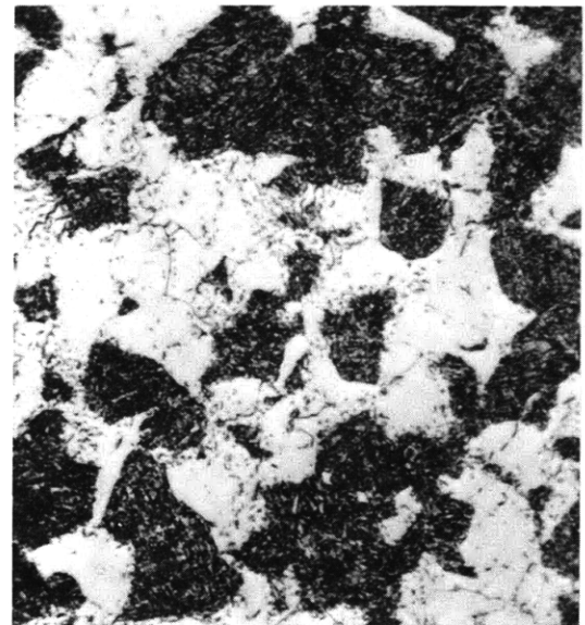
Figure C17d – 53 Percent Ferrite – 4 Percent Pearlite 43 Percent Martensite 1200 F – 8500 Sec
