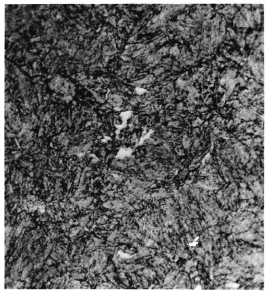
Figure C21d – 1 Percent Ferrite – 99 Percent Martensite 1200 F – 3350 Sec
