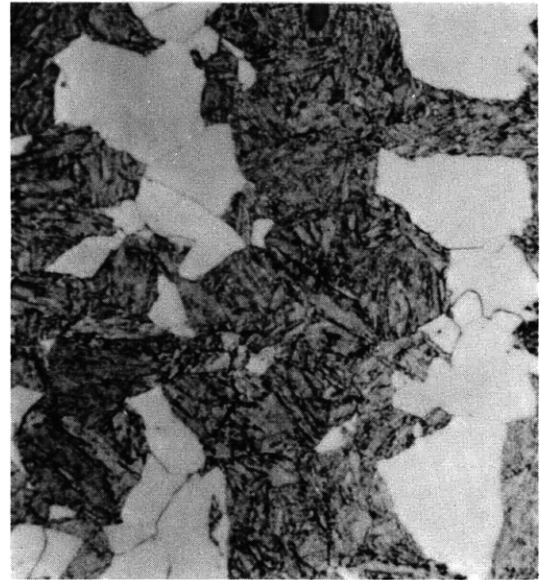
Figure C5d – 26 Percent Ferrite – 74 Percent Martensite 1200 F – 3350 Sec
