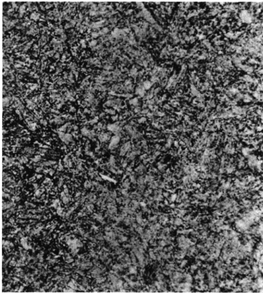
Figure C15a – Trace Bainite – 100 Percent Martensite 875 F – 152 Sec
