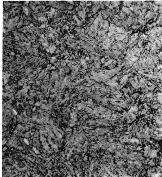
Figure C14d – Trace Ferrite – 100 Percent Martensite 1200 F – 8500 Sec
