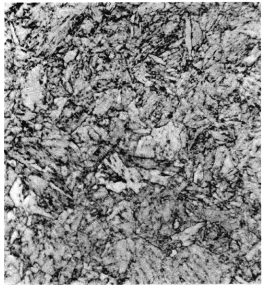
Figure C15b – 100 Percent Martensite 1200 F – 3350 Sec
