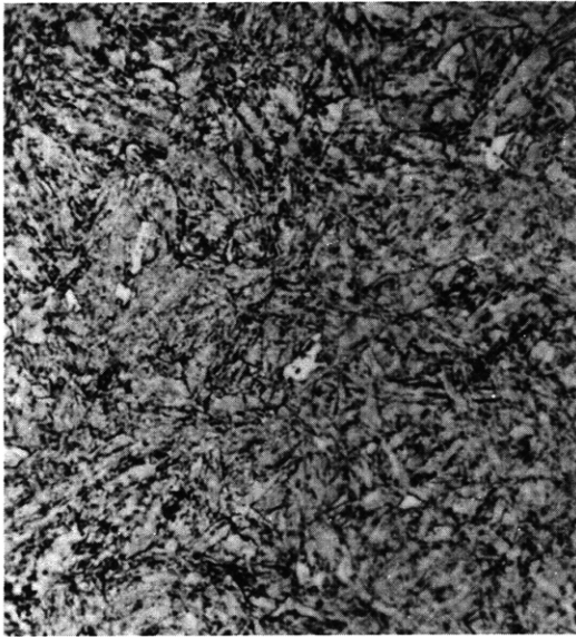
Figure C4a – 1 Percent Bainite – 99 Percent Martensite 875 F – 152 Sec
