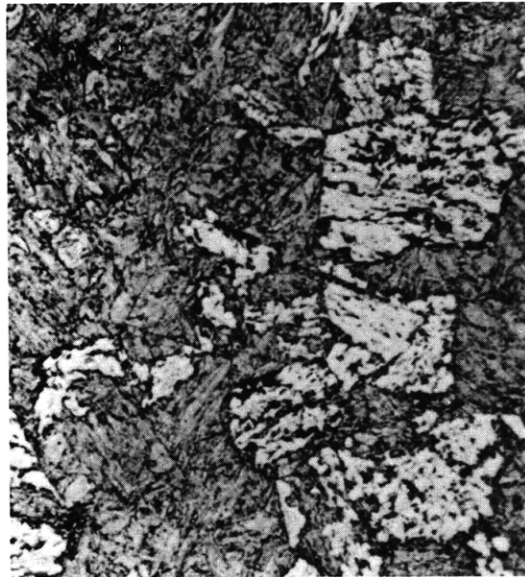
Figure C11c – 27 Percent Bainite – 73 Percent Martensite 875 F – 1600 Sec
