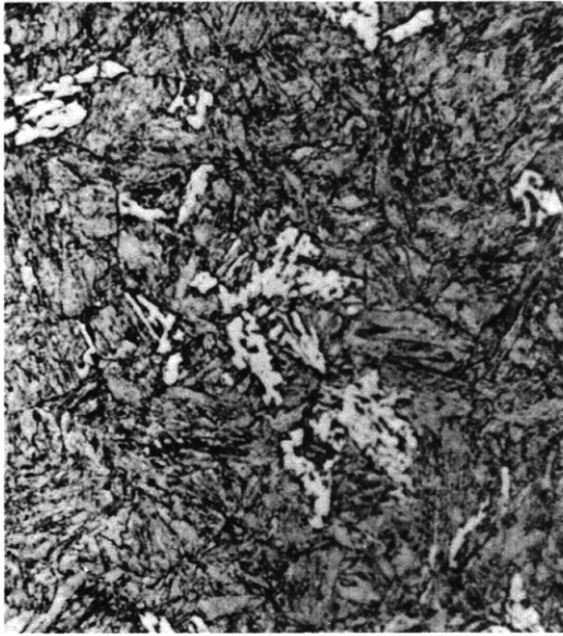
Figure C21a – 6 Percent Bainite – 94 Percent Martensite 875 F – 152 Sec
