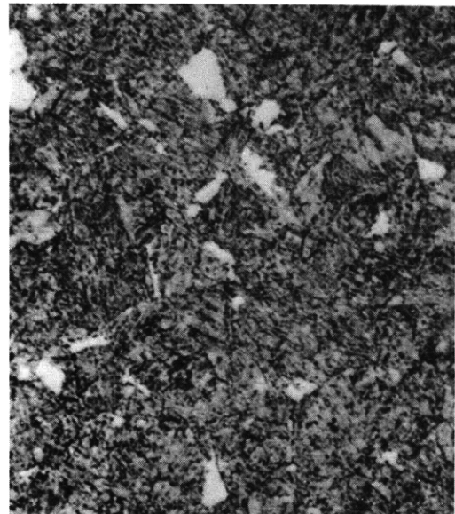
Figure C19d – 12 Percent Ferrite – 88 Percent Martensite 1200 F – 3350 Sec
