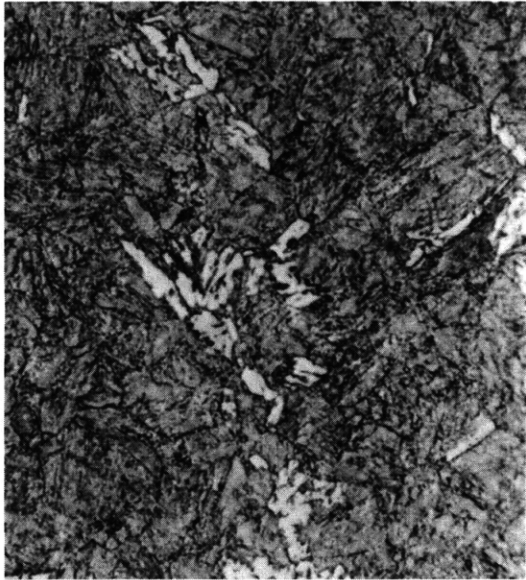
Figure C5c – 7 Percent Bainite – 93 Percent Martensite 875 F – 152 Sec
