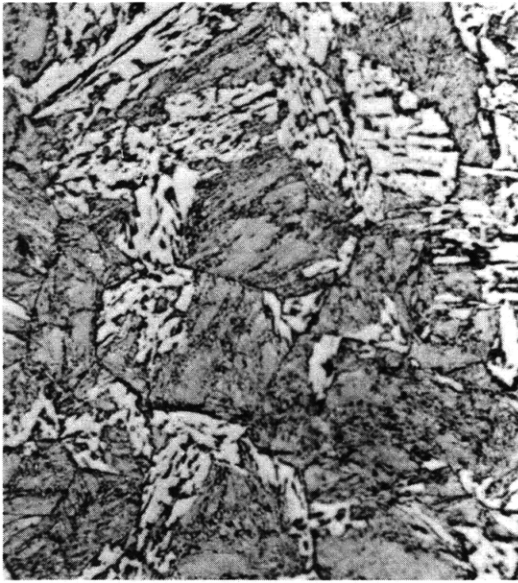
Figure C3a – 21 Percent Bainite – 79 Percent Martensite 875 F – 152 Sec
