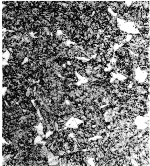
Figure C3d – 11 Percent Ferrite – 89 Percent Martensite 1200 F – 3350 Sec
