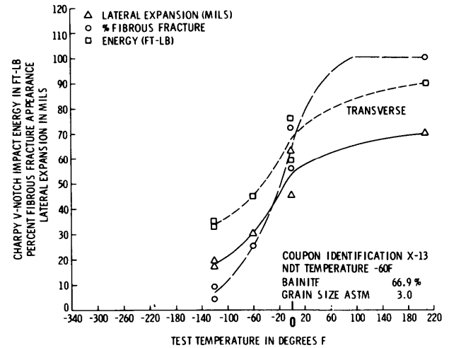
Figure D7 – Transverse Charpy V-Notch Impact Data for Specimens Austenitized at 2000 F for 1 Hour, Transferred to 1640 F for 5 Minutes Minimum, Isothermally Treated at 875 F for 1600 Seconds, Water Quenched and Tempered at 1150 F for 1 Hour
