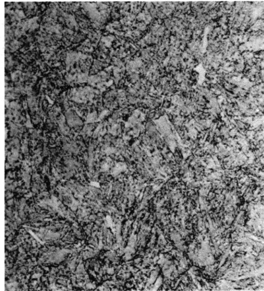
Figure C4d – 1 Percent Ferrite – 99 Percent Martensite 1220 F – 3350 Sec
