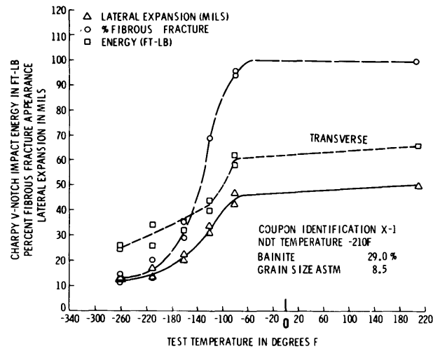
Figure D2 – Transverse Charpy V-Notch Impact Data for Specimens Austenitized at 1640 F for 1/2 Hour, Isothermally Treated at 875 F for 152 Seconds, Water Quenched and Tempered at 1150 F for 1 Hour
