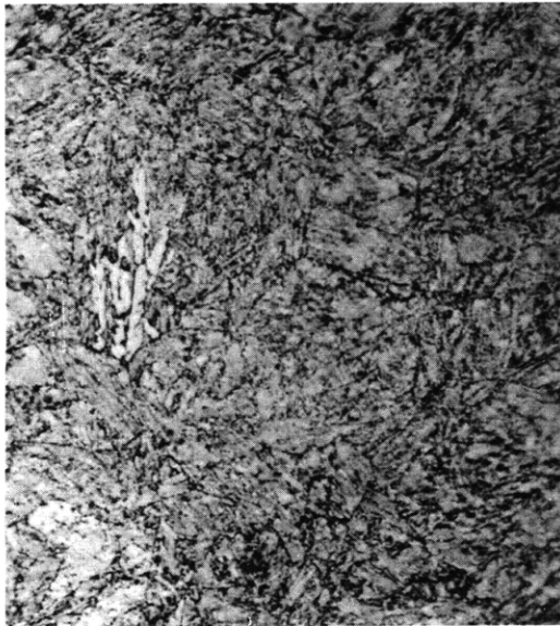
Figure C4c – Trace Bainite – 100 Percent Martensite 875 F – 152 Sec
