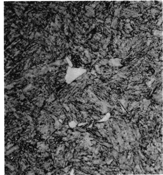
Figure C7d – 1 Percent Ferrite – 99 Percent Martensite 1200 F – 8500 Sec
