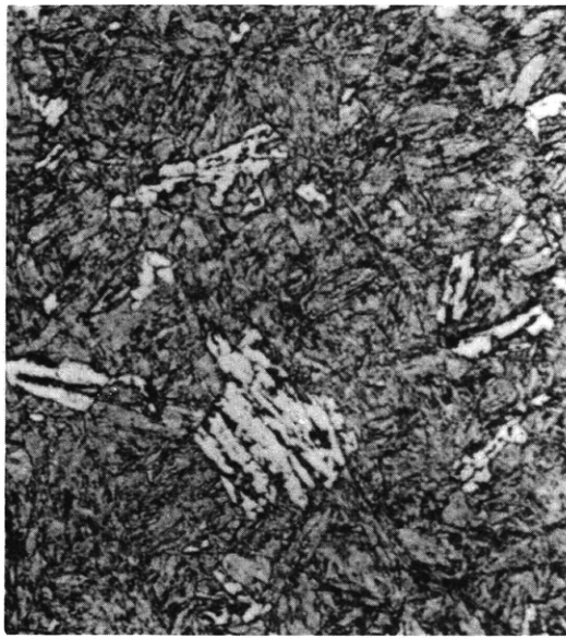
Figure C17a – 9 Percent Bainite – 91 Percent Martensite 875 F – 152 Sec
