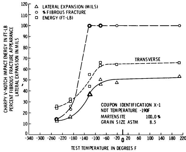
Figure D4 – Transverse Charpy V-Notch Impact Data for Specimens Austenitized at 1640 F for 1/2 Hour, Isothermally Treated at 1200 F for 3350 Seconds, Water Quenched and Tempered at 1150 F for 1 Hour
