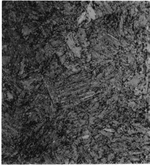
Figure C2d – 2 Percent – 98 Percent Martensite 1200 F – 8500 Sec
