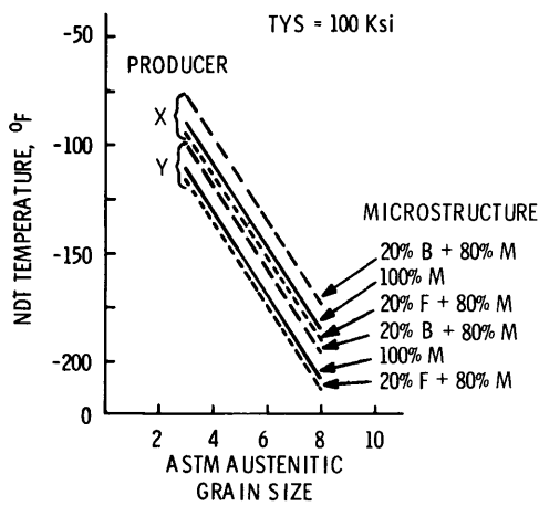
Figure 8a – Functional Relationship between NDT Temperature and Prior Austenitic Grain Size in Terms of Microconstituents and Producer
