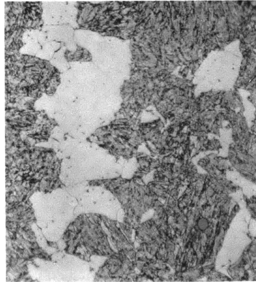
Figure C18d – 21 Percent Ferrite – 79 Percent Martensite 1200 F – 8500 Sec
