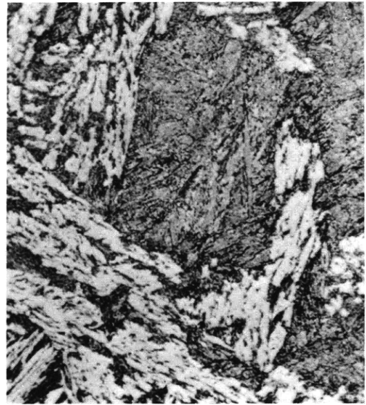
Figure C13b – 58 Percent Bainite – 42 Percent Martensite 875 F – 1600 Sec
