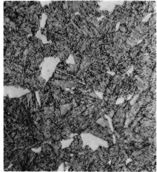
Figure C5b – 5 Percent Ferrite – 95 Percent Martensite 1200 F – 3350 Sec
