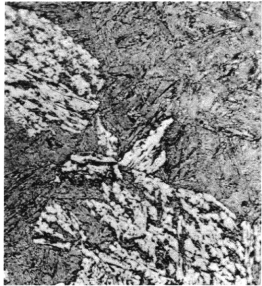
Figure C13d – 30 Percent Bainite – 70 Percent Martensite 875 F – 1600 Sec
