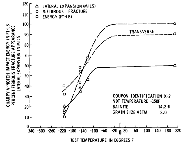
Figure D2 – Transverse Charpy V-Notch Impact Data for Specimens Austenitized at 1640 F for 1/2 Hour, Isothermally Treated at 875 F for 152 Seconds, Water Quenched and Tempered at 1150 F for 1 Hour
