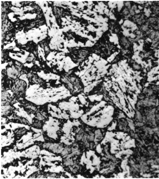
Figure C8a – 50 Percent Bainite – 50 Percent Martensite 875 F – 1600 Sec.
