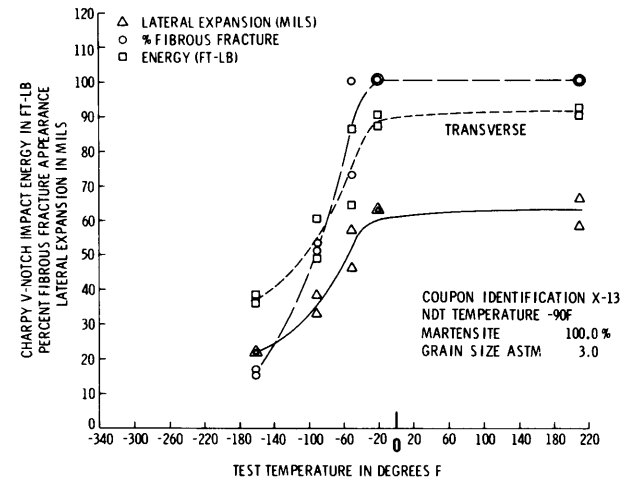
Figure D6 – Transverse Charpy V-Notch Impact Data for Specimens Austenitized at 2000 F for 1 Hour, Transferred to 1640 F for 5 Minutes Minimum, Water Quenched and Tempered at 1100 F for 1 Hour
