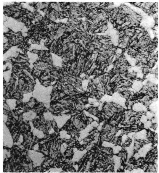
Figure C17b – 22 Percent Ferrite – 78 Percent Martensite 1200 F – 3350 Sec
