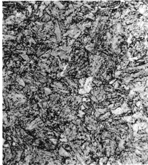
Figure C6b – Trace Ferrite – 100 Percent Martensite 1200 F – 3350 Sec
