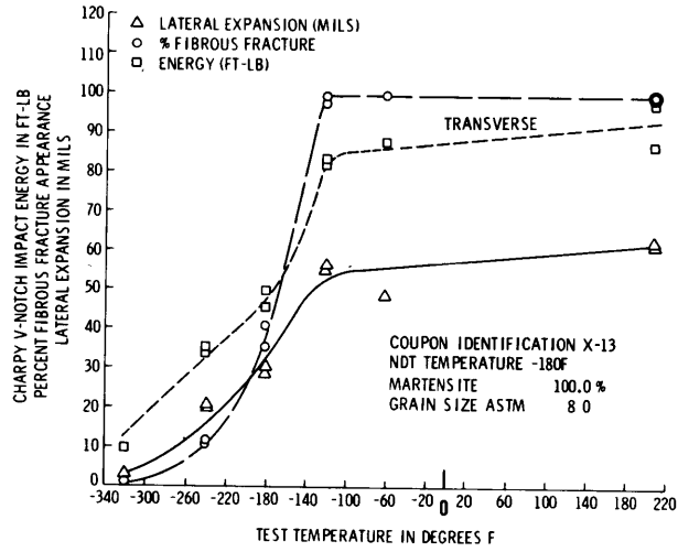
Figure D4 (Continued)
