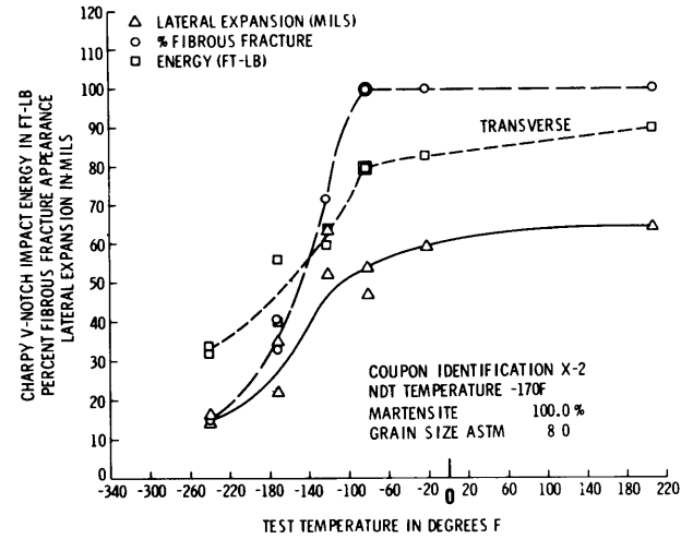
Figure D4 – Transverse Charpy V-Notch Impact Data for Specimens Austenitized at 1640 F for 1/2 Hour, Isothermally Treated at 1200 F for 3350 Seconds, Water Quenched and Tempered at 1150 F for 1 Hour
