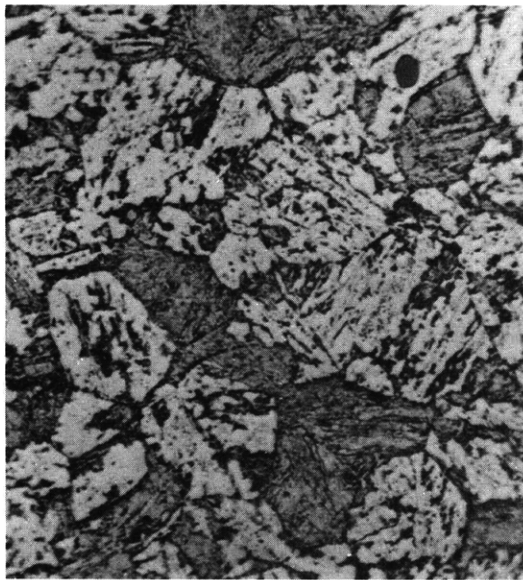
Figure C9c – 60 Percent Bainite – 40 Percent Martensite 875 F – 1600 Sec
