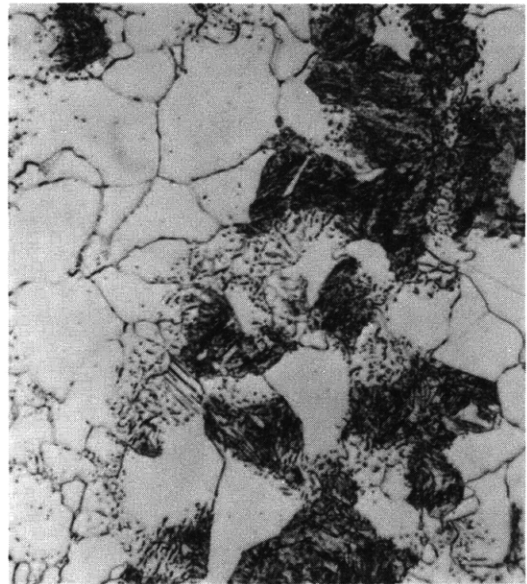
Figure C1d – 67 Percent Ferrite – 11 Percent Pearlite 22 Percent Martensite 1200 F – 8500 Sec
