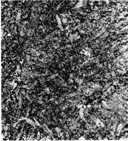
Figure C11a – 1 Percent Bainite – 99 Percent Martensite 875 F – 152 Sec
