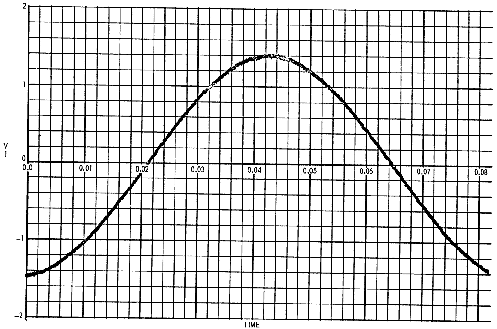
Figure 30 - Partial Computer Plot of File 42 Showing v_1 Points for 10-Hz Sine Wave
