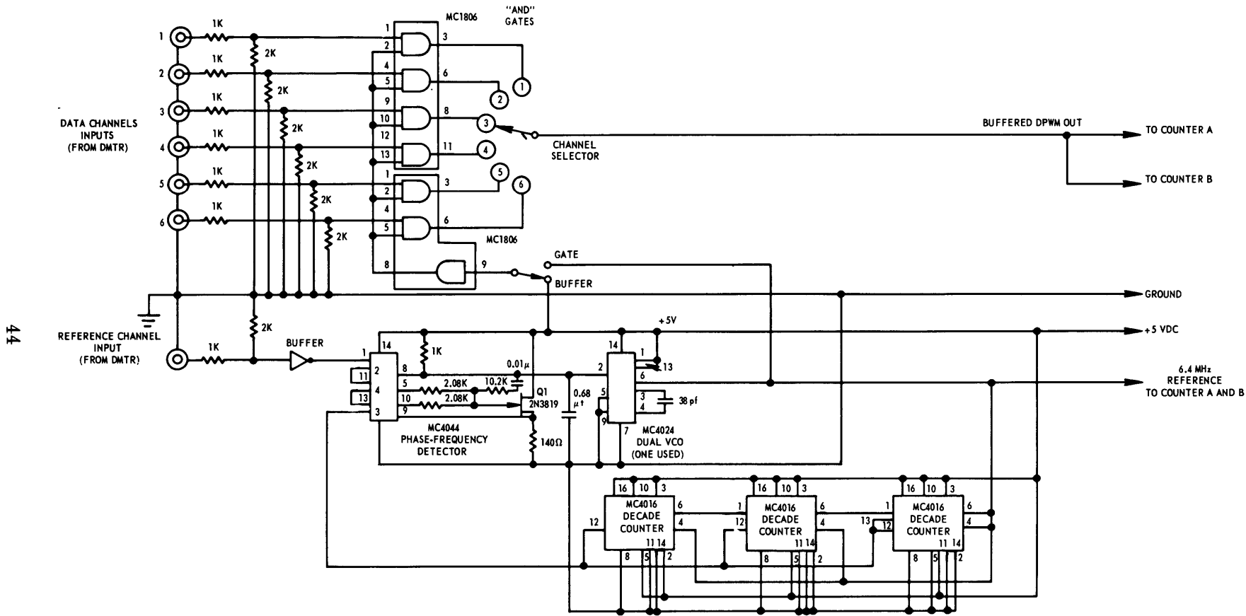
Figure 23 – Digital Interface Electronics – Gating Modules and Phase-Locked Loop
