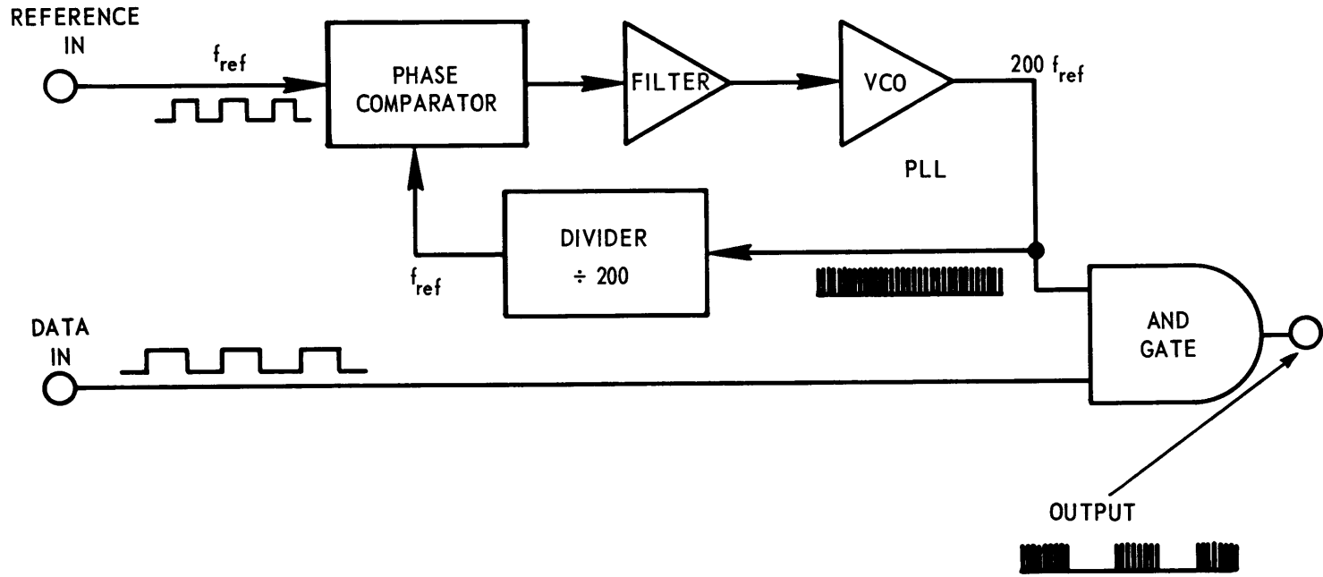
Figure 11 – Typical Digital Demodulation Using a Phase-Locked Loop
