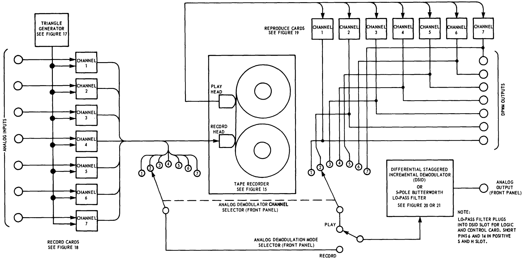
Figure 14 – Model 300 Block Diagram
