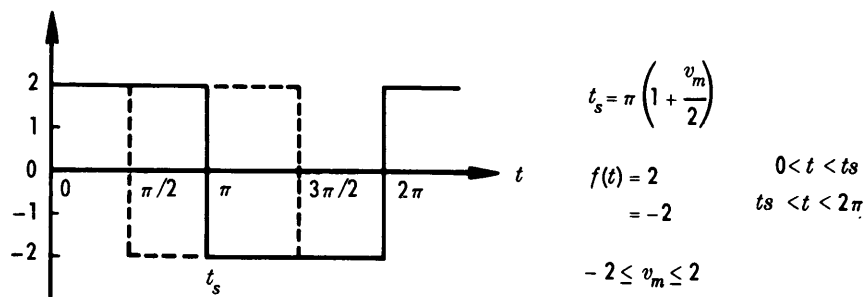
Figure 2 – Typical Data Storage in Differential Pulse Width Modulation
