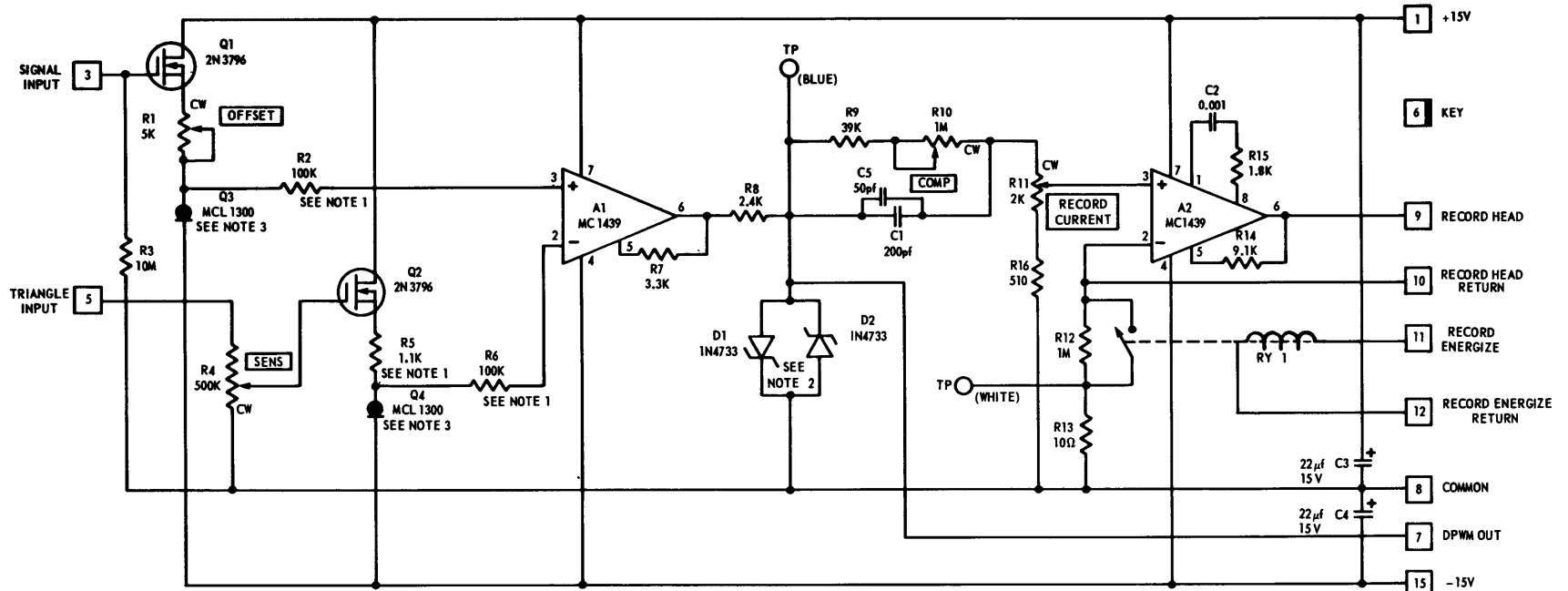
Figure 18 – Model 300 Record Card
