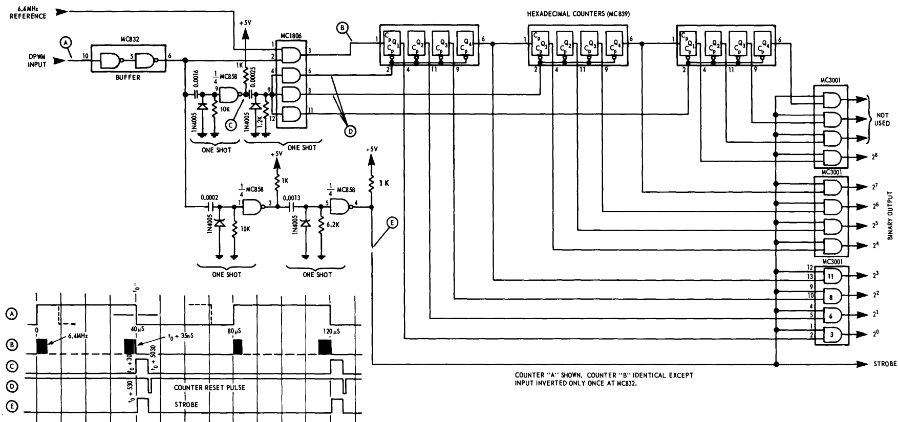
Figure 24 – Digital Interface Electronics Counter
