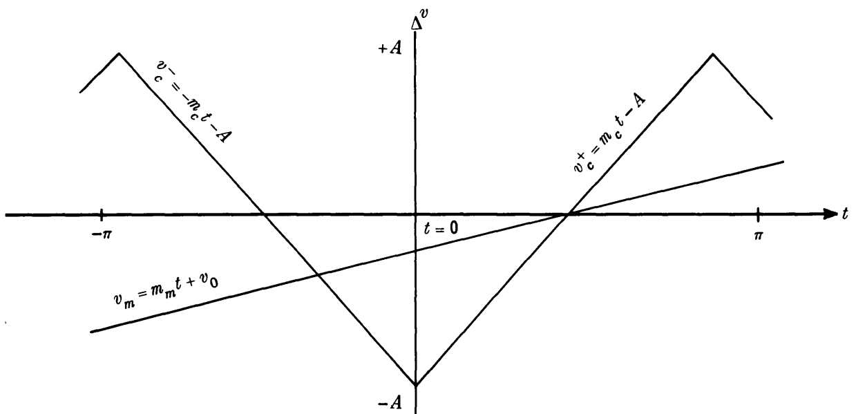
Figure A3 – Intersection of a Ramp with Differential Pulse Width Modulation Triangular Carrier
