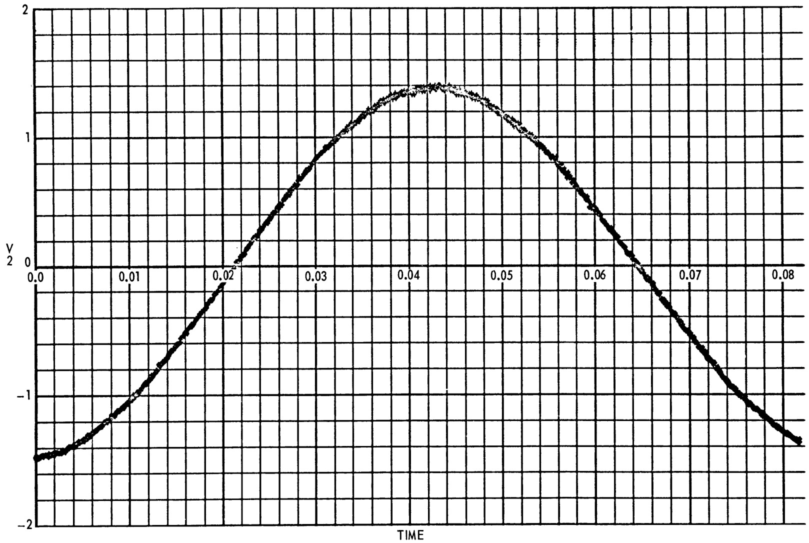
Figure 31 – Partial Computer Plot of File 42 Showing v_2 Points for 10-Hz Sine Wave
