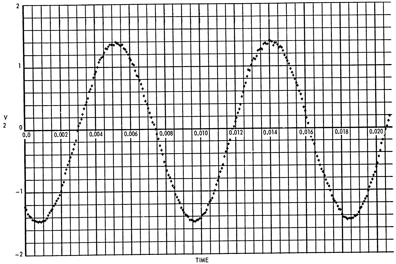
Figure 33 - Partial Computer Plot of File 43 Showing v_2 Points for 100-Hz Sine Wave
