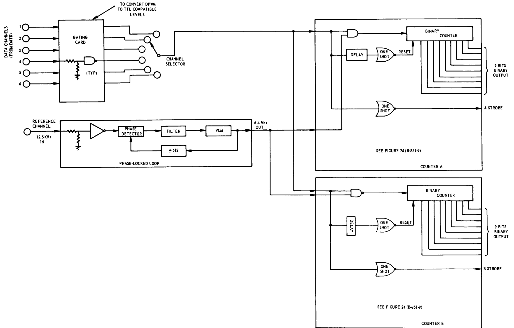
Figure 22 – Digital Interface Electronics General Arrangement
