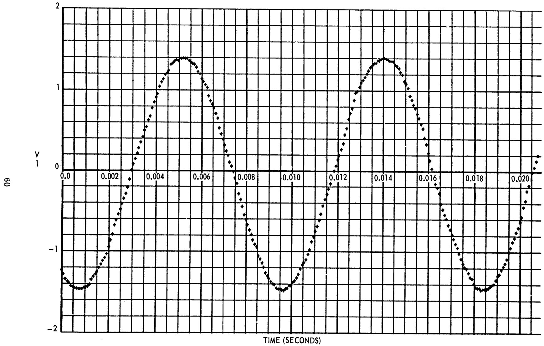
Figure 32 – Partial Computer Plot of File 43 Showing v_1 Points for 100-Hz Sine Wave
