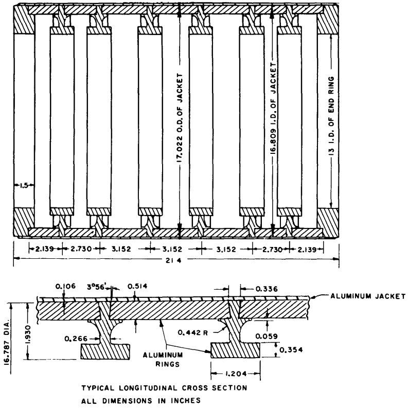
Figure 1a - Model DSRV-1A
