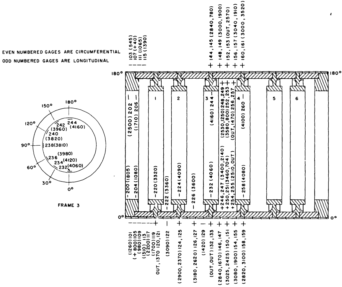
Figure 3a - Model DSRV-1A
