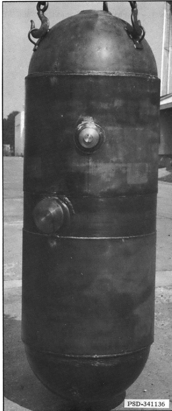
Figure 2 - Model DSRV-1F after Fabrication
