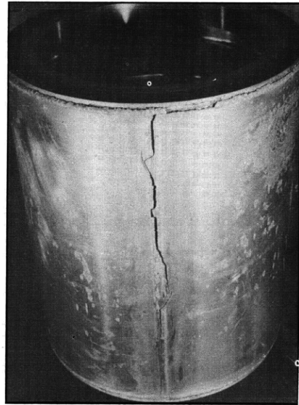
Figure 4 - Models DSRV-1A and DSRV-1F after Cyclic Testing
