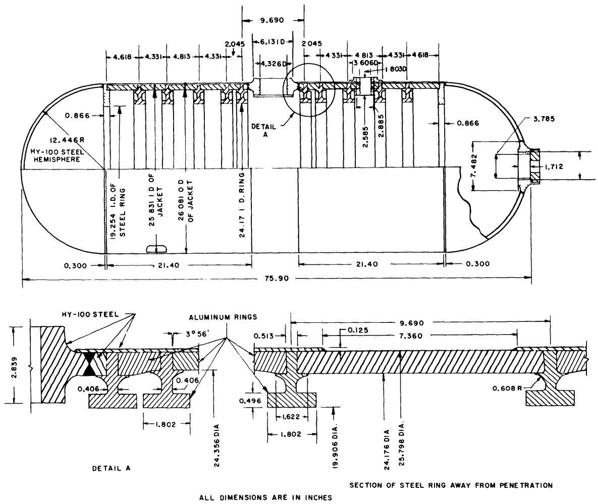
Figure 1b - Model DSRV-1F
