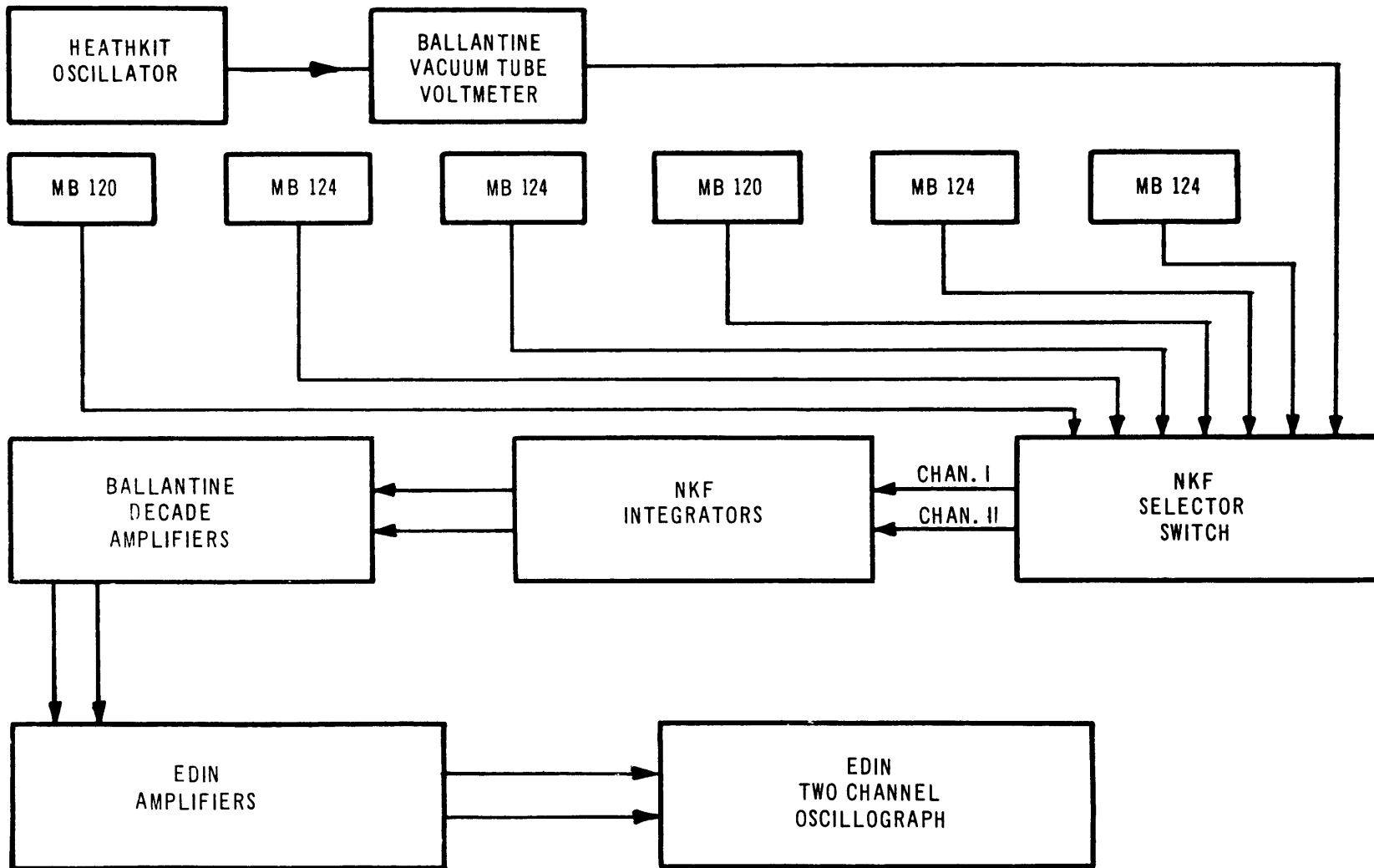
Figure 4 - Electronic Instrumentation for Linear Vibration Measurements
