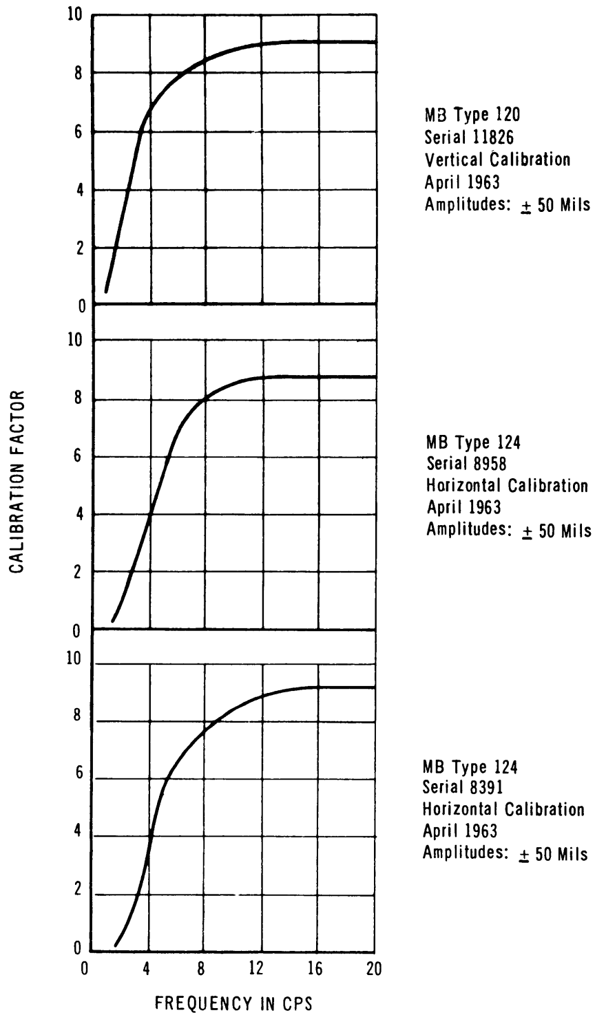
Figure 9 - Calibration Curves - Thrust Bearing Foundation
