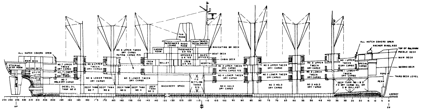
Figure 1 - General Arrangement Inboard Profile Ship "S6-4"
