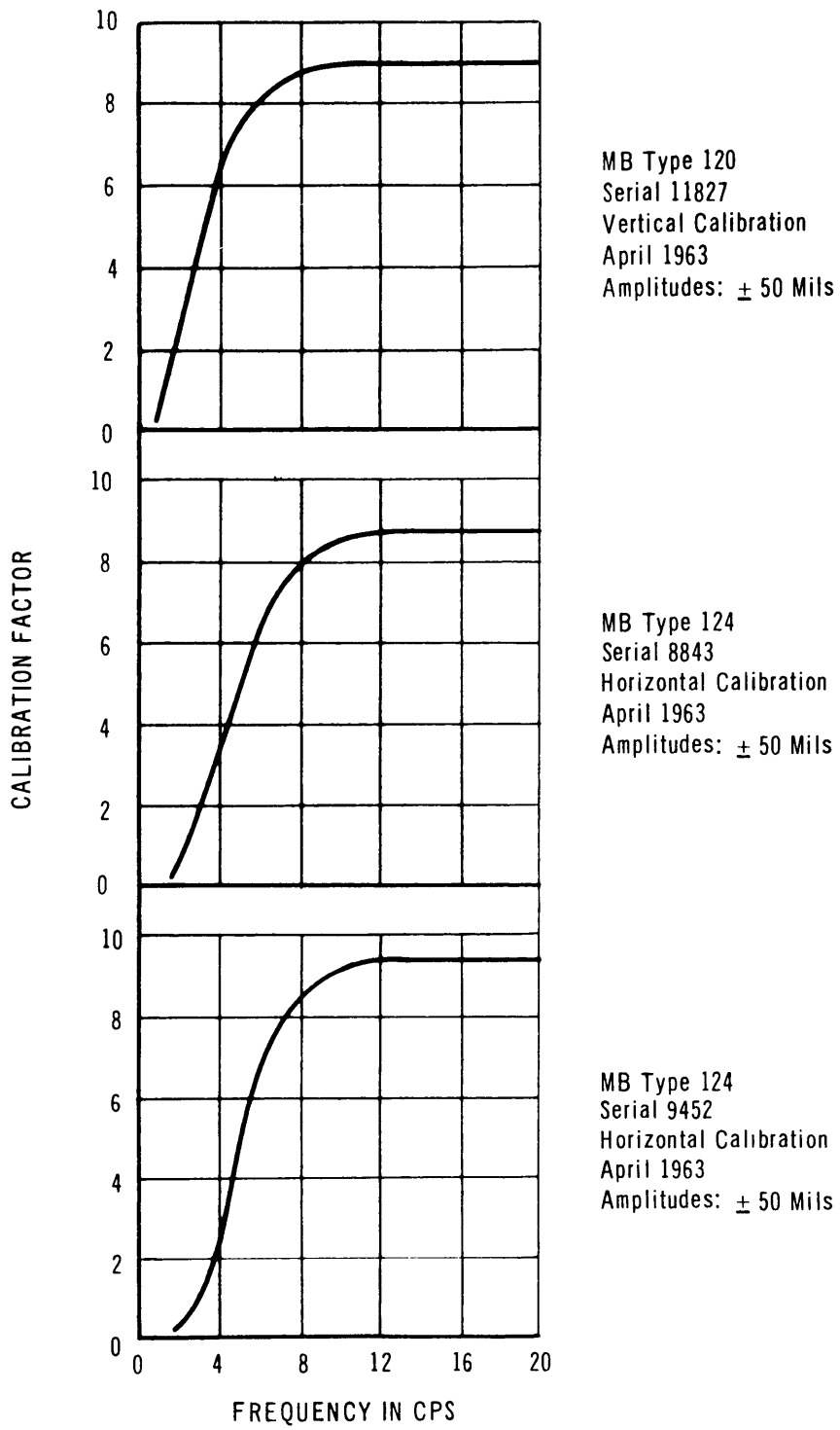
Figure 8 - Calibration Curves - Stern
