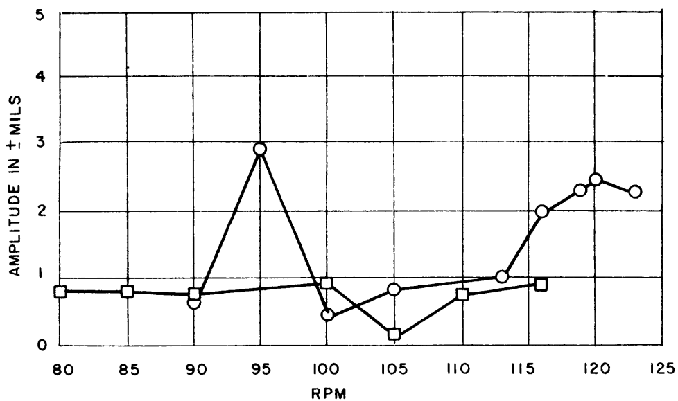
Figure 11 - Athwartship Vibration at Stern - Deep Water - Aft Peak Tank Full
