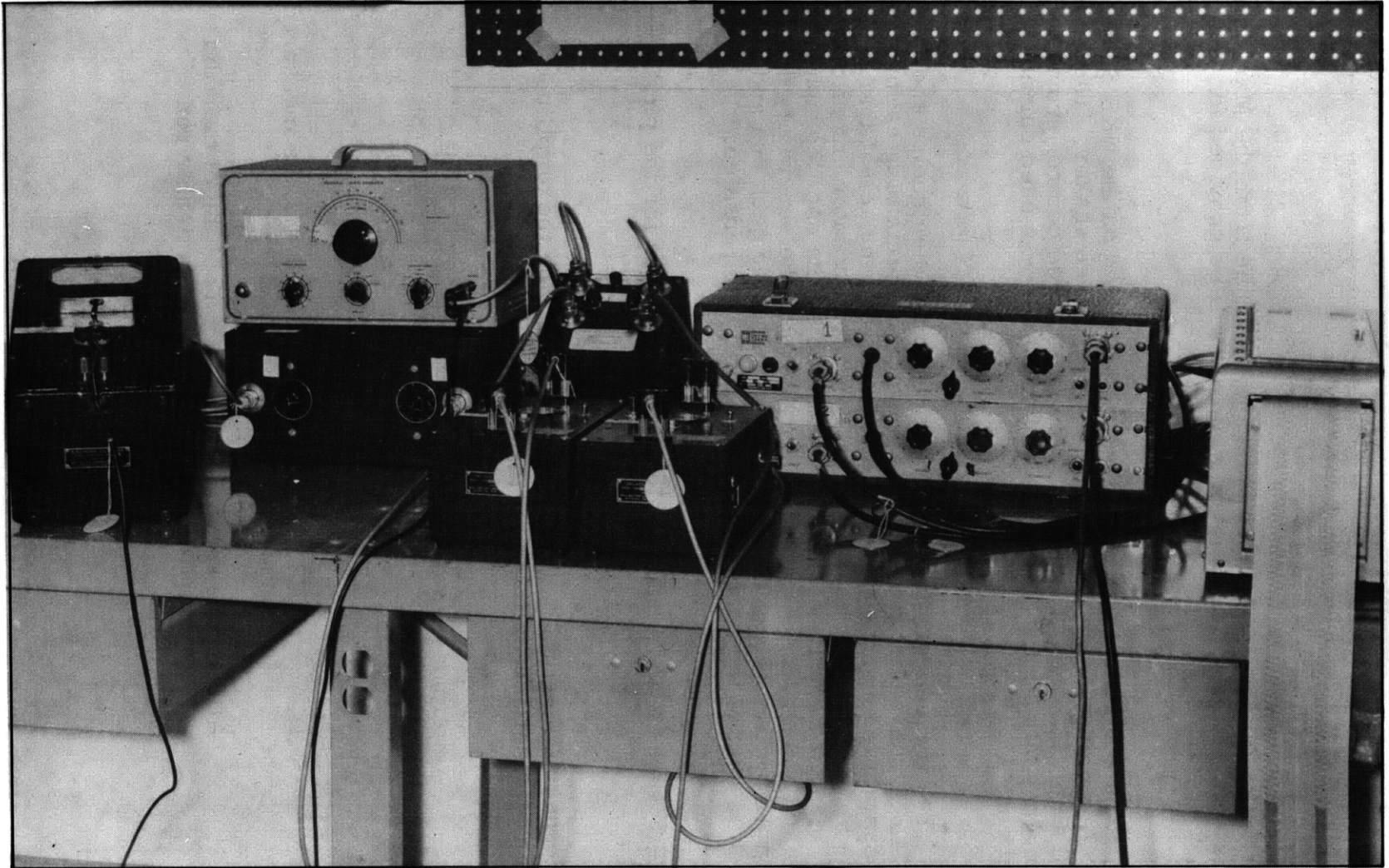
Figure 7 - Instrumentation Arrangement
