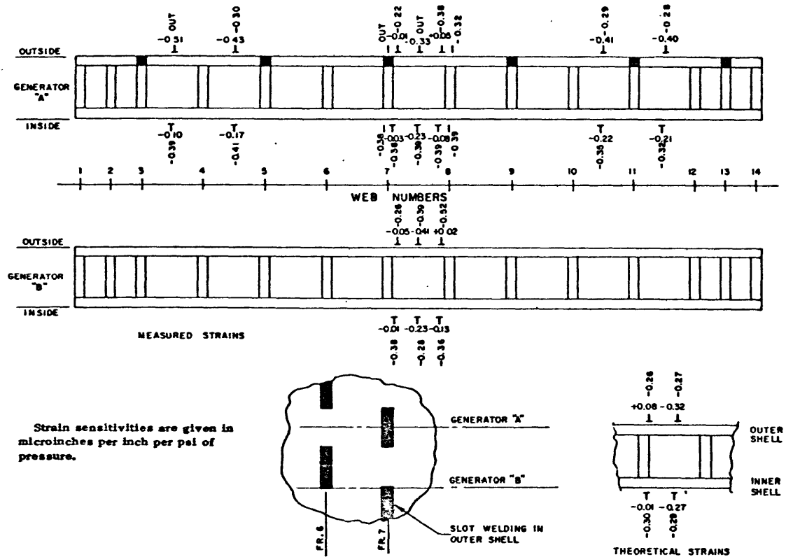
Figure 10 - Theoretical and Measured Strain Sensitivities for Model OV-1
