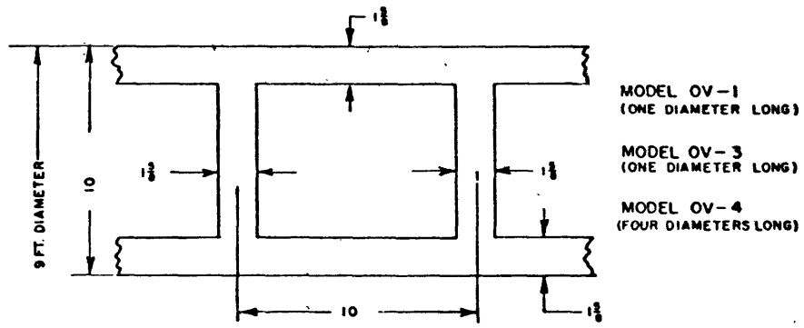
Figure 2a. W/D = 0.631
