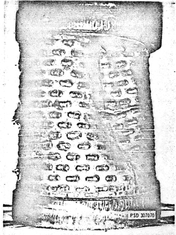
Figure 13 - View of Overall Failure of Model OV-2
