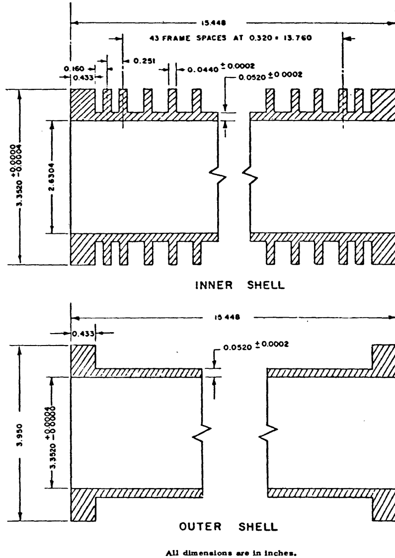
Figure 9 - Details of Model OV-5
