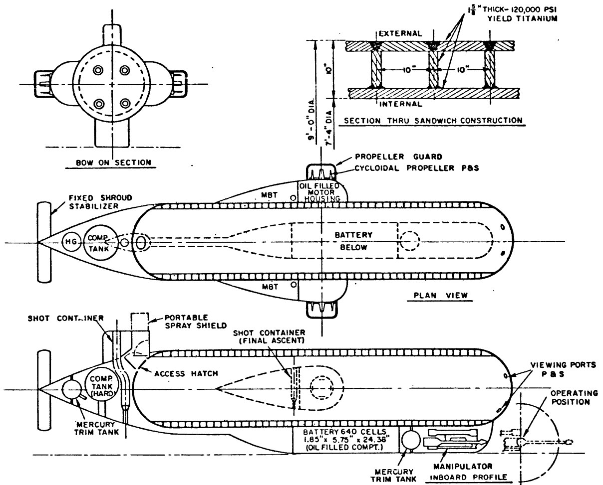
Figure 1 - Inboard Profile of Proposed Oceanographic Vehicle
