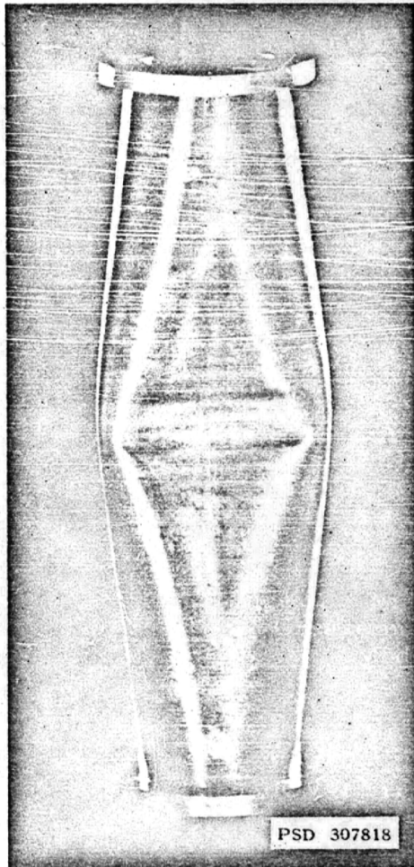
Figure 17 - Model OV-4 after Collapse
