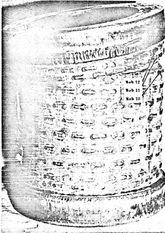
Figure 12 - View of Axisymmetric Crease in Outer Shell of Model OV-1
