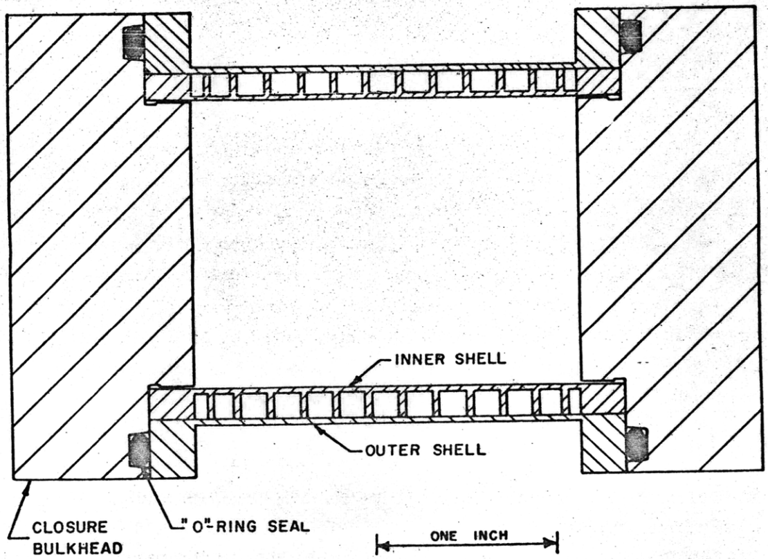
Figure 6 - Assembly Drawing of Model OV-3
