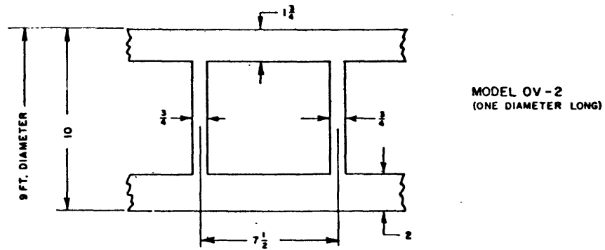
Figure 2b. W/D = 0.633
