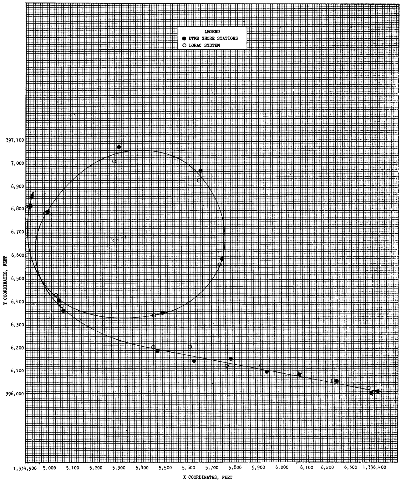
Figure 1 - Turning Circle Using Right Rudder
