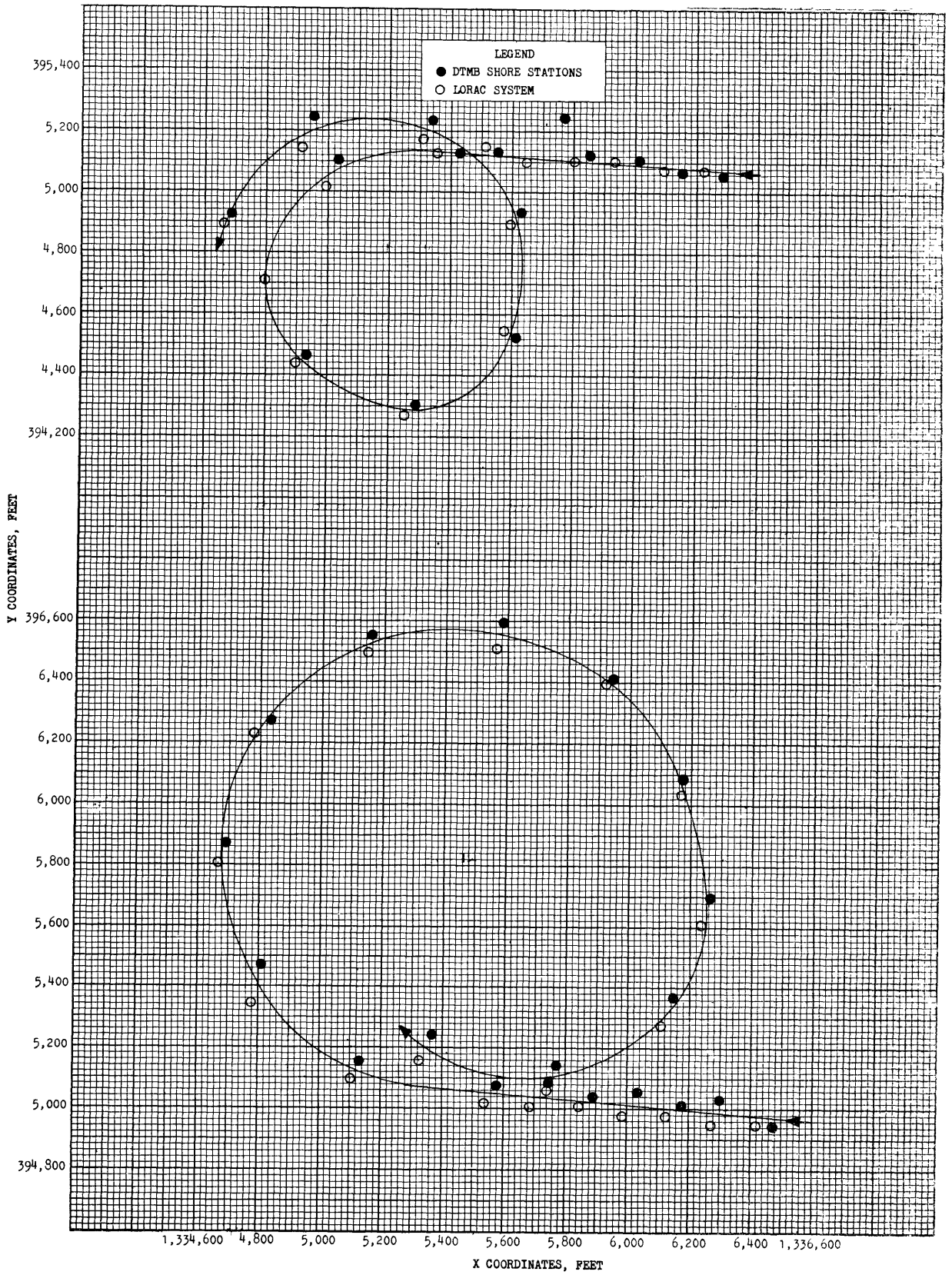
Figure 3 - Turning Circles Using Right and Left Rudder
