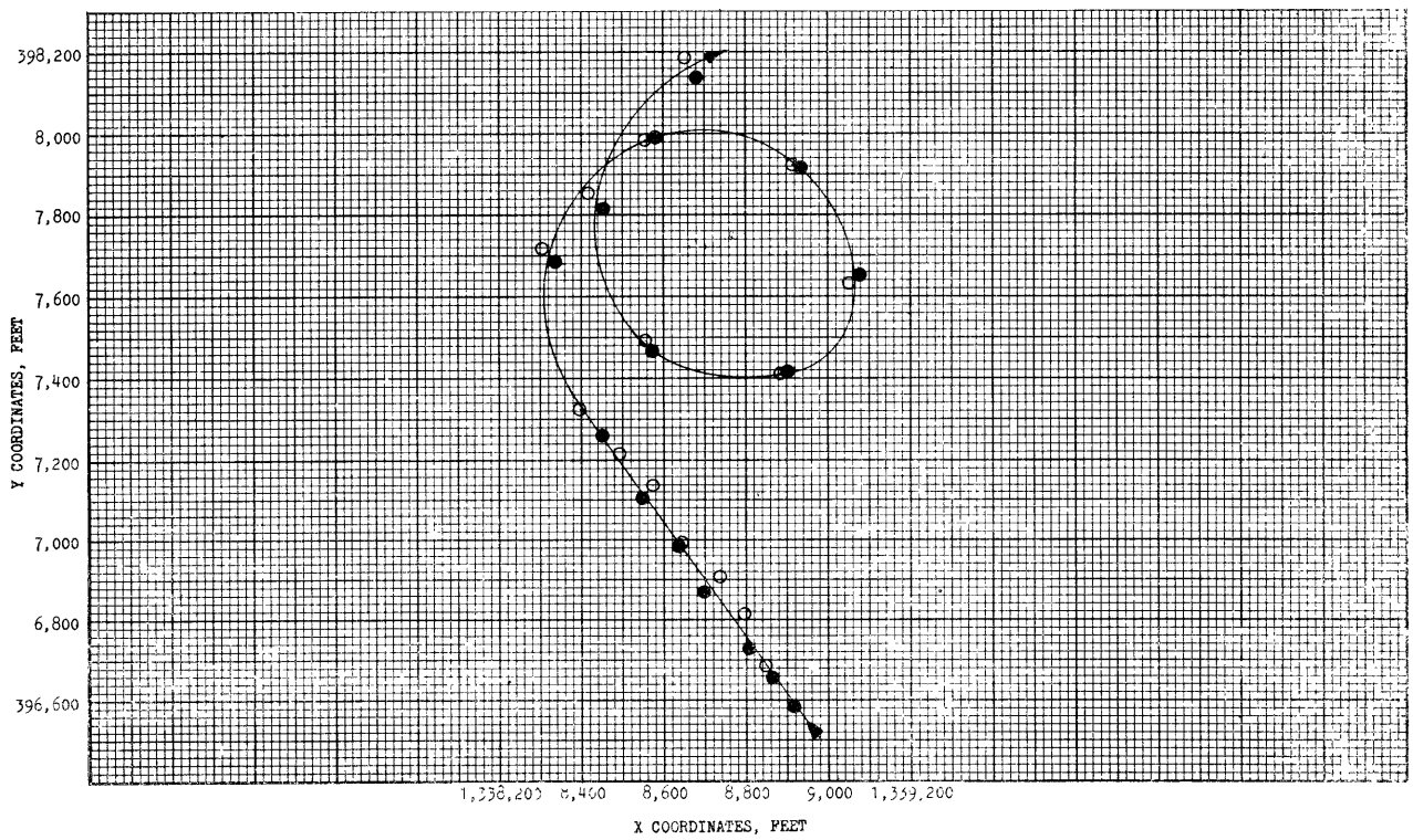
Figure 6 - Turning Circles Using Right Rudder
