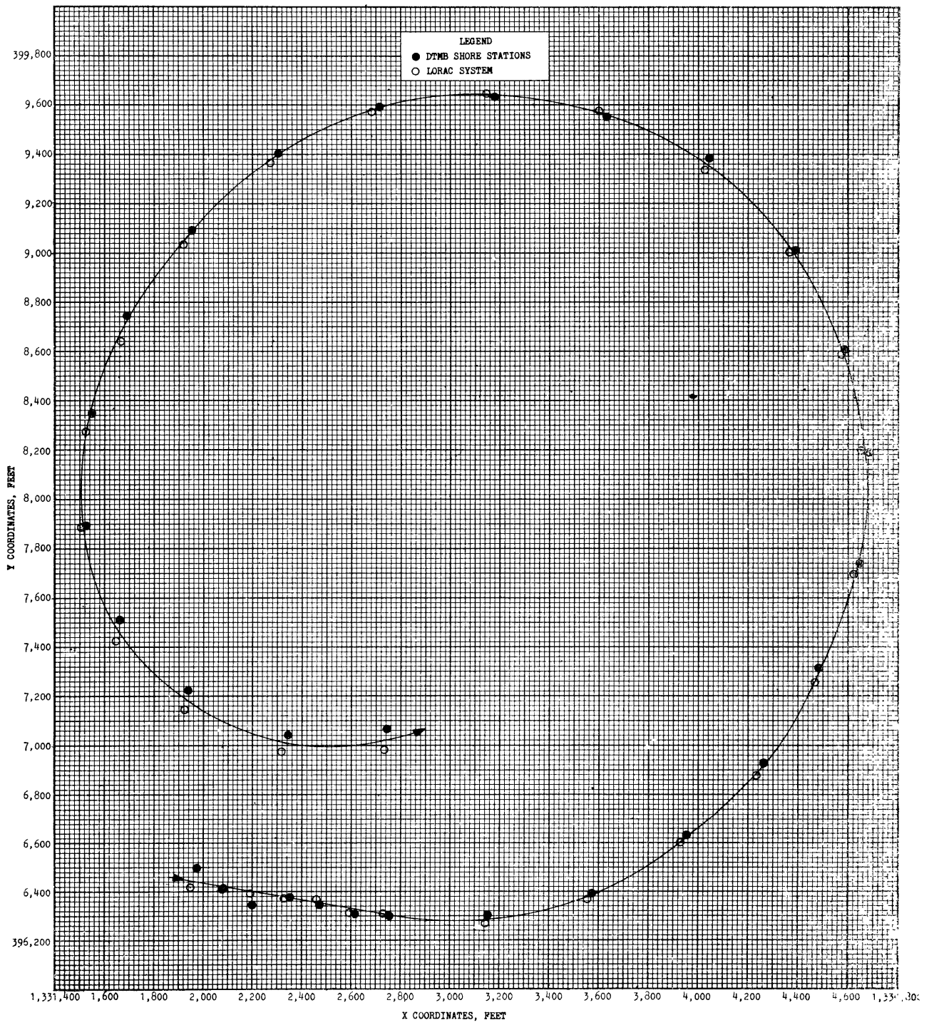
Figure 2 - Turning Circle Using Left Rudder
