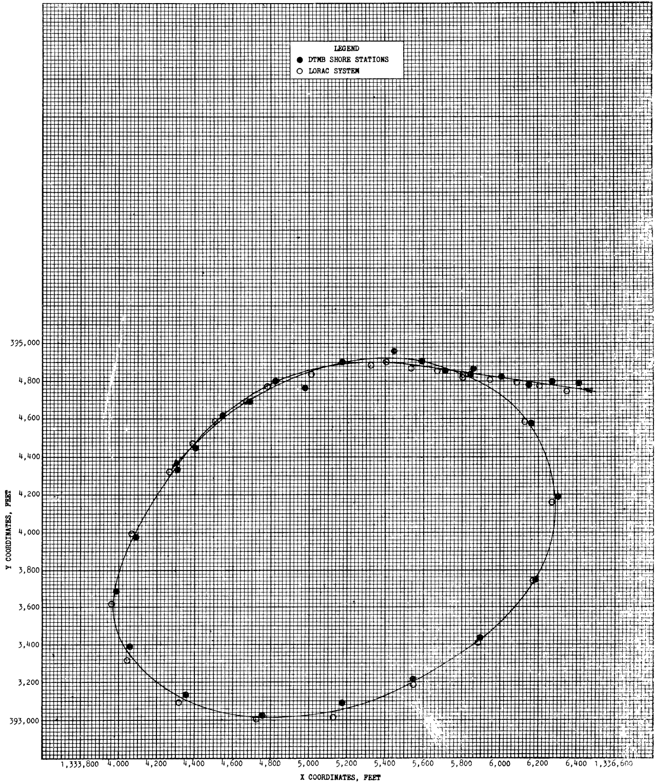
Figure 5 - Turning Circle Using Left Rudder
