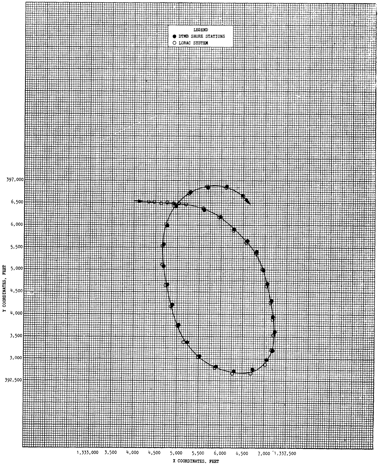
Figure 4 - Turning Circle Using Right Rudder
