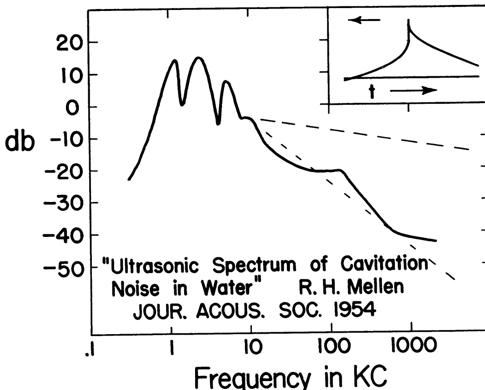
Figure 7. A measured spectrum of cavitation noise. The solid curve represents the spectrum of the steady noise observed at a distance of 1 meter from a metal rod, 2 inches long and 1/16 inch in diameter, rotated at 4300 rpm about a transverse axis through its center. The reference level for the decibel scale corresponds to sound pressure of 1 dyne/cm 2 in a 1 cy/sec band of frequency. The cavities observed were about 1 mm in diameter. The pressure was approximately 1 atmos.
