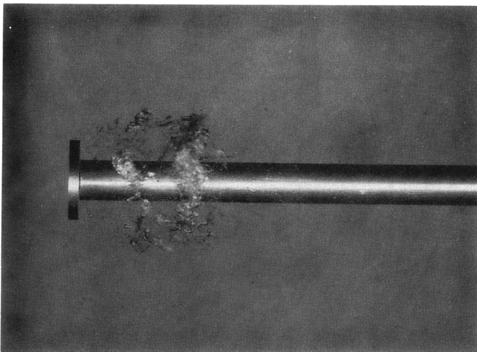
Figure 12. Transient cavities in the vortex sheet behind a sharp-edged disk. The water flows from left to right. (From Ref. 31.)
