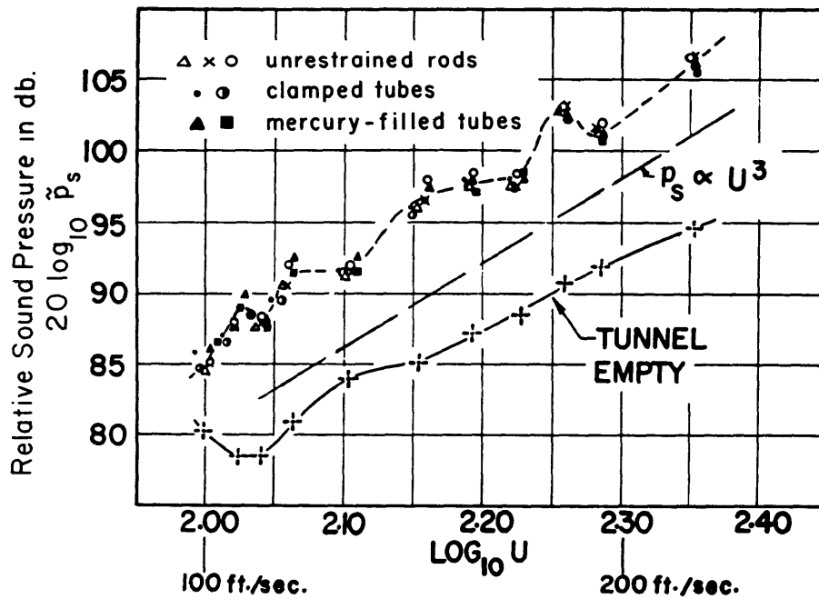
Figure 21. The sound pressure radiated by a cylinder shedding vortices in air, as a function of speed. (From Etkin et al [53].)
