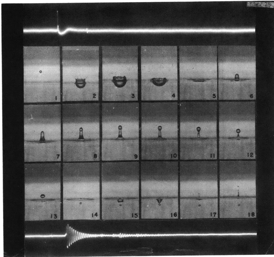
Figure 18. Oscillogram of sound pressure and photographs of splash produced by impinging water droplet. The interval between frames is 13 millisecc. The impact sound occurs between Frames 1 and 2; bubble sound begins between Frames 13 and 14. The bubble can be seen in Frames 14 to 18. The mass of the droplet is 56 mg; its velocity at impact, 350 cm/sec.
