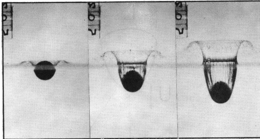
Figure 13. High-speed motion pictures of a 1-inch steel sphere entering the water at a velocity of 35 ft/sec. The time interval between frames is 1.6 millisecc. (From Ref. 34.)
