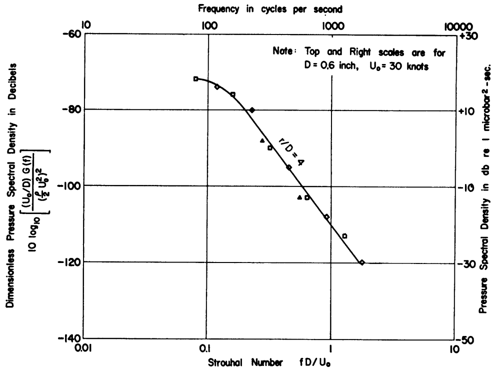
Figure 20. The spectral density of the fluctuating pressure in the near-field of a free jet of water. (From Jorgensen [21].)
