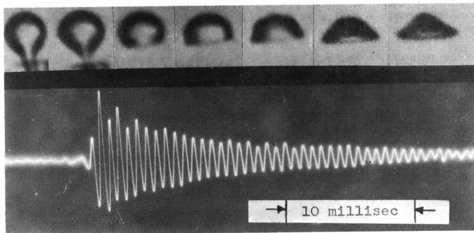
Figure 1. Oscillogram of the sound pulse from an air bubble formed at a nozzle, with synchronized photographs of the bubble. The time each photograph was taken corresponds to the point below the bubble on the oscillogram.
