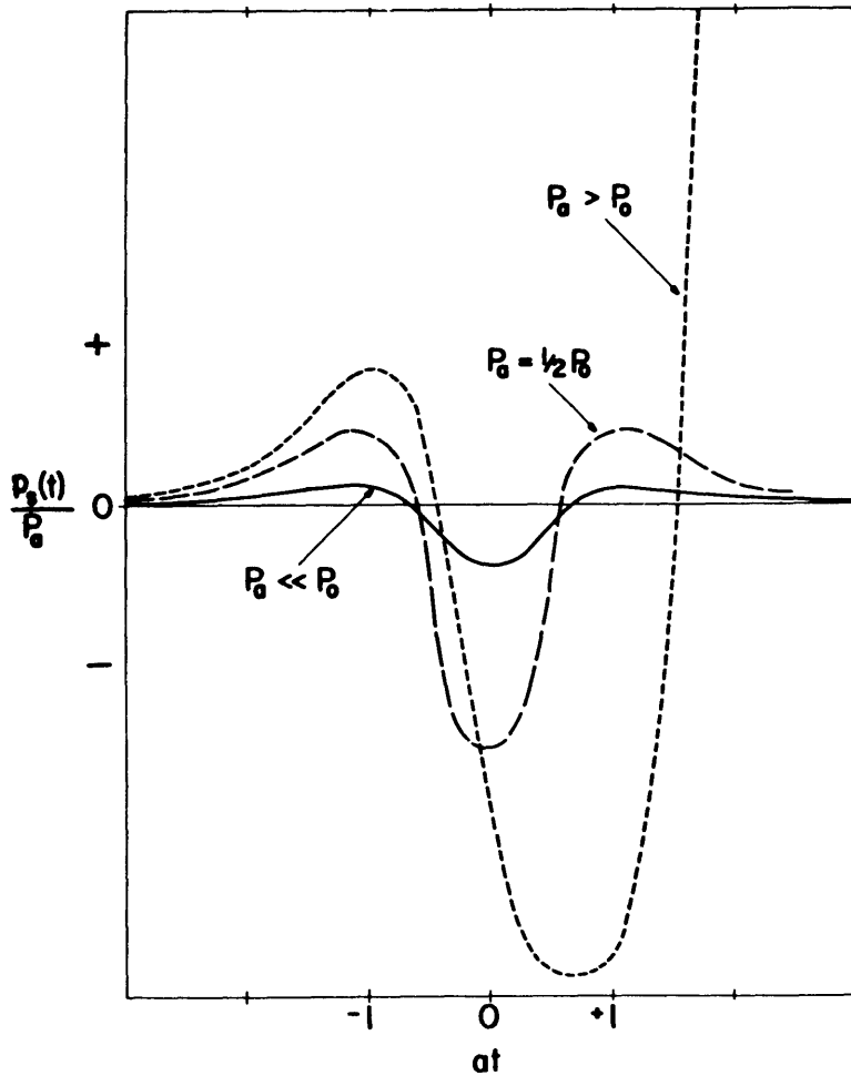
Figure 2... The sound pressure radiated by a bubble in response to an environmental pressure given by p_e(t) = P_0 - P_a \operatorname{sech}^2 at , which is similar to the pressure on a bubble moving around the surface of a cylinder in a flow. The curves indicate the development of non-linearity for successively smaller values of P_0 relative to P_a . The solid curve represents the linear range.
