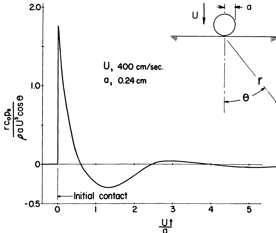
Figure 17. Pressure pulse produced by the impact of a water droplet.
