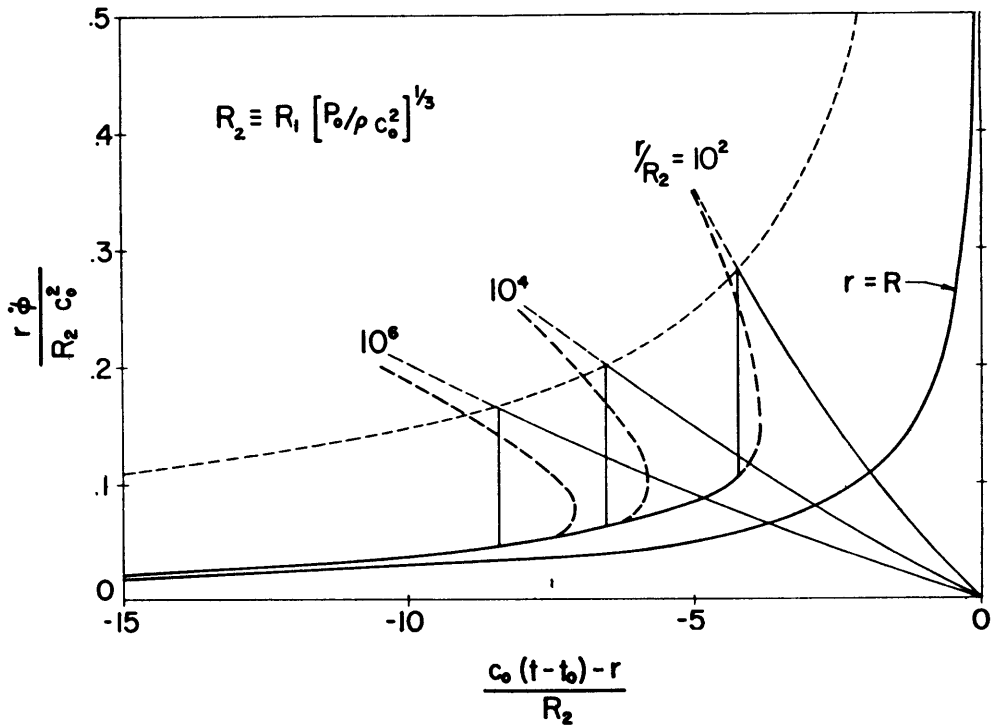
Figure 10. Pressures and shocks radiated by a vapor cavity collapsing in a compressible liquid. (Values according to Mellen [30].)
