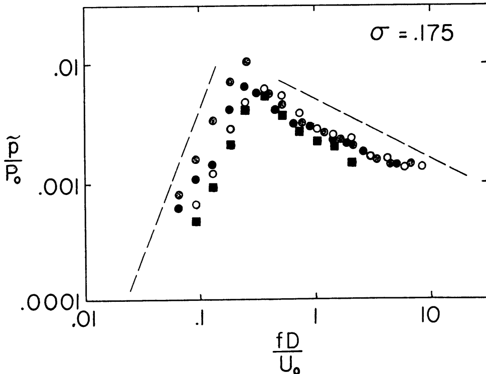
Figure 8. The measured spectrum of noise produced by a cavitating jet. The symbol \tilde{p} represents the rms pressure in a half-octave band of frequency, at a point four diameters off the axis and four diameters downstream from the orifice. The different spots represent different combinations of jet diameter, D ( 3/8 , 3/4 , and 1\ 1/2 inch), and ambient pressure, P_0 ( 1/2 , 1, and 2 atmos). U_0 is the efflux velocity; \sigma is the cavitation index, 2P_0/\rho U_0^2 . (From Jorgensen [21])
