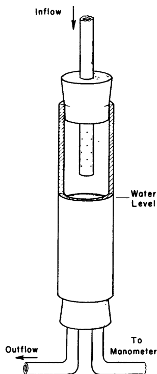
Figure 1 - Basic Form of Meter Chamber
