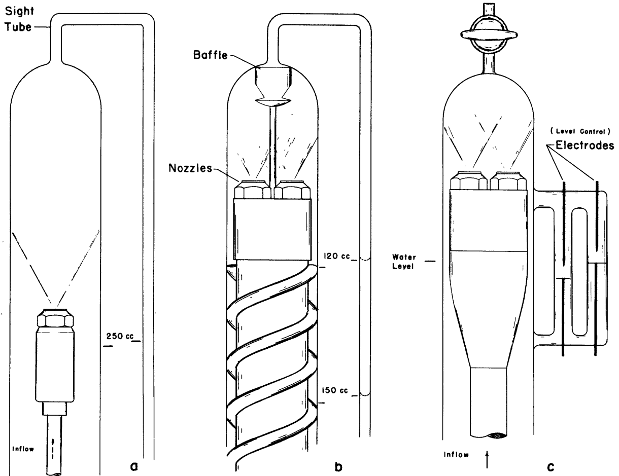
Figure 4 - Details of Three Arrangements of Meter Chamber
