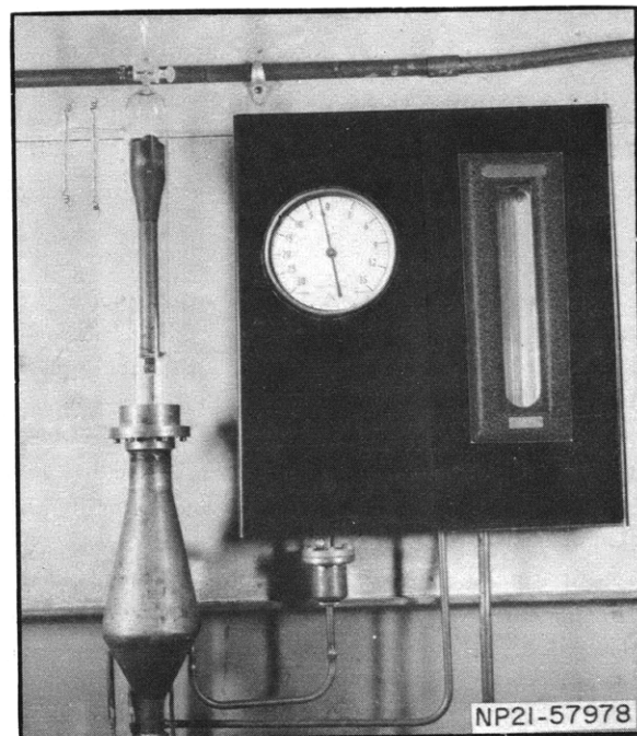
Figure 3 - Meter Chamber, Pressure Gage, and Flowmeter Installed
