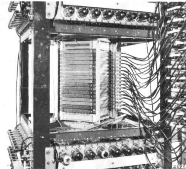
Fig. 3-2. First Bank of Magnetic-Core Storage
