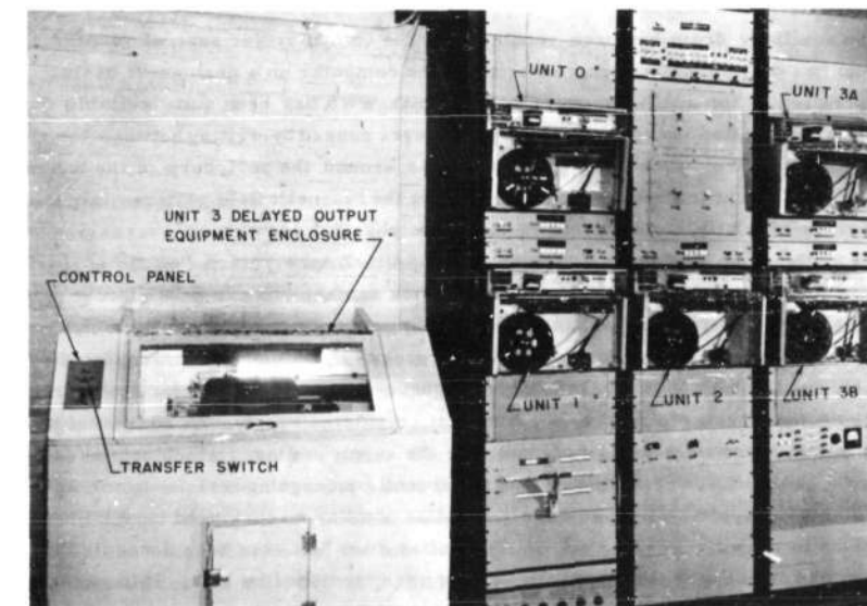
Fig. 3-5. Magnetic-Tape Units and Delayed-Output Equipment
