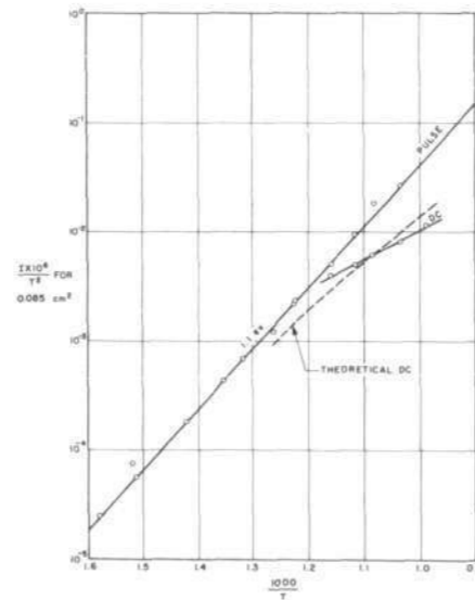
Fig. 4-2. Richardson Plot, RT 414
