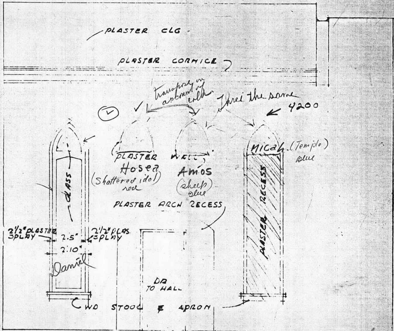
Chapel EAST WALL ELEV. 1/4" = 1'-0"
