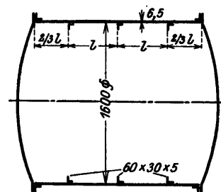
Figure 30 - Experimental Model with Three Frames
