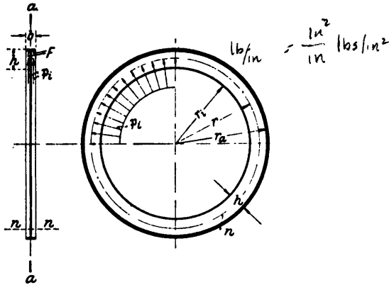
Figure 8 - Circular Ring or Frame under Internal Pressure p_i
