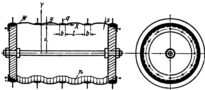
Figure 13 - Tube Free to Expand and Contract Axially and Fitted with Transverse Frames
