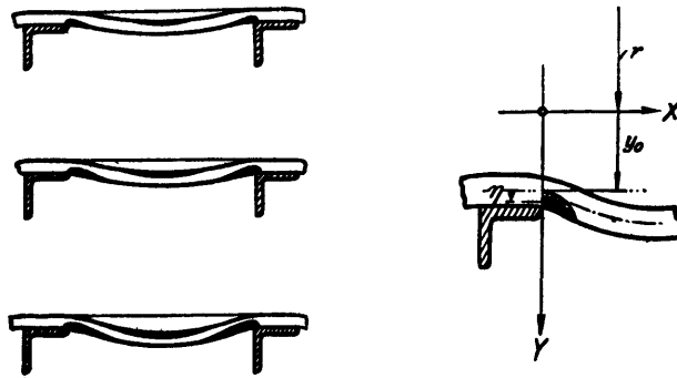
Figure 28 - Schematic View of the Gradual Extension of the Regions Where the Elastic Limit Is Exceeded as the Pressure Increases
