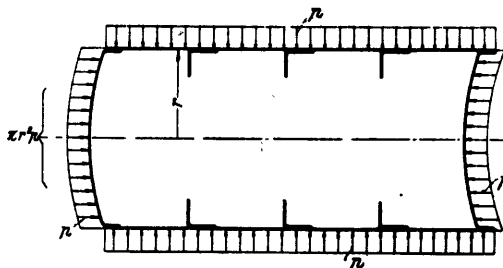
Figure 12 - Submerged Body Fitted with Frames and Ends
