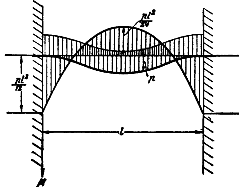
Figure 15 - Straight Rod Clamped at Both Ends (Deflection Curve and Curve of Moments)
