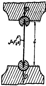
Figure 2 - Diagram of a Rod under Compression with Hinged Bearings
