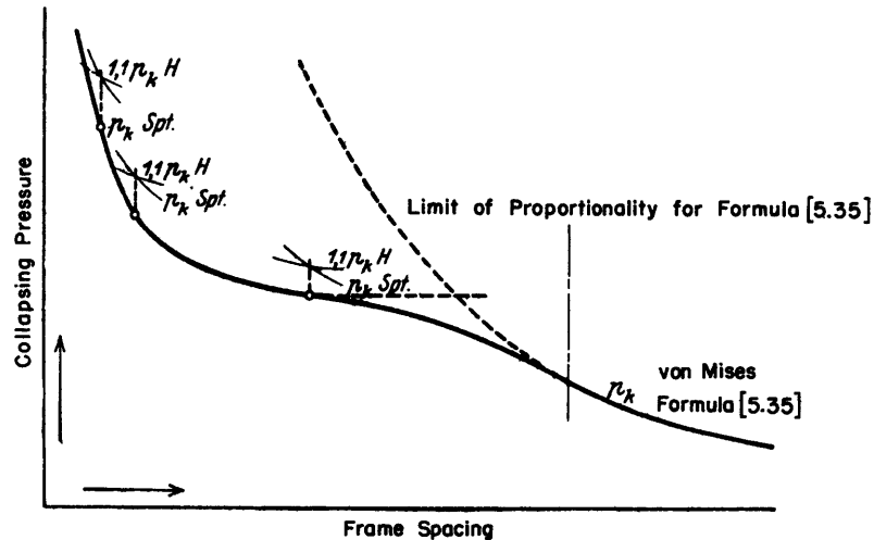
Figure 32 - Collapsing Pressure of a Cylindrical Tube of Constant Shell Thickness and Variable Frame Spacing under a Uniform External Pressure
