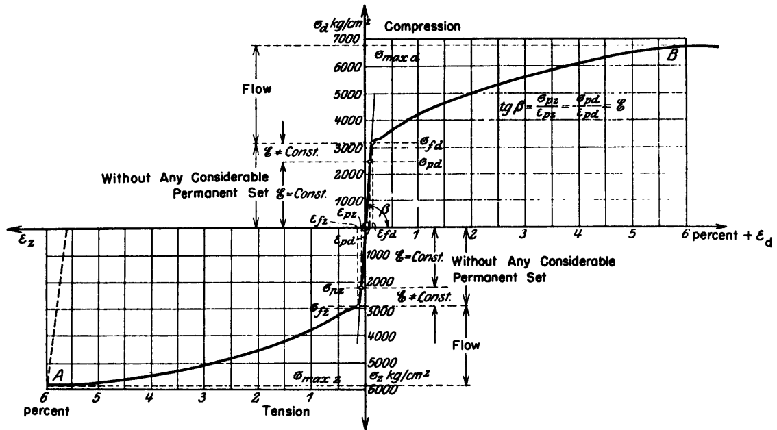
Figure 4 - Stress-Strain Diagram
