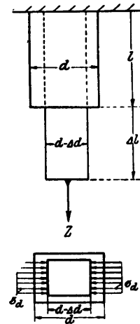
Figure 20 - Diagram of a Rod in Tension and Subject to an Additional Hydraulic Load \sigma_d
