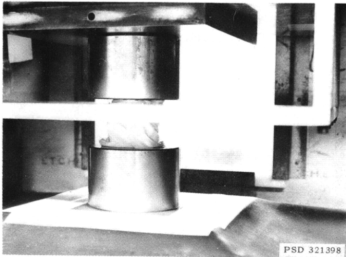
Figure A22a – Specimen Wrapped in Wet Cotton prior to Test
