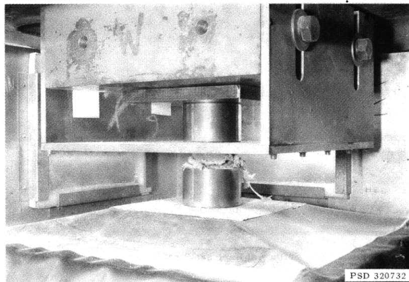
Figure A18b – Interior of Spall Shield after Test
