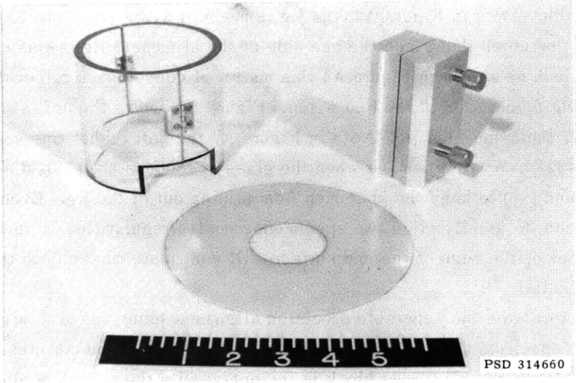
Figure A3 – Fragment Shields and Precision Alignment Block for Centering Bearing Blocks and Specimen Alignment Jig under Compression Subpress
