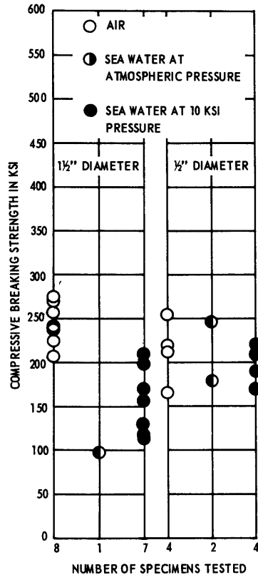
Figure 4 – Effect of Specimen Size on the Compressive Breaking Strength of 7265 (50-KSI) Strengthened Glass
