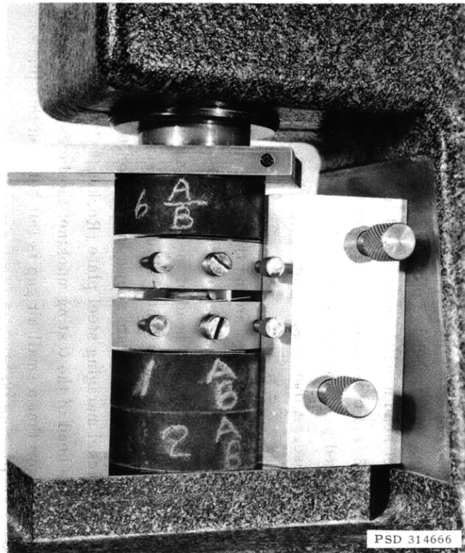
Figure A8 – Separable Precision Alignment Blocks and Specimen Alignment Jig under Center of Compression Subpress
