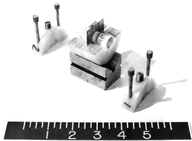
Figure A5 – Specimen Alignment Jig with Specimens and Center Gasket in Place
