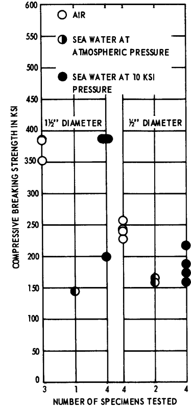
Figure 6 – Effect of Specimen Size on the Compressive Breaking Strength of 9611 (100-KSI) Strengthened Pyroceram
