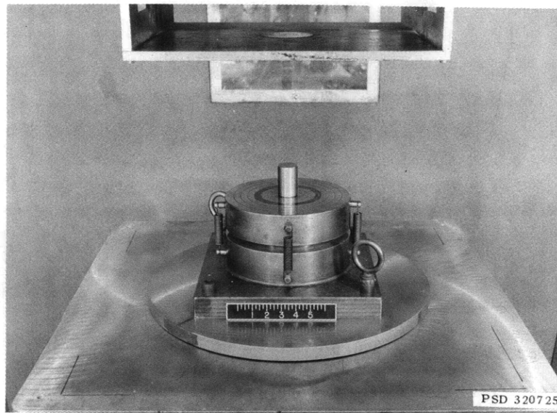
Figure A13 – Self-Aligning Swivel Loading Head
