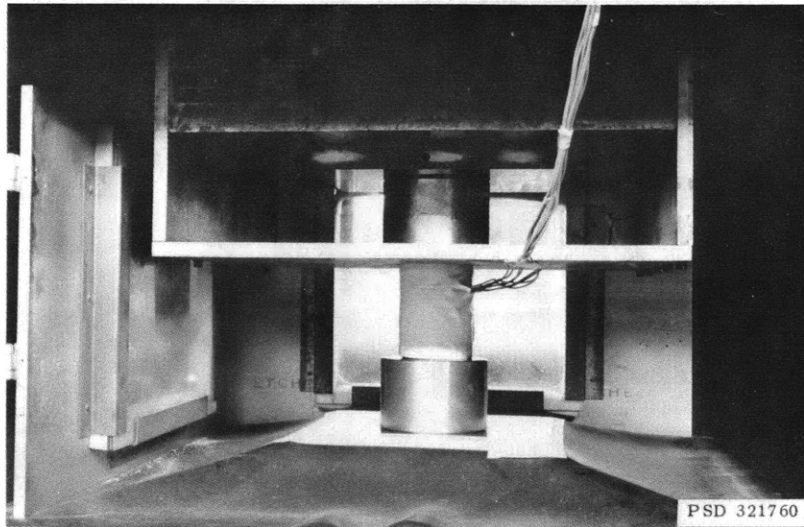
Figure A26 – Strain-Gaged Specimen Wrapped in Vinyl Tape to Contain Fragments
