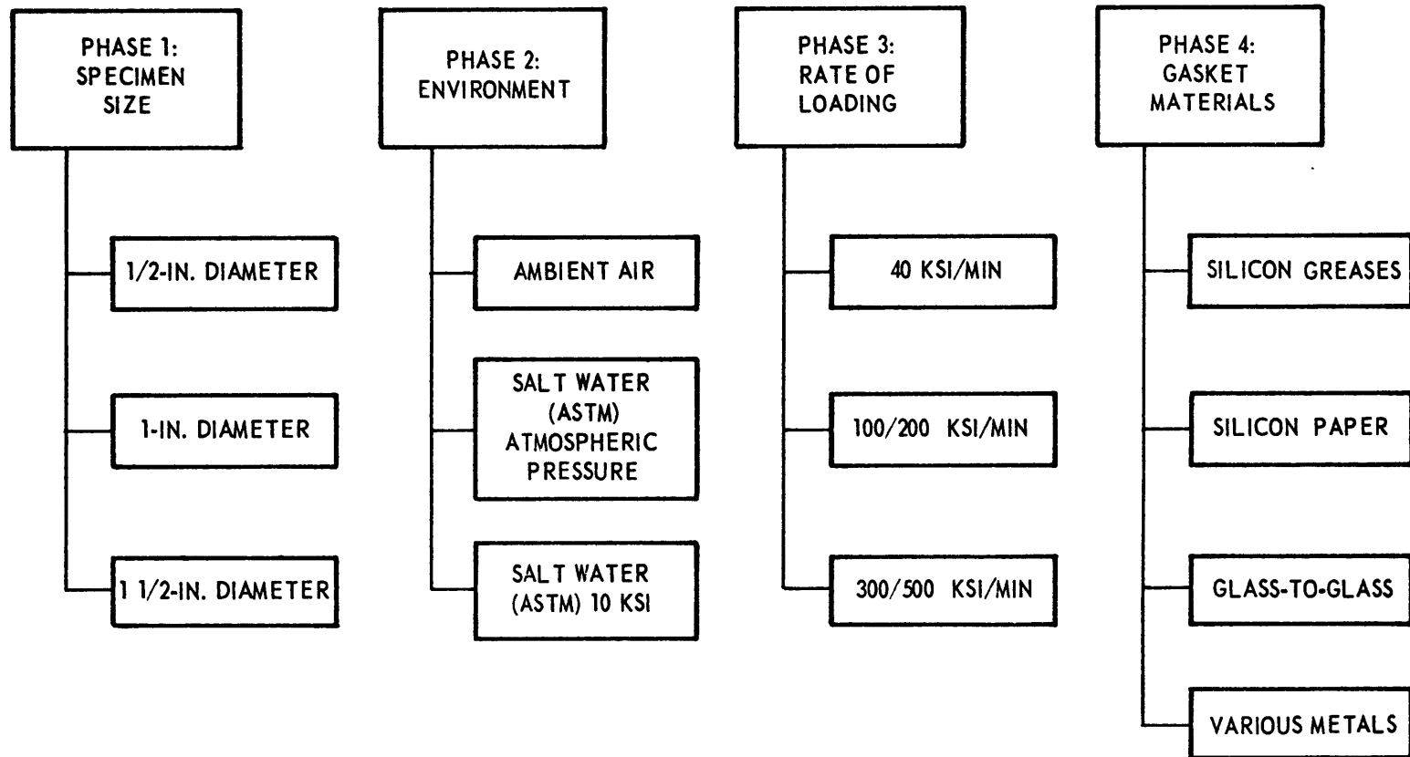
Figure 1 – Investigative Steps in a Program to Establish the Compressive Strength of Glasses
