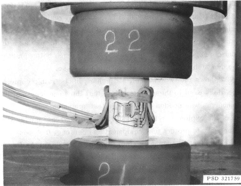
Figure A23 – Strain-Gaged Specimens and Sintered Tungsten Carbide Bearing Blocks
