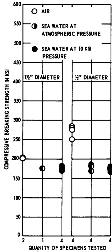
Figure 7 – Effect of Specimen Size on the Compressive Breaking Strength of 9606 Annealed Pyroceram
