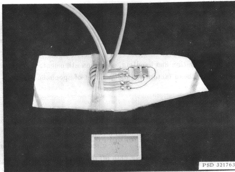
Figure A24 – Temperature-Compensating Dummy Gage
