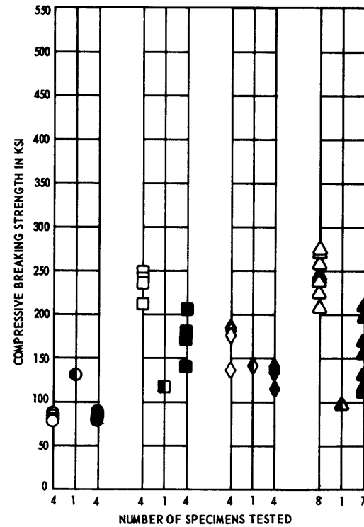
Figure 8 – Effects of Environment on the Compressive Breaking Strength of 1 1/2-Inch-Diameter Glass Specimens
