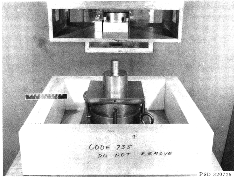
Figure A14 – Adaptor Box Around Swivel Head and Three-Piece Steel Frame Attached to the Top Head of the Testing Machine
