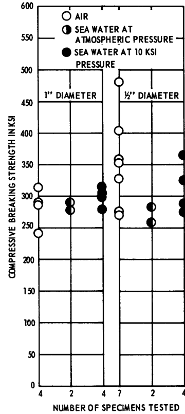
Figure 5 – Effects of Specimen Size on the Compressive Breaking Strength of Annealed AD-99C Alumina
