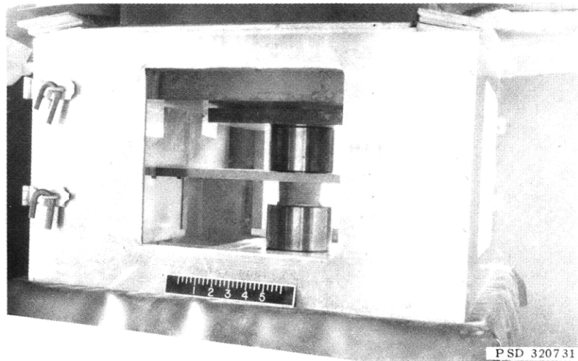
Figure A18a – Test Setup with Spall Shield in Place
