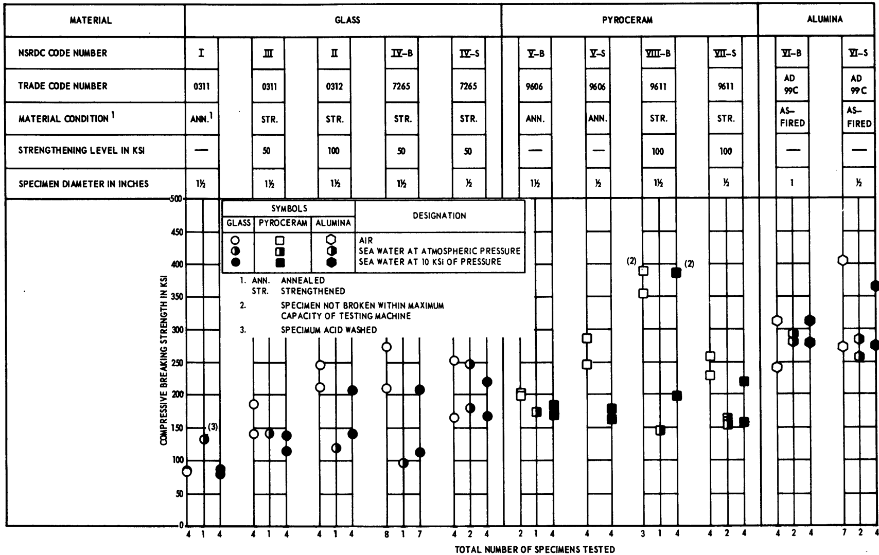
Figure 3 - Effects of Size and Environment on the Uniaxial Compressive Breaking Strength of Glass, Alumina, and Pyroceram
