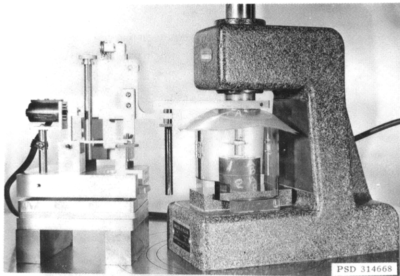
Figure A10 – Complete Test Setup Showing Compression Subpress, Deflectometer, Spall Shield, Hardened Parallel Bearing Blocks, Gasket Material, and Specimens Centered on the Loading Table of the Testing Machine
