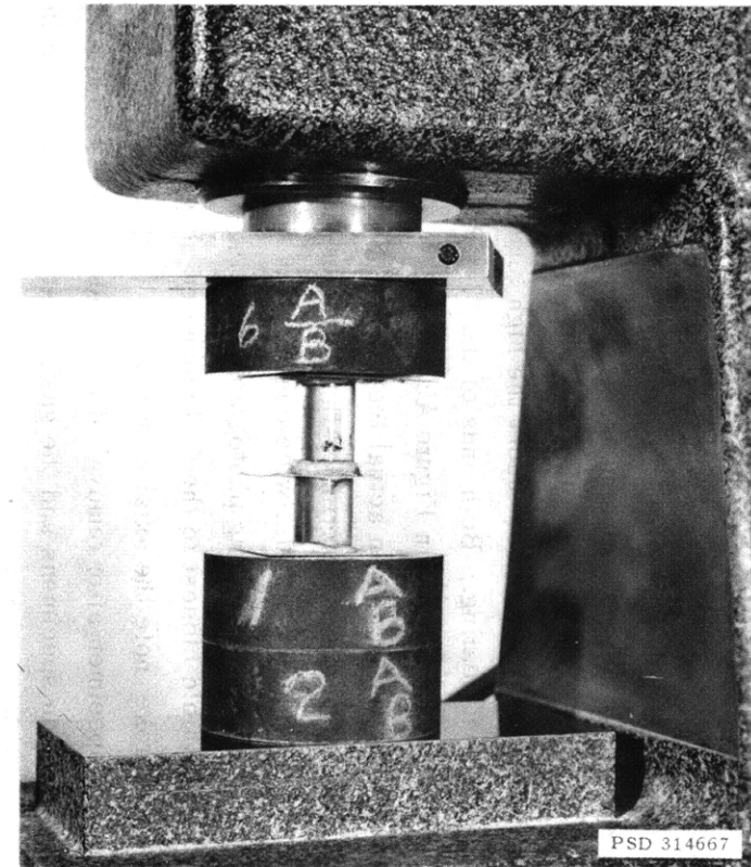
Figure A9 – Test Setup after Removal of Precision Alignment Blocks and Specimen Alignment Jig
