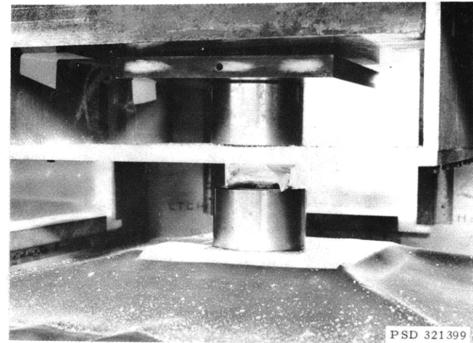
Figure A22b – Specimen Wrapped in Wet Cotton after Completion of Test
