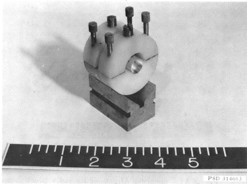
Figure A6 – Assembled Specimen Alignment Jig
