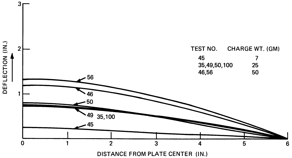
Figure 12c - 1/8-Inch Medium Steel, Air Backed, SOD = 35 Inches
