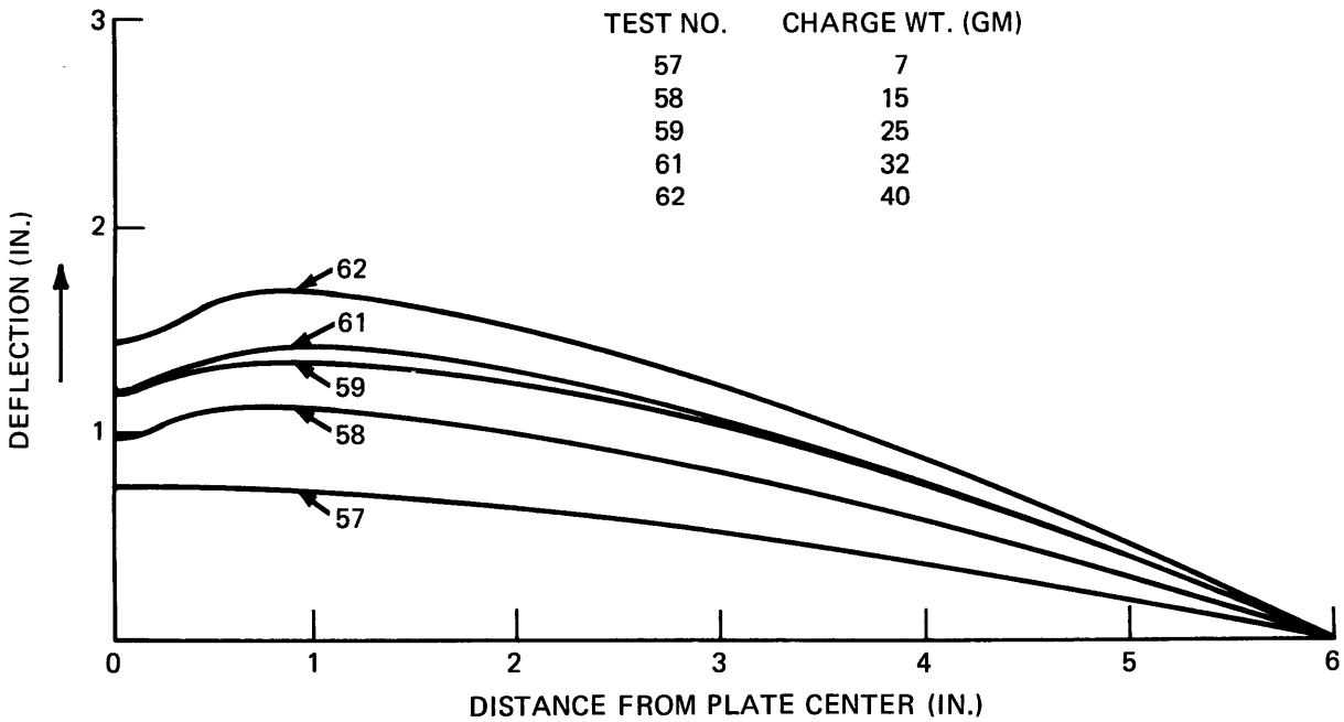
Figure 12f - 1/16-Inch Aluminum, Water Backed, SOD = 35 Inches
