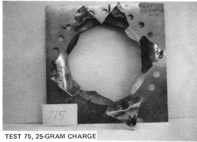
Figure 13d – Center Rupture of a 1/16-Inch Aluminum, Air-Backed Plate (Charge only 6 in. from the plate)
