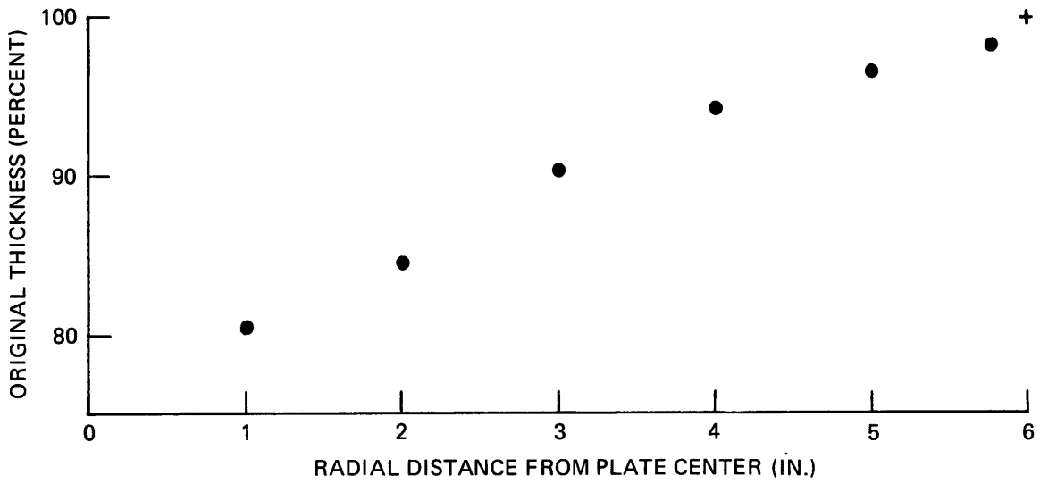
Figure 14a – Final Thickness across a 1/8-Inch Aluminum Plate
