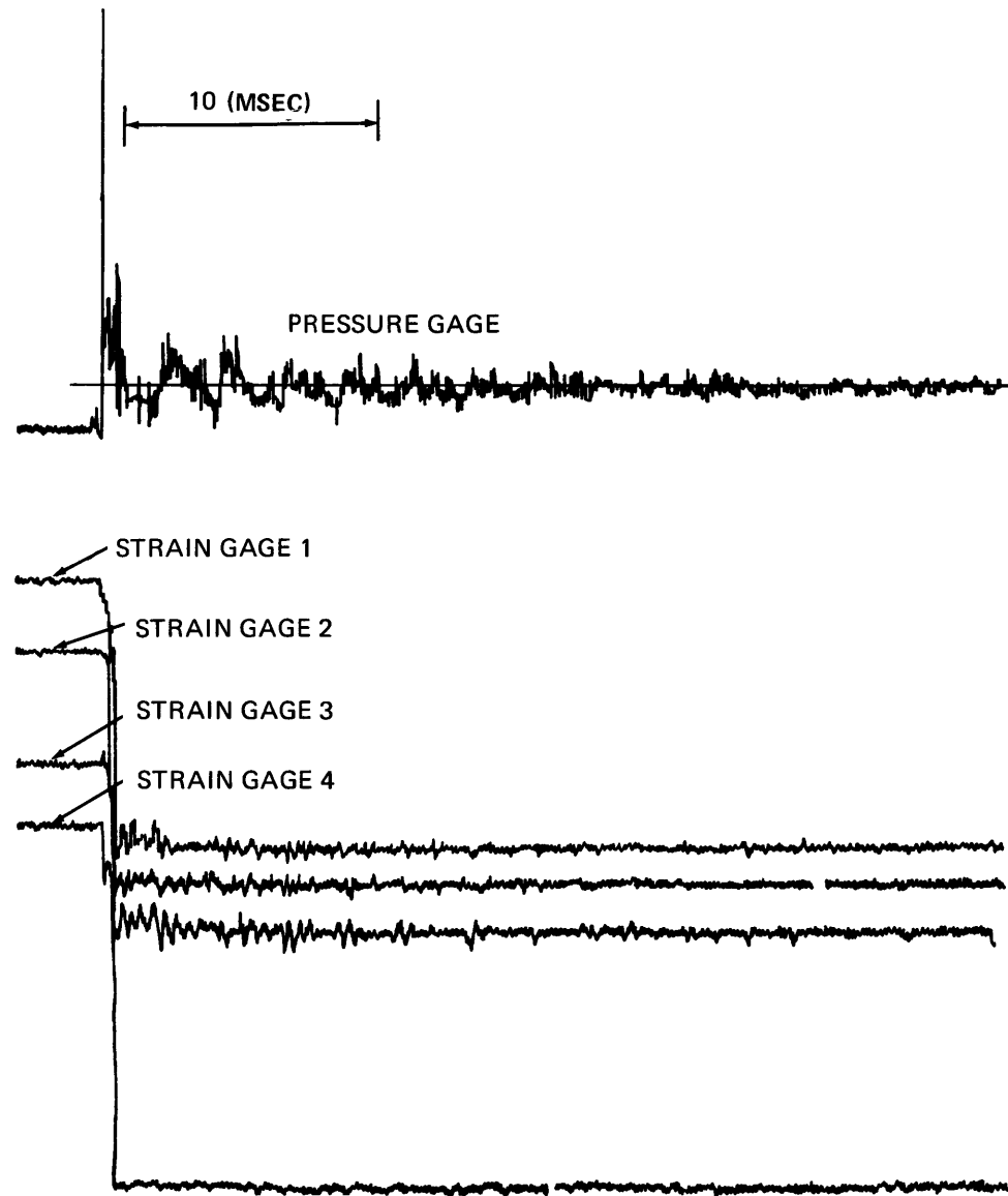
Figure 15f – Slow-Speed Playback of Test 107
