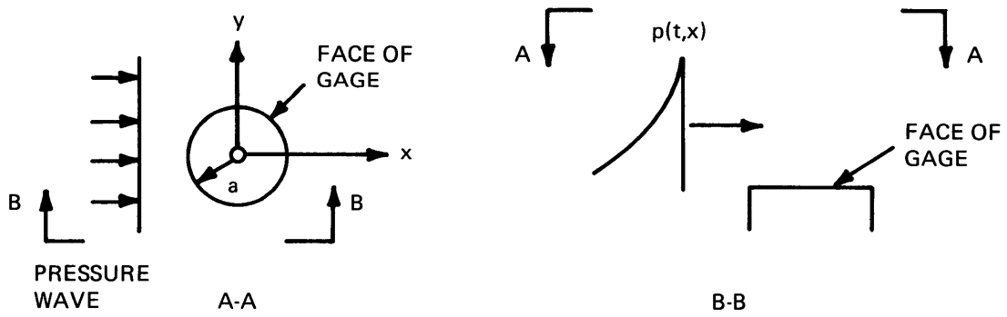
Figure A.4 – Passage of Wave over Gage
