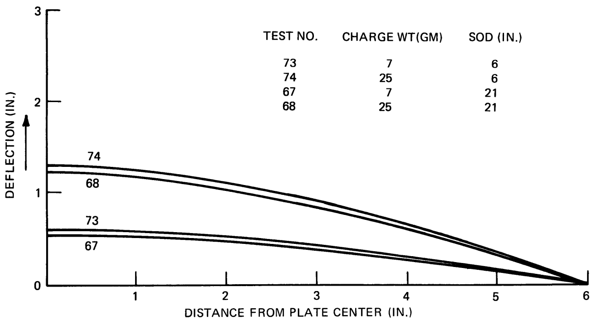
Figure 12o - 3/16-Inch Medium Steel, Air Backed, SOD = 21 Inches and 6 Inches
