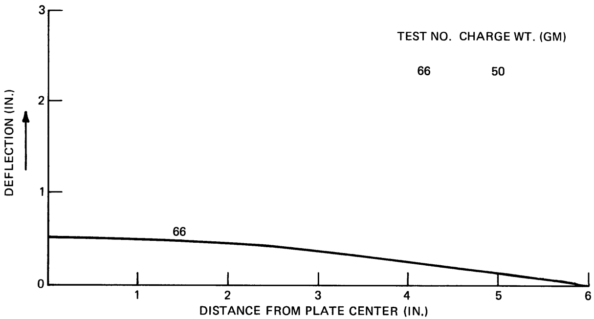
Figure 12d - 1/8-Inch Medium Steel, Water Backed, SOD = 35 Inches
