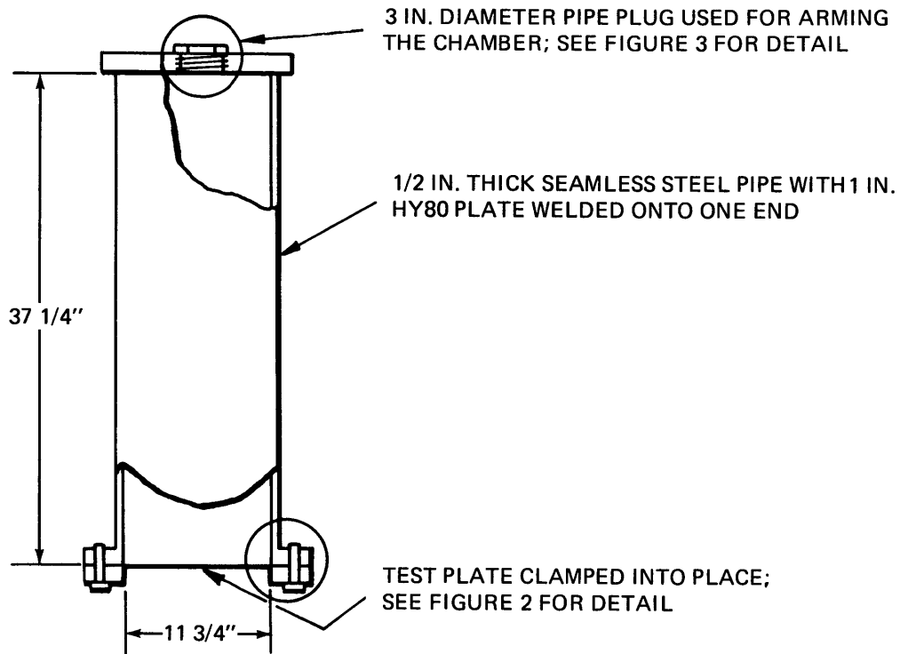
Figure 1 – Explosion Chamber
