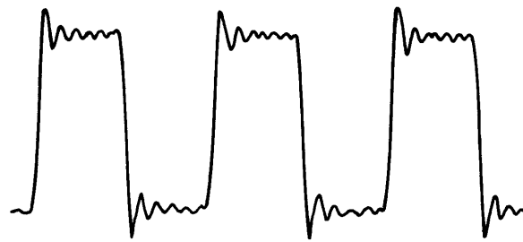
Figure A.3 – A 2-KC Square Wave as Recorded by the Amplifier-Tape Recorder Segment of the Recording System
