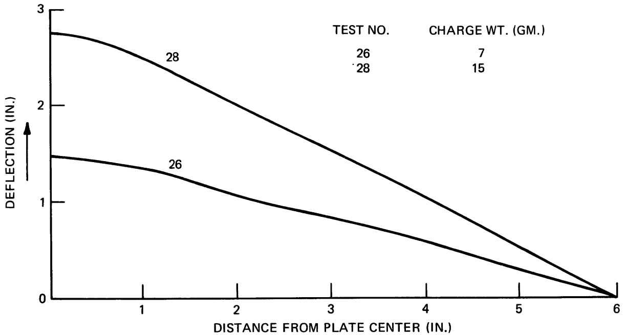
Figure 12e - 1/16-Inch Aluminum, Air Backed, SOD = 35 Inches
