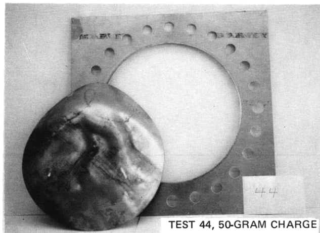
Figure 13f – Edge Failure of a 1/8-Inch Aluminum, Air-Backed Plate (All plates with charge at opposite end of chamber failed in this way)
