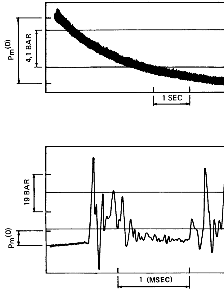
Figure 18 – Comparison between Predicted and Measured Maximum Pressure (A and B represent the same event with different times scales; from Weibull 3 )
