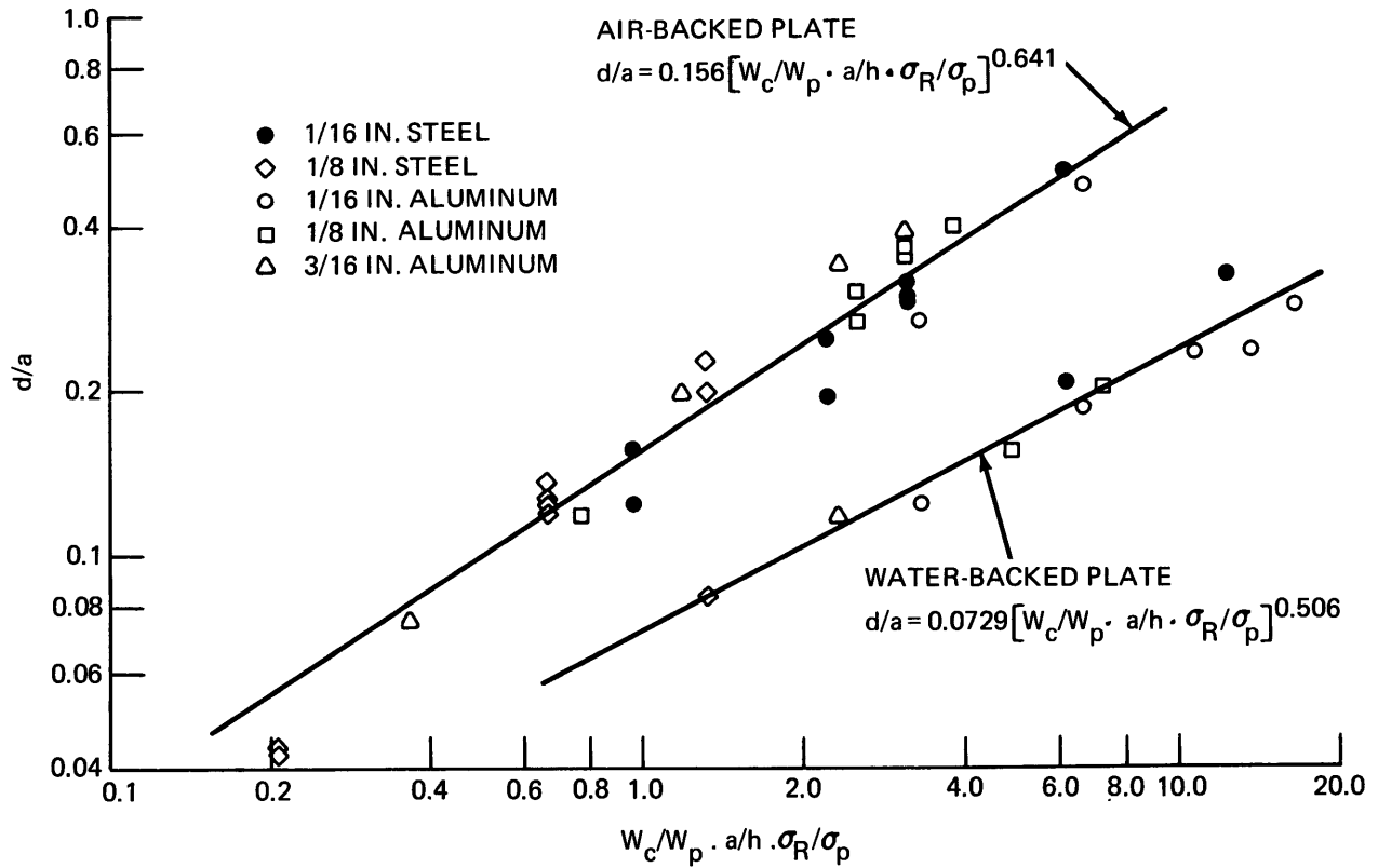
Figure 16a – Plates Tested on the Long Chamber
