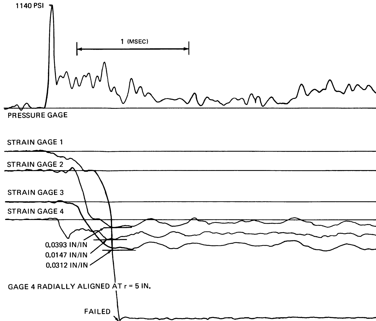
Figure 15e - High-Speed Playback of Test 107 (The 1/16-in. steel plate was loaded by a 15-g Pentolite charge detonated at the 35-in. SOD. The resulting permanent deflection at the plate center was 1.15 in.)
