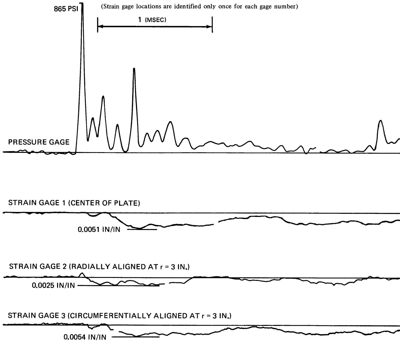
Figure 15a – High-Speed Playback of Test 98
