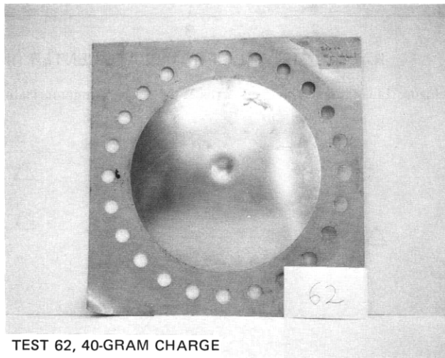
Figure 13e – Water-Backed 1/16-Inch Aluminum Plate Very Near Failure (Note the pronounced dimple at the center)
