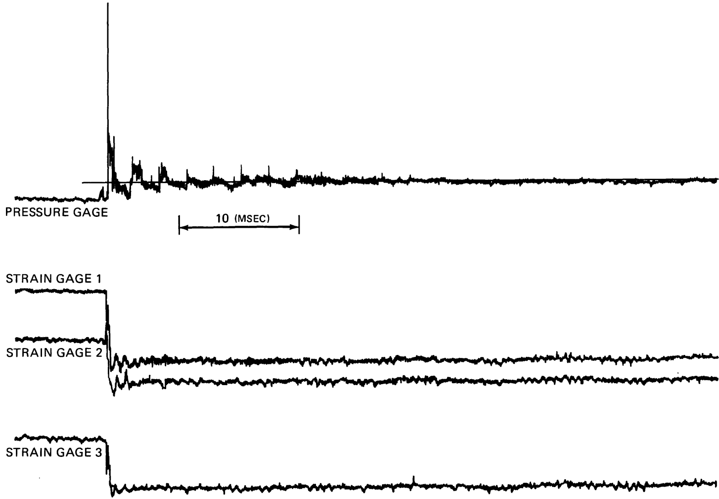
Figure 15d – Slow-Speed Playback of Test 100
