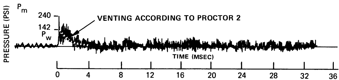
TEST 102 – 25G CHARGE VENTING THROUGH A 108-IN 2 HOLE
