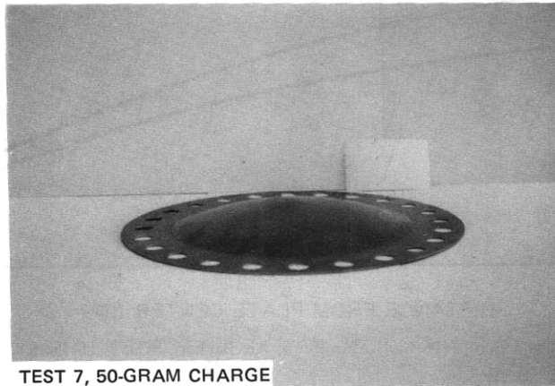
TEST 7, 50-GRAM CHARGE
