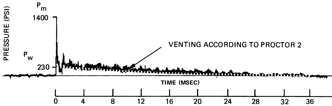
TEST 94 – 50G CHARGE VENTING THROUGH A 6.8-IN 2 HOLE
