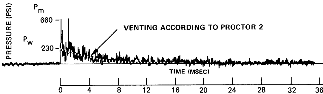
TEST 97 – 50G CHARGE VENTING THROUGH A 27.2-IN 2 HOLE
