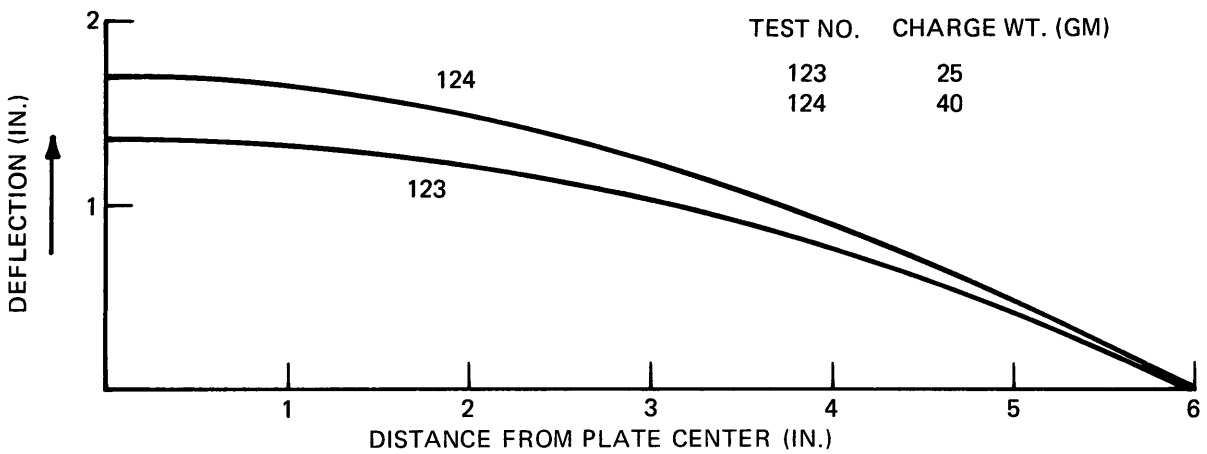
Figure 12n - 3/16-Inch Aluminum, Air Backed, SOD = 16 Inches
