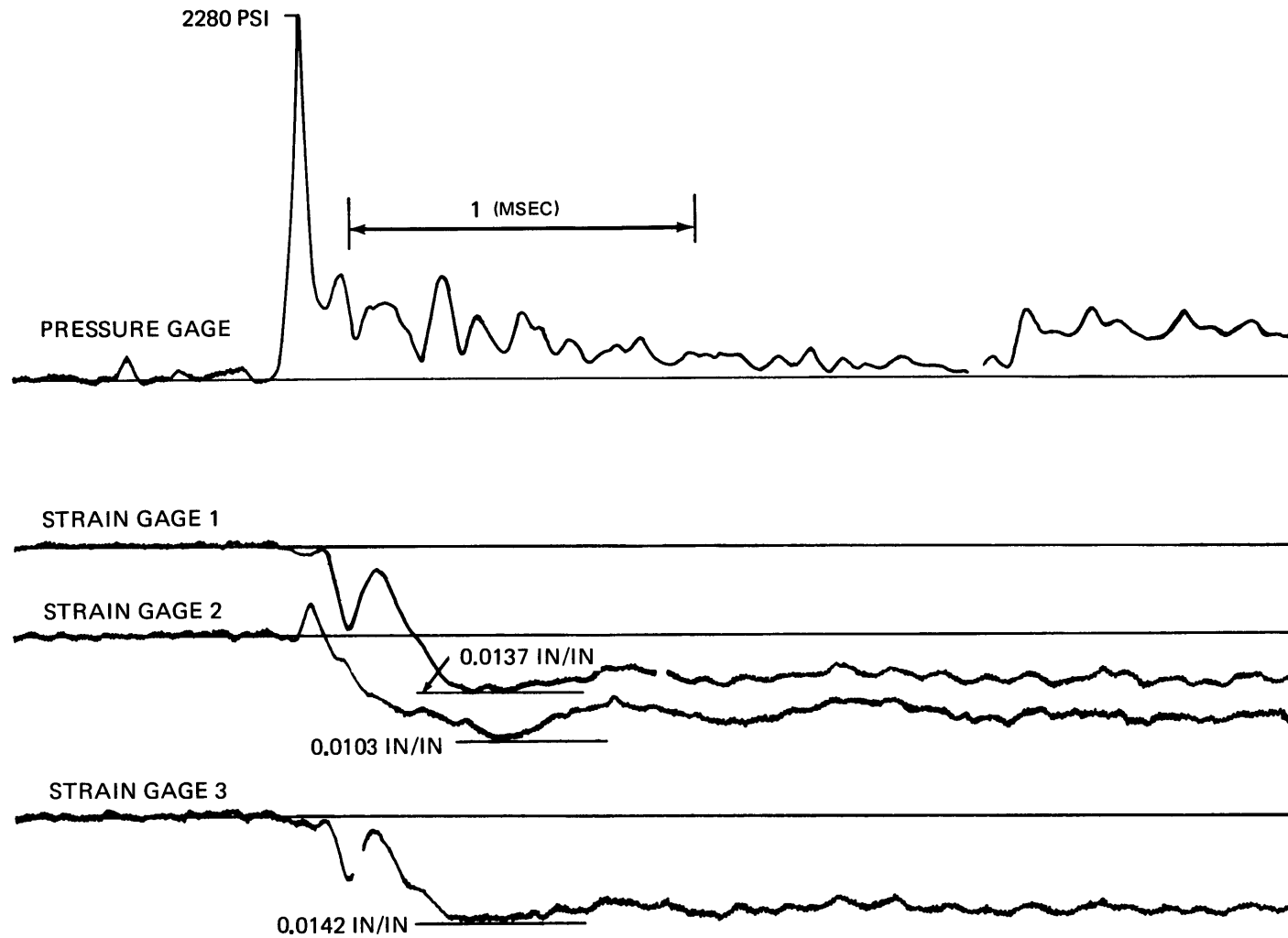
Figure 15c - High-Speed Playback of Test 100
