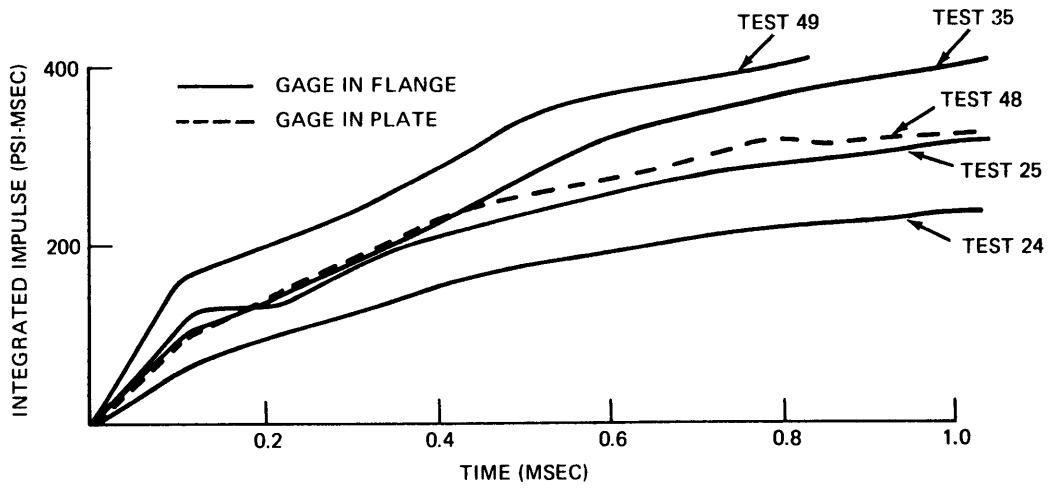
Figure 10c - 25-Gram Charges Detonated at Full SOD
