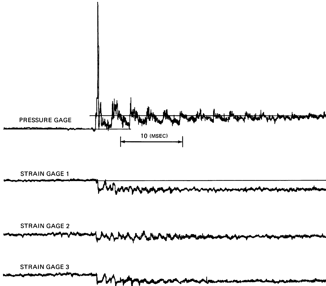
Figure 15b – Slow-Speed Playback of Test 98
