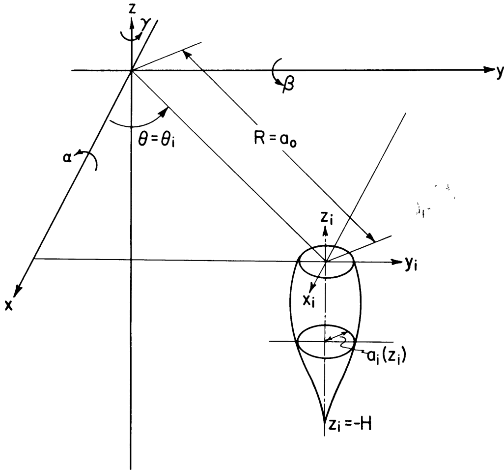
Figure 1 - The i^{\text{th}} Spar in Its Equilibrium Position
