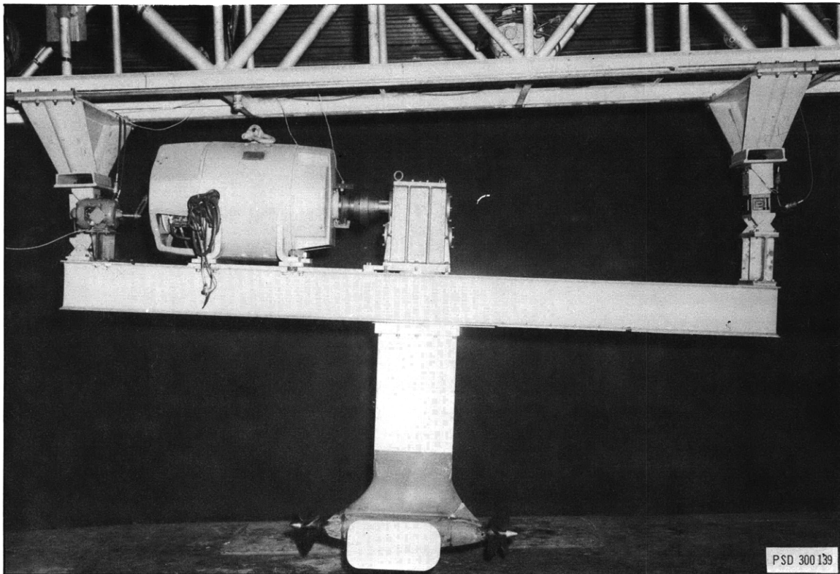
Figure 12 – 500-Horsepower Nacelle Dynamometer Test Setup
