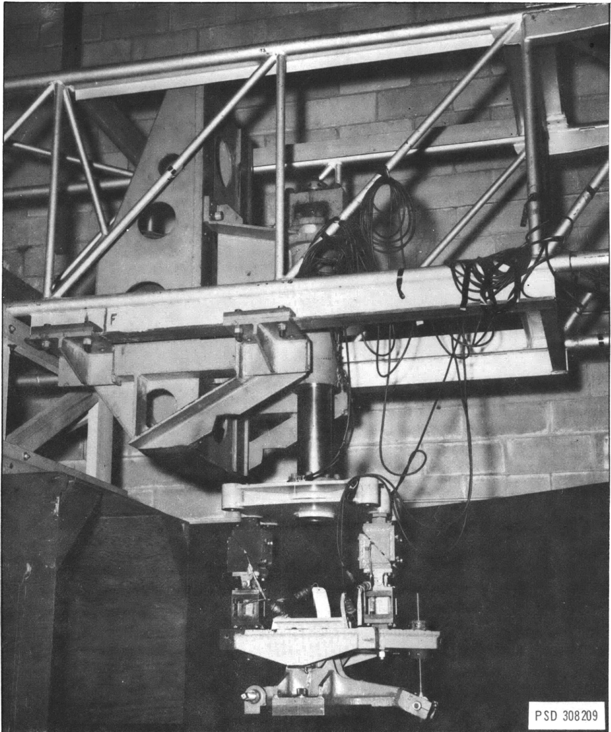
Figure 16 – Hydrofoil Dynamometer with Tow Bridge
