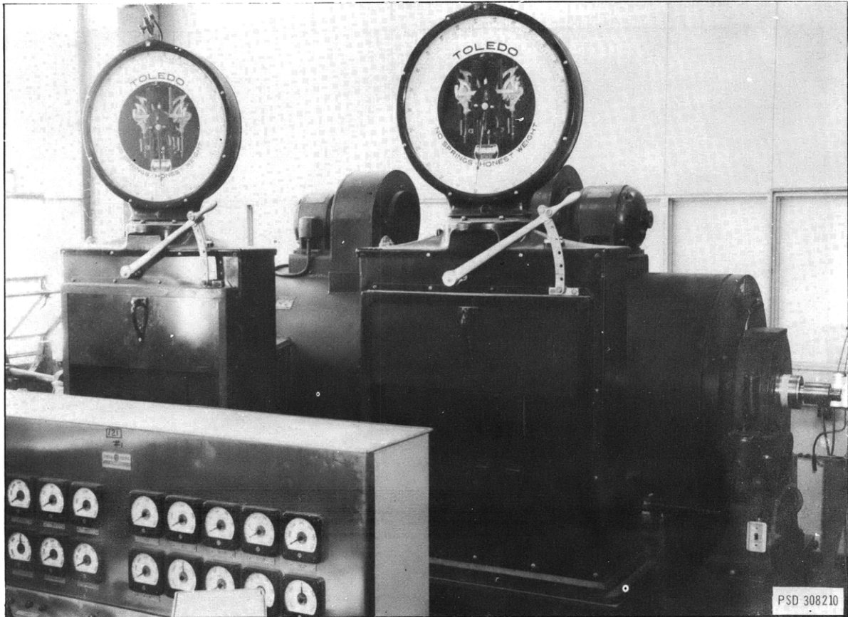
Figure 18 – 400-Horsepower Induction Motor Dynamometers
