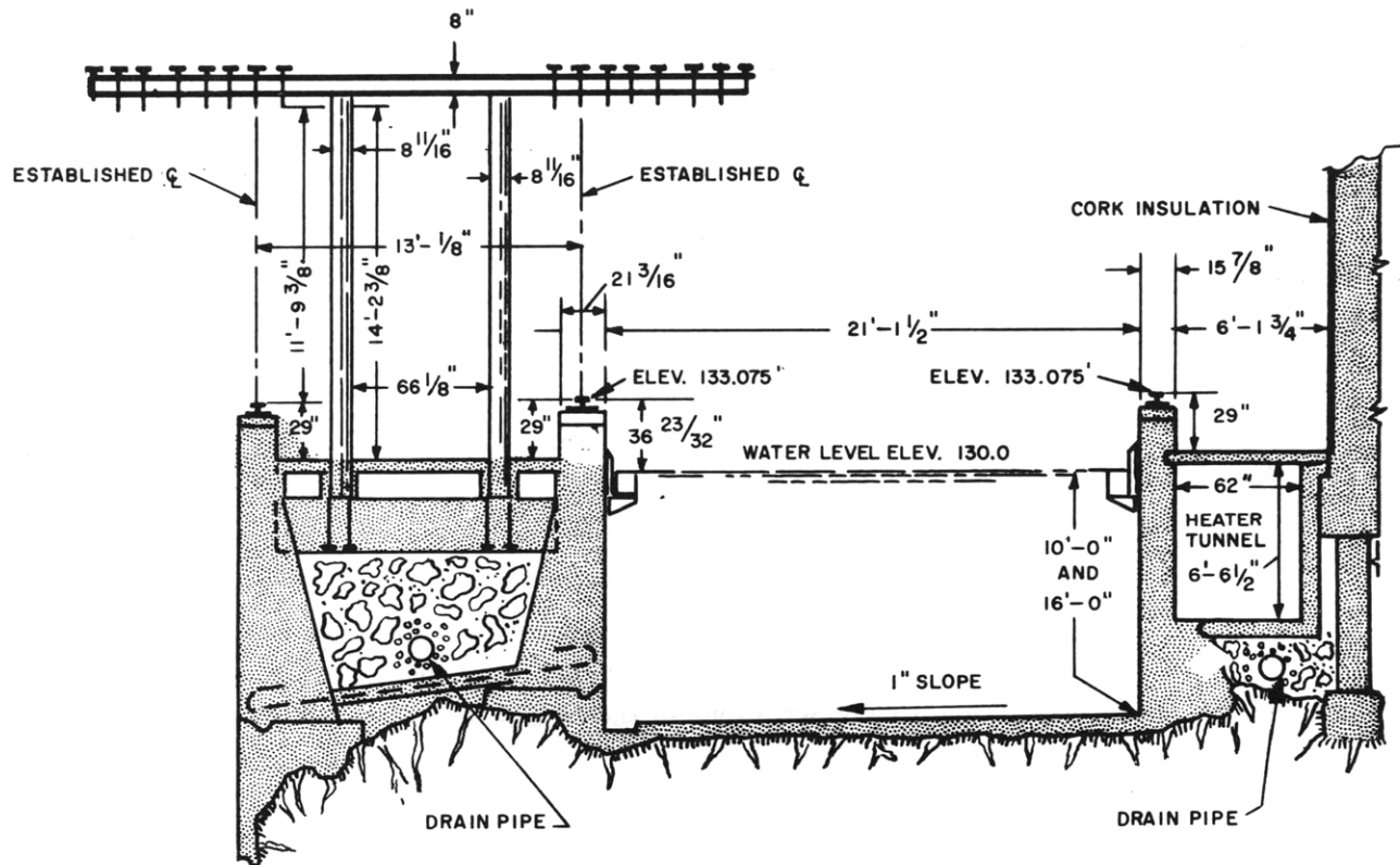
Figure 2 - Cross-Sectional View of High-Speed Basin
