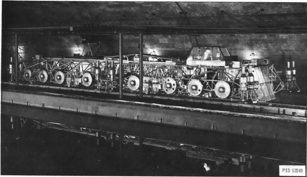
Figure 4 – Carriage 5 with Steel Wheels
