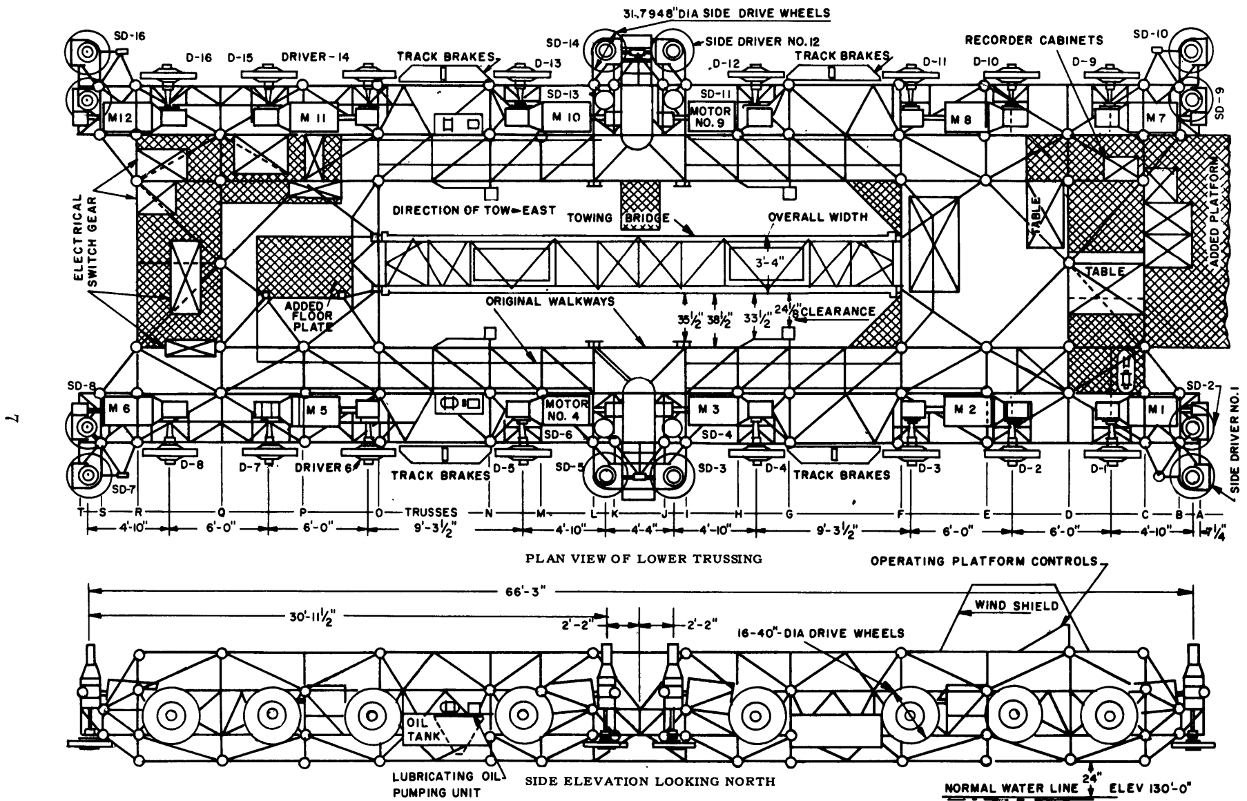
Figure 6 – General Arrangement of Carriage 5
