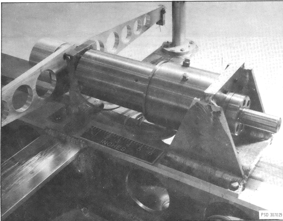
Figure 11 – 500-Horsepower Nacelle Dynamometer in Calibration Stand
