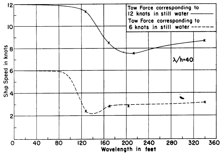
Figure 3 - Reduction of Speed with Constant Tow Force and Wavelength/Waveheight Ratio Length of ship equal to 170 feet.
