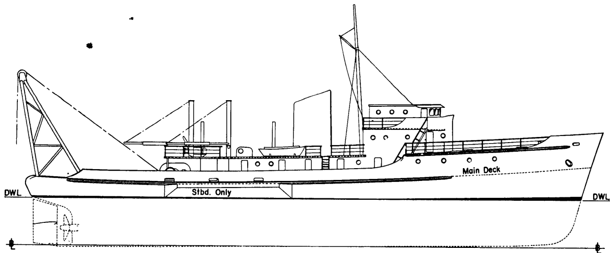
Figure 1b - Outboard Profile (Rev. 2)
