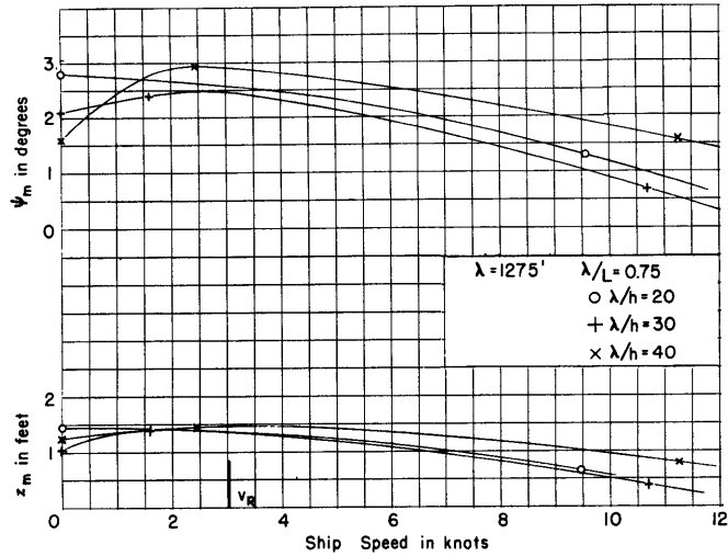
Figure 4a - Wavelength 127.5 Feet
