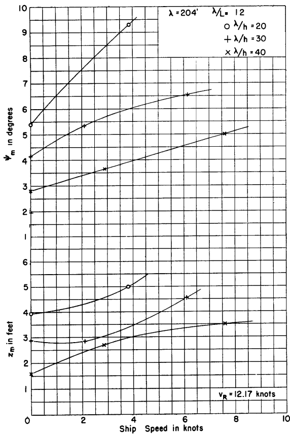
Figure 4c - Wavelength 204 Feet
