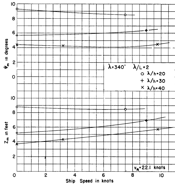
Figure 4d - Wavelength 340 Feet
