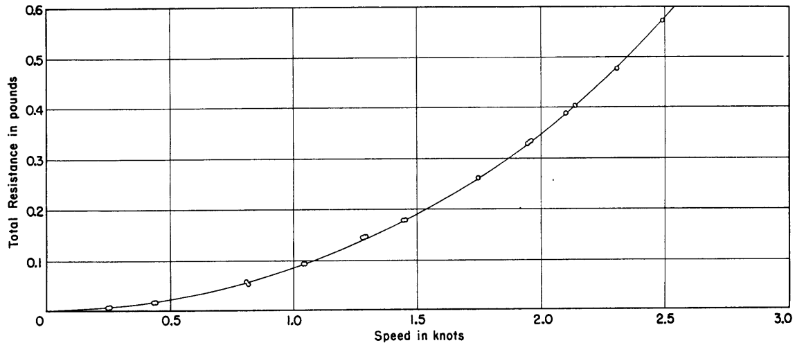
Figure 5 - Total Resistance of Model in Still Water
