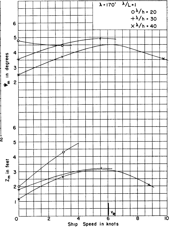
Figure 4b - Wavelength 170 Feet
