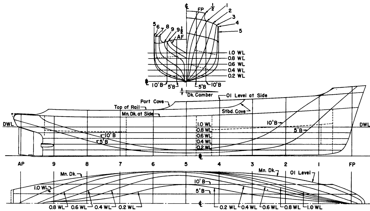
Figure 1a - Preliminary Lines
