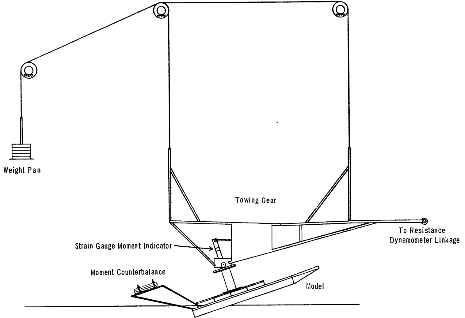
Figure 2 - Setup of Model and Towing Gear
