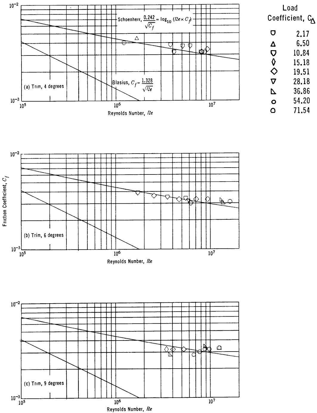
Figure 10 - Variation of Friction Coefficient with Reynolds Number
