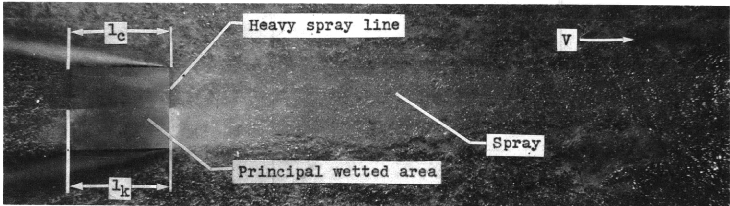
Figure 3b - Typical Photograph for High Trim Angles
