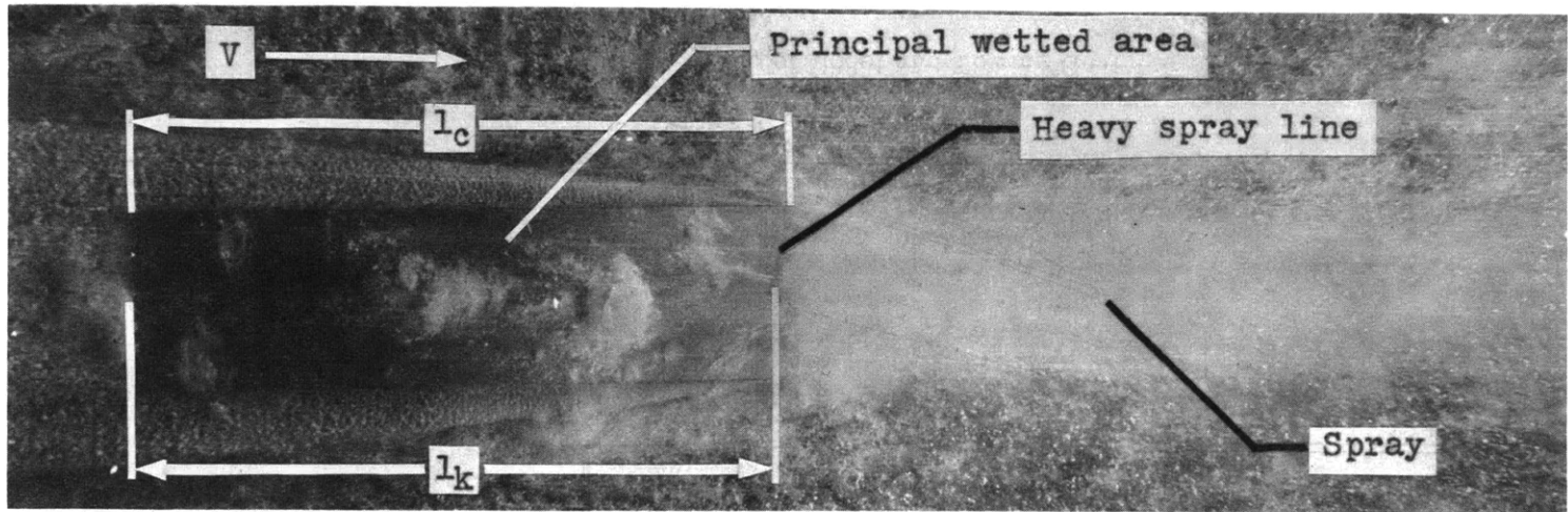
Figure 3a - Typical Photograph for Low Trim Angles Showing Air Bubbles Beneath Principal Wetted Area
