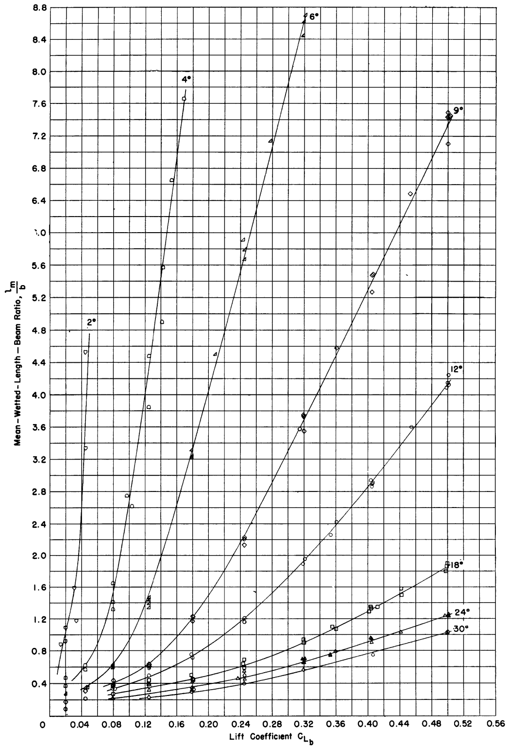
Figure 4 - Variation of Mean-Wetted-Length-Beam Ratio l_m/b with Lift Coefficient C_{Lb}
