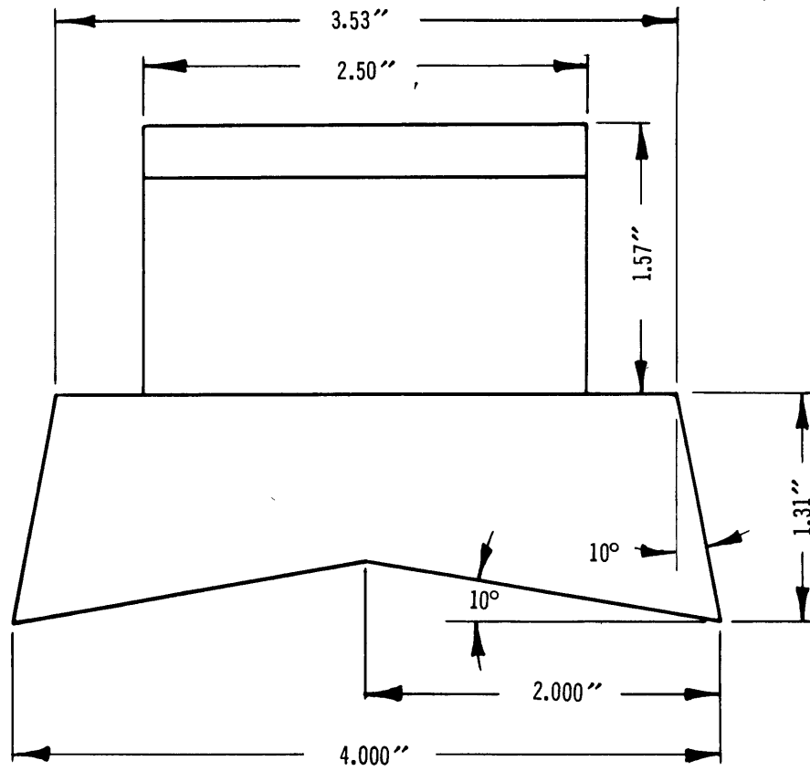
Figure 1 - Cross Section and Sketch of Model
