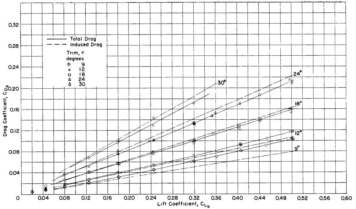
Figure 9 - Variation of Drag Coefficient with Lift Coefficient
