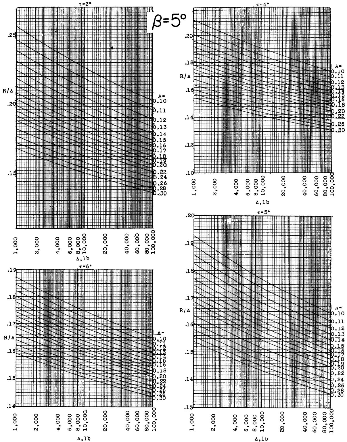
(b) \tau = 3^\circ, 4^\circ, 5^\circ, \text{ and } 6^\circ
