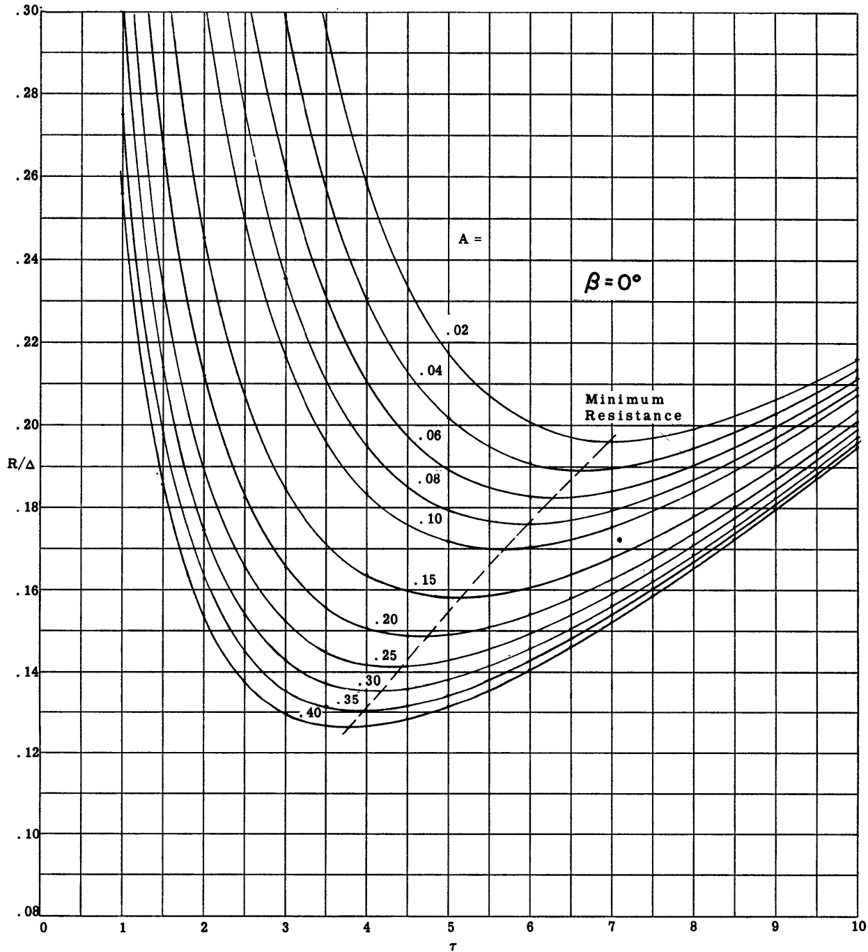
(a) \beta = 0^\circ
