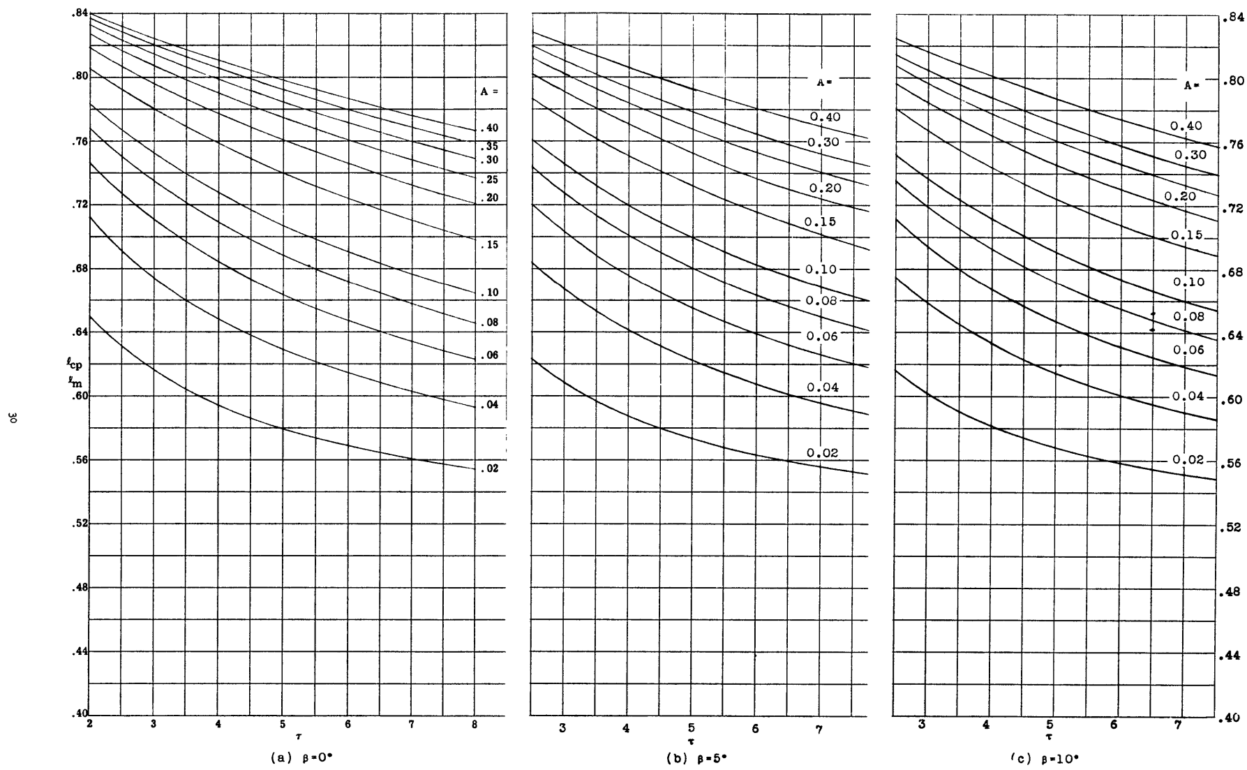
Figure 10 - Center-of-Pressure/Mean-Wetted-Length Ratio Versus Trim Angle
