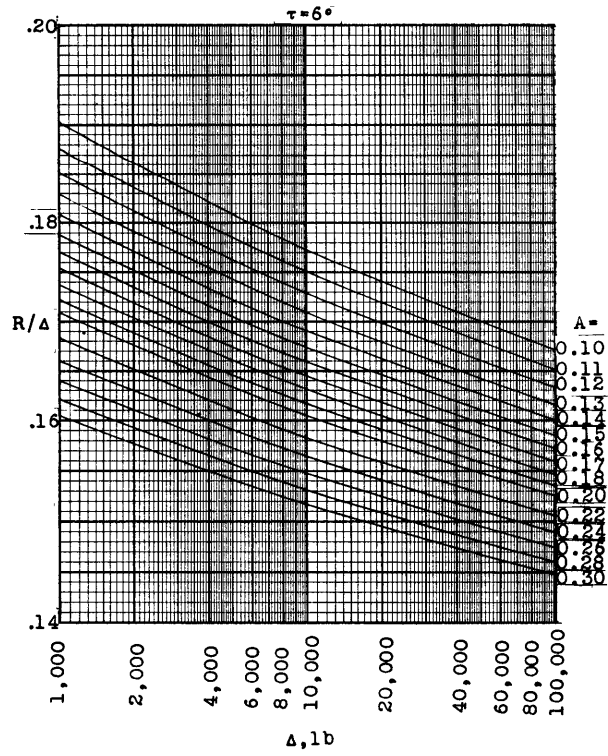
(b) \tau = 3^\circ, 4^\circ, 5^\circ, \text{ and } 6^\circ
