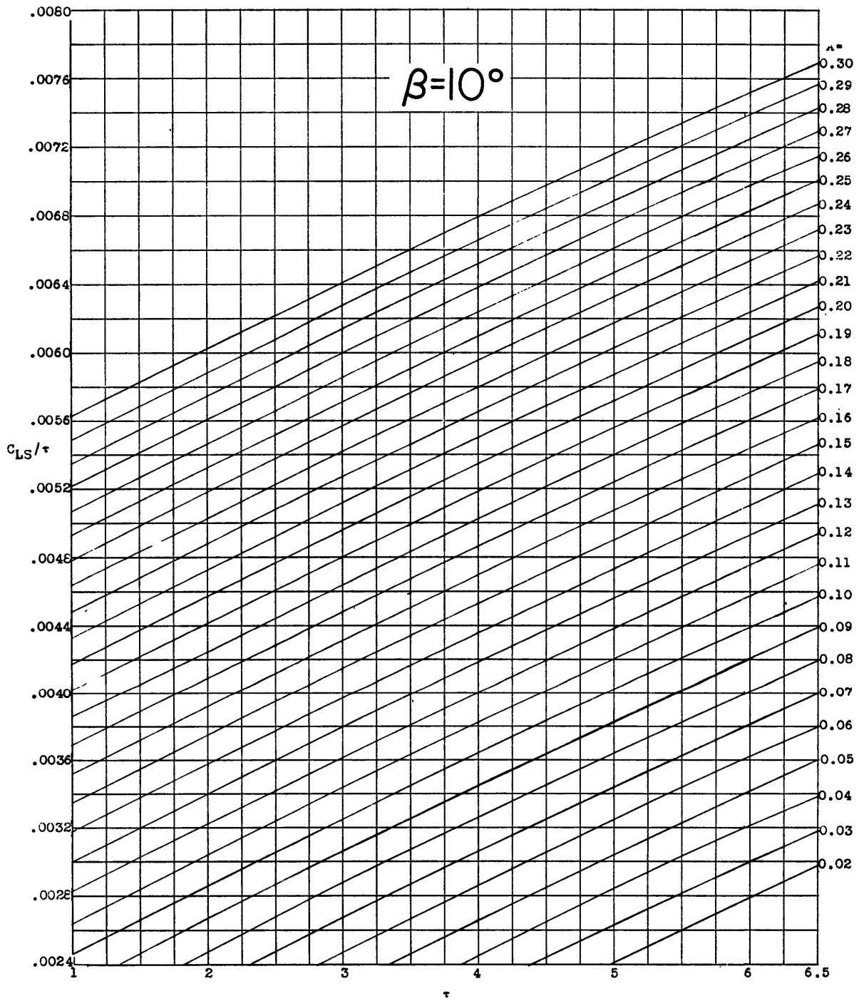
(c) \beta = 10^\circ Figure 1 - Concluded.
