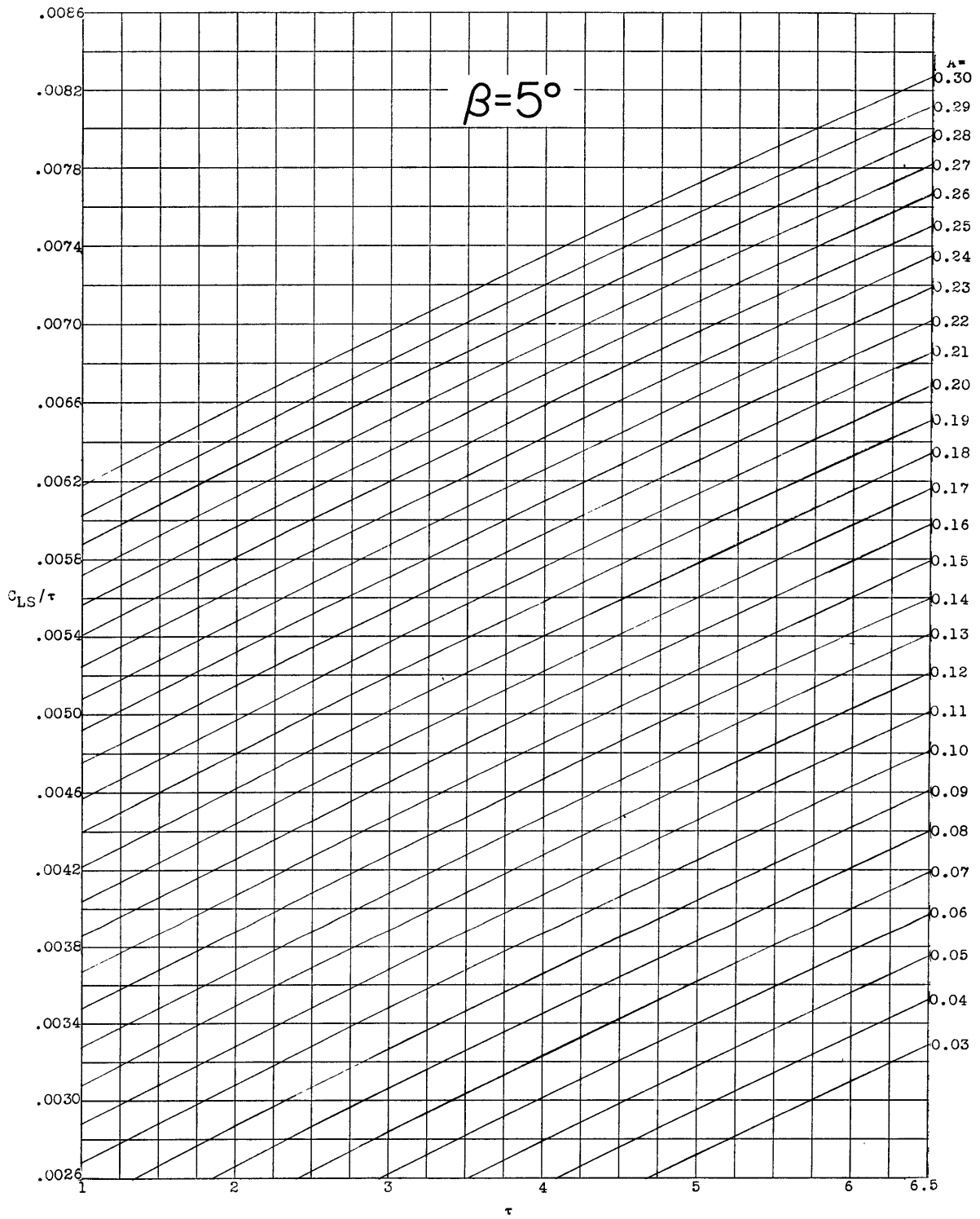
(b) \beta = 5^\circ Figure 1 - Continued.
