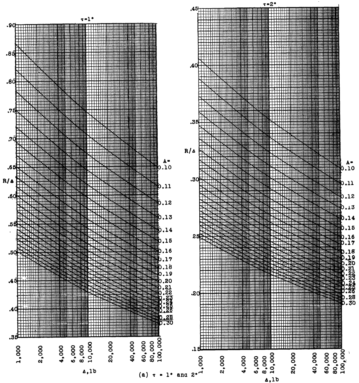
Figure 6 - Resistance/Weight Ratio Versus weight. \beta = 10^\circ
