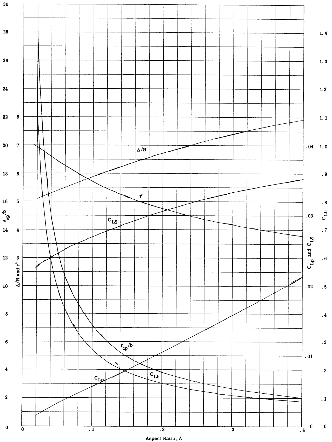
(a) \beta = 0^\circ
