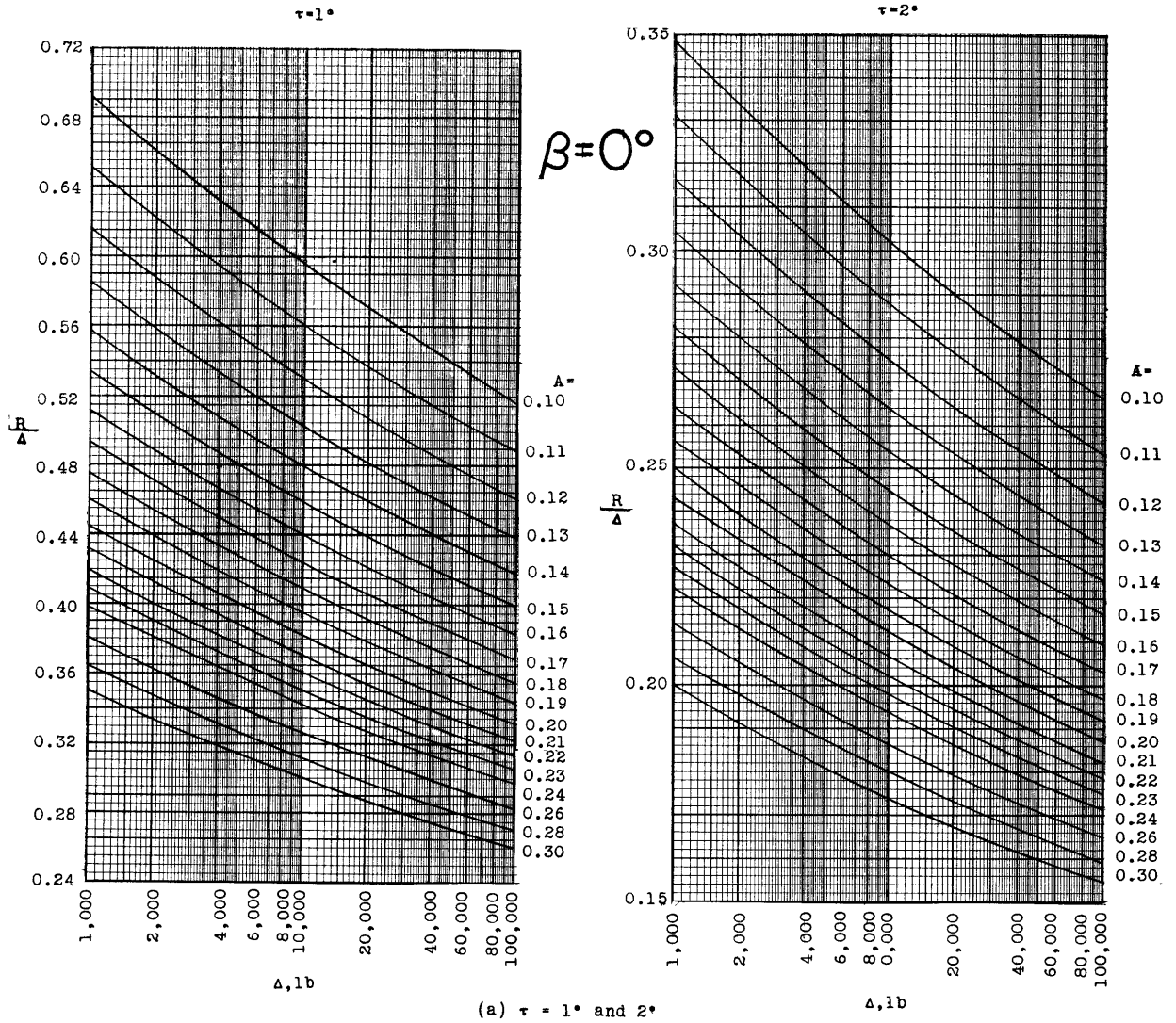
Figure 4 - Resistance/Weight Ratio Versus Weight. \beta = 0^\circ
