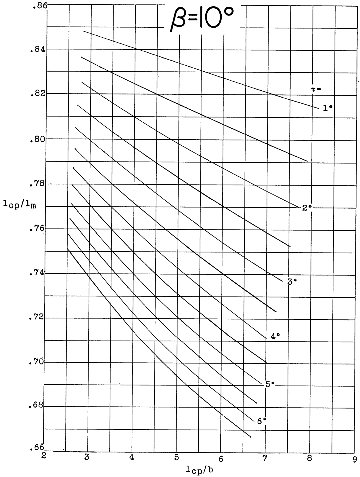
(c) \beta = 10^\circ Figure 2 - Concluded.
