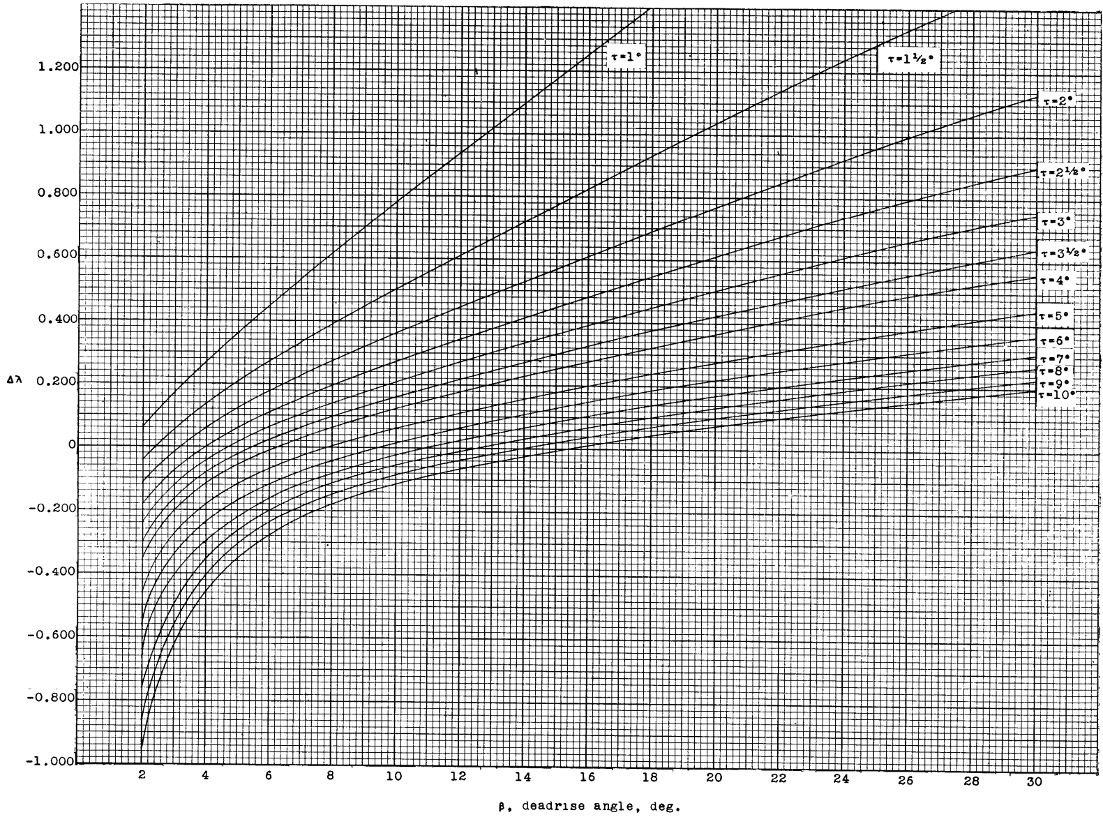
Figure 7 - Effective Increase in Friction-Area Length-Beam Ratio ( \Delta\lambda ) Due to Spray Contribution to Drag
