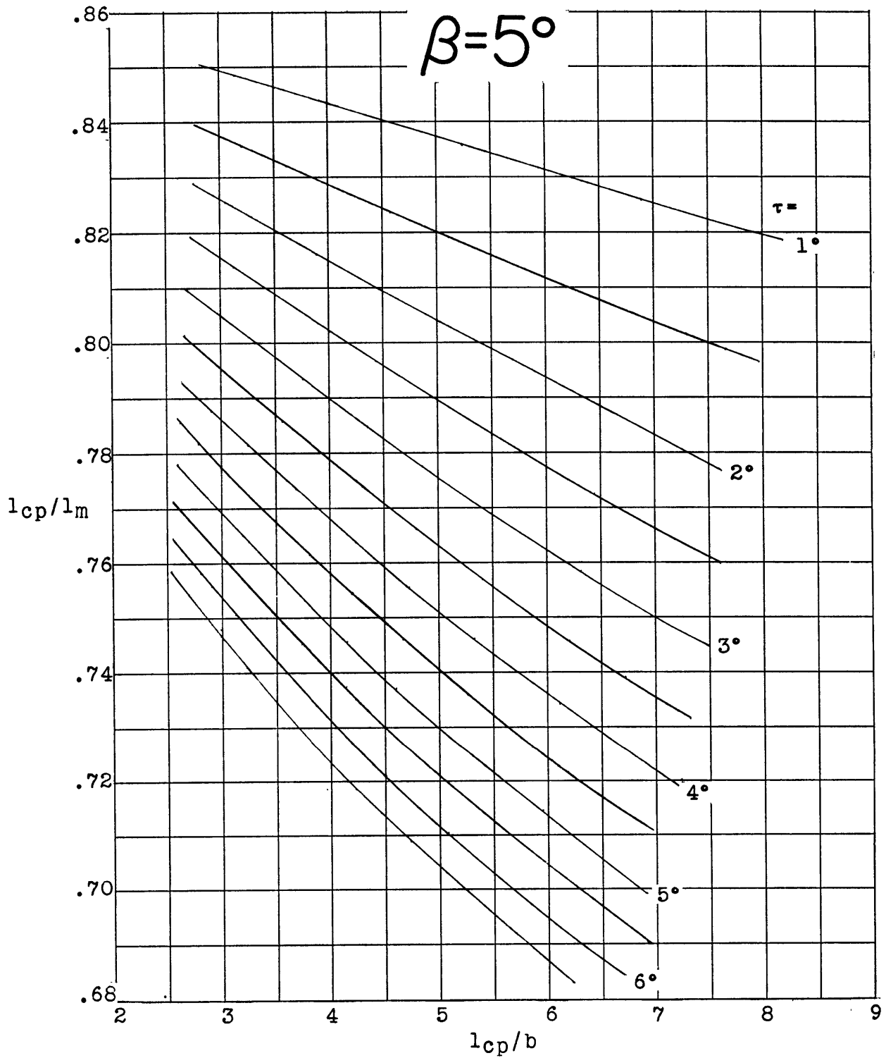
(b) \beta = 5^\circ Figure 2 - Continued.
