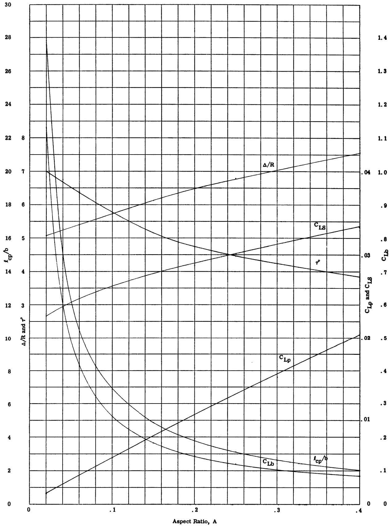
Figure 9 (continued) - Optimum Values of Lift/Drag ( \Delta/R ) for Planing Hulls of Low Aspect Ratio, and the Corresponding Values of \tau , C_{Lb} , f_{cp}/b , and C_{LS}
