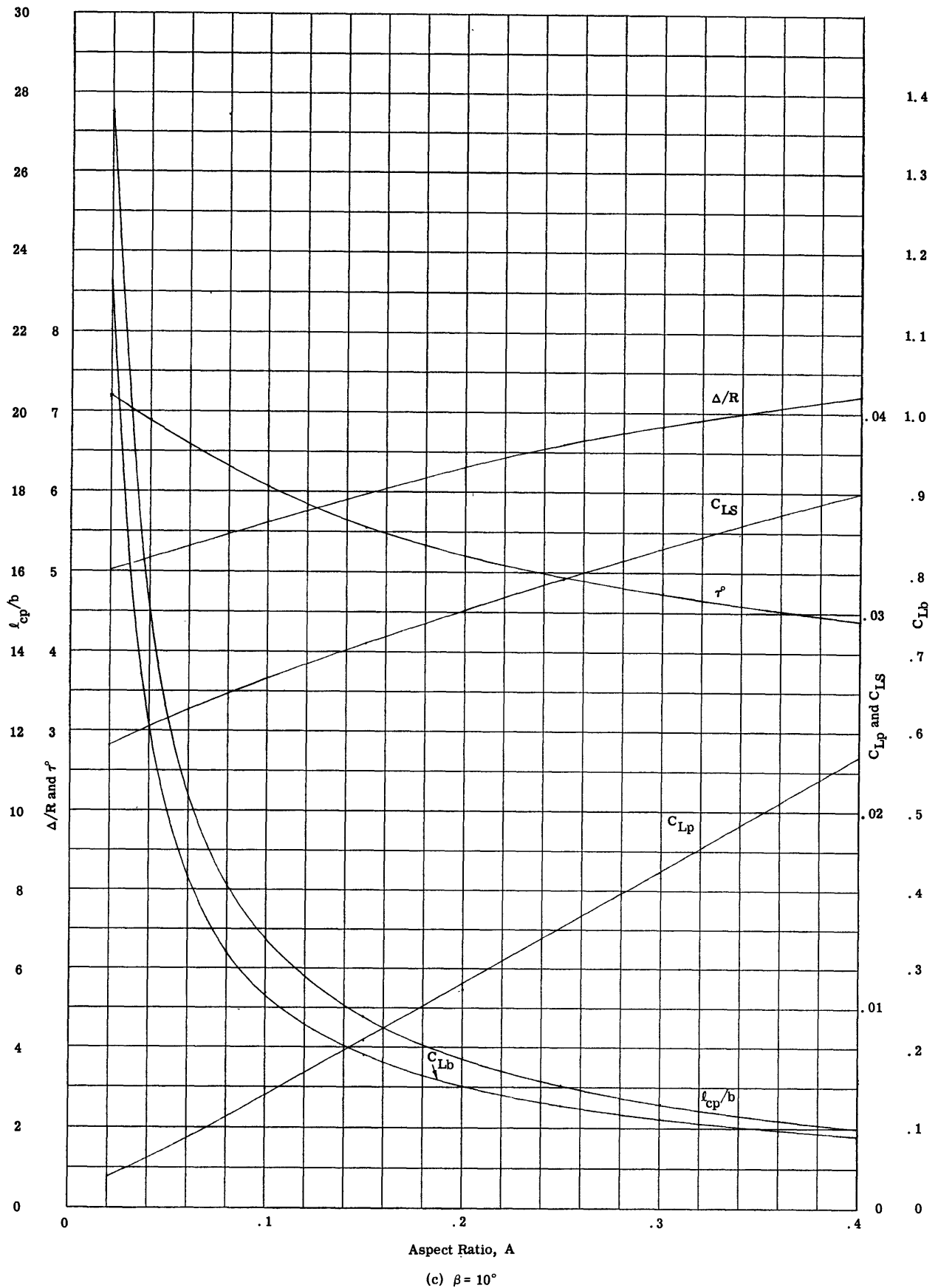
Figure 9 (concluded) - Optimum Values of Lift/Drag ( \Delta/R ) for Planing Hulls of Low Aspect Ratio, and the Corresponding Values of \tau , C_{Lb} , \ell_{cp}/b , and C_{LS}
