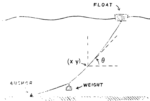
Figure 1 - Mooring line
