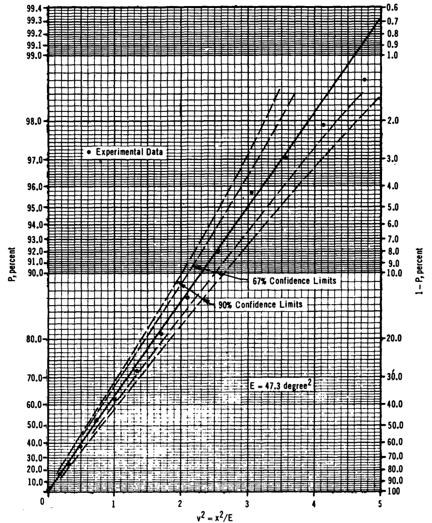
Figure 4 - Cumulative Distribution of Variation in Pitch Angle (Sample 1) for USCGC UNIMAK
