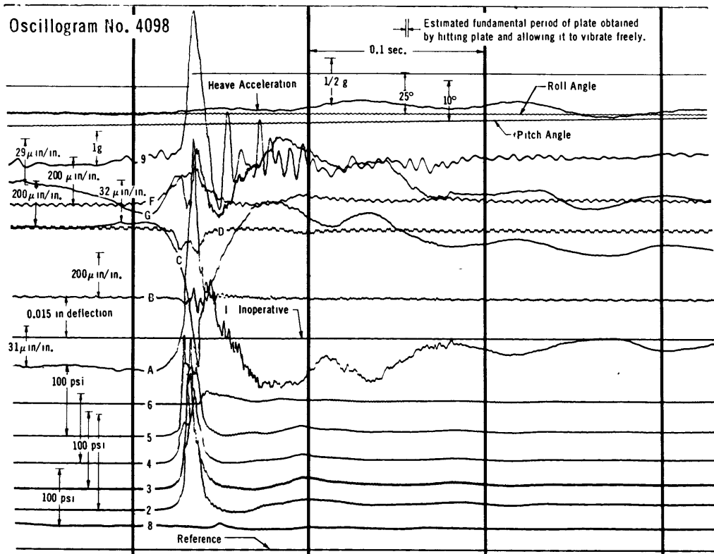
Figure 11 - Samples of Records Taken During the Tests
