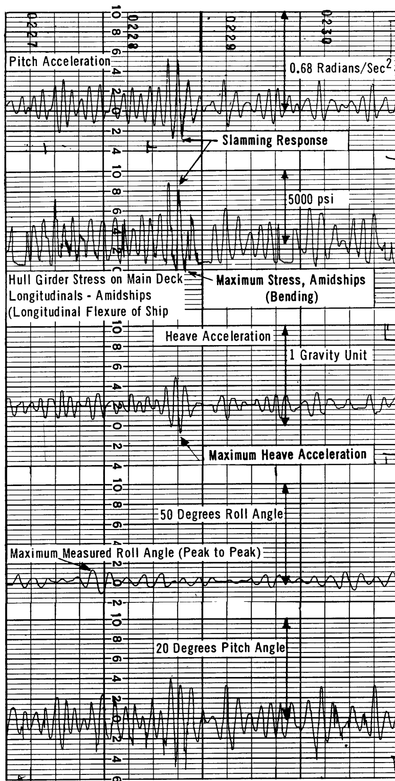
Figure 11e - Oscillogram at Time of Maximum Measured Stress and Heave Acceleration 1 Feb 1955
