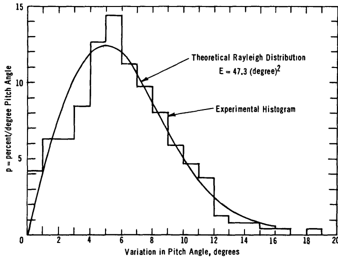
Figure 3 - Distribution of Variation in Pitch Angle (Sample 1) for USCGC UNIMAK
