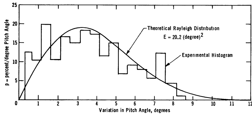
Figure 5 - Distribution of Variation in Pitch Angle (Sample 2) for USCGC UNIMAK
