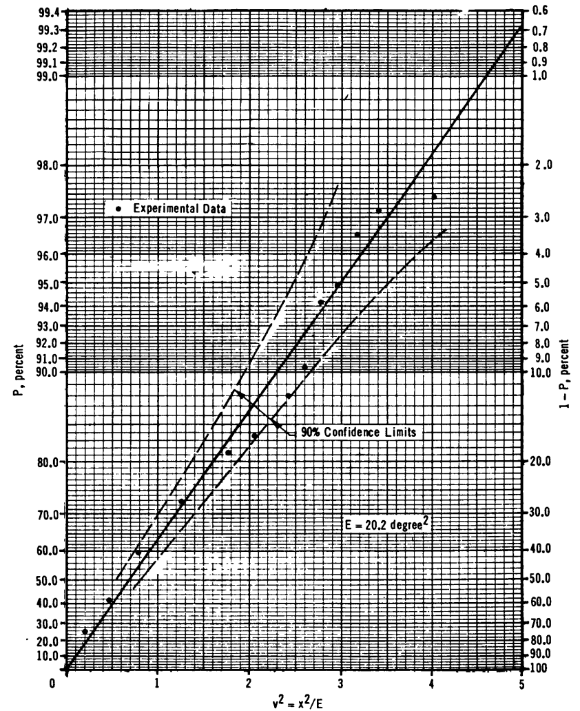
Figure 6 - Cumulative Distribution of Variation in Pitch Angle (Sample 2) for USCGC UNIMAK
