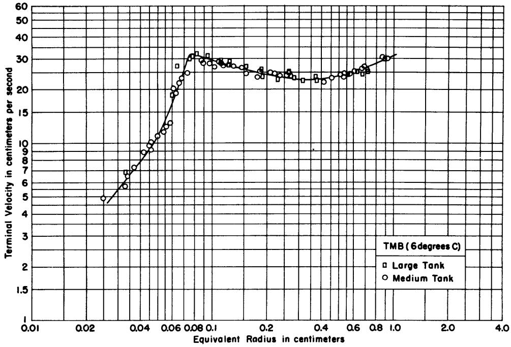
Figure 6 - Terminal Velocity of Air Bubbles in Cold Filtered Water as a Function of Bubble Size
