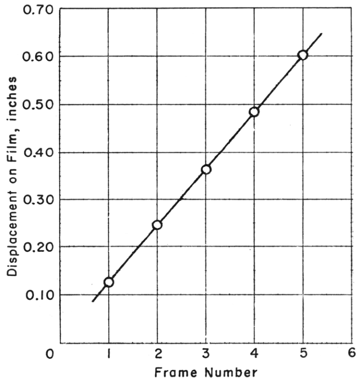
Figure 3 - Evaluation of Velocity of Rise of Bubbles
