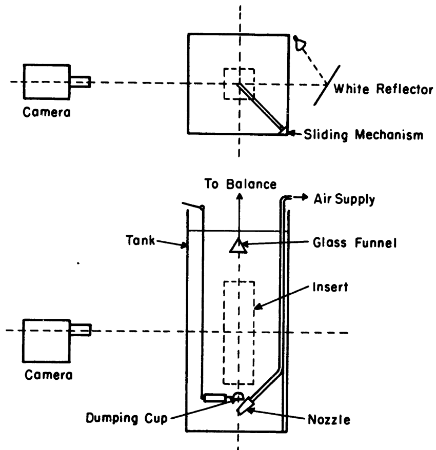
Figure 1 - Experimental Setup
