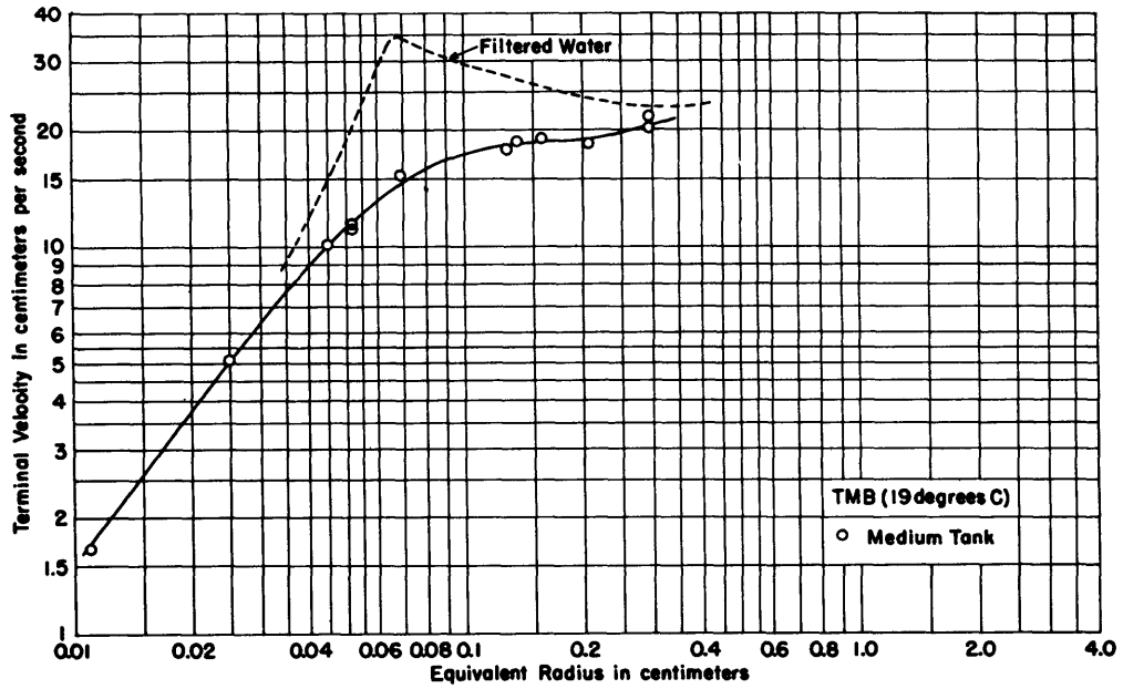
Figure 8 - Terminal Velocity of Air Bubbles in Water Containing Glim as a Function of Bubble Size
