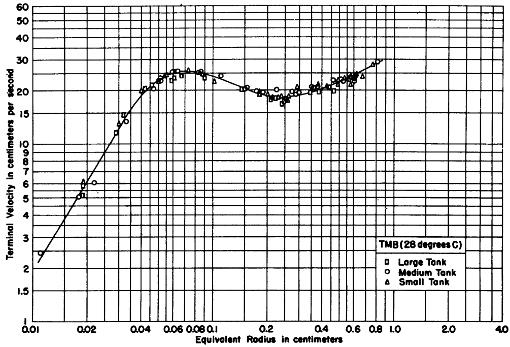
Figure 10 - Terminal Velocity of Air Bubbles in Varsol as a Function of Bubble Size
