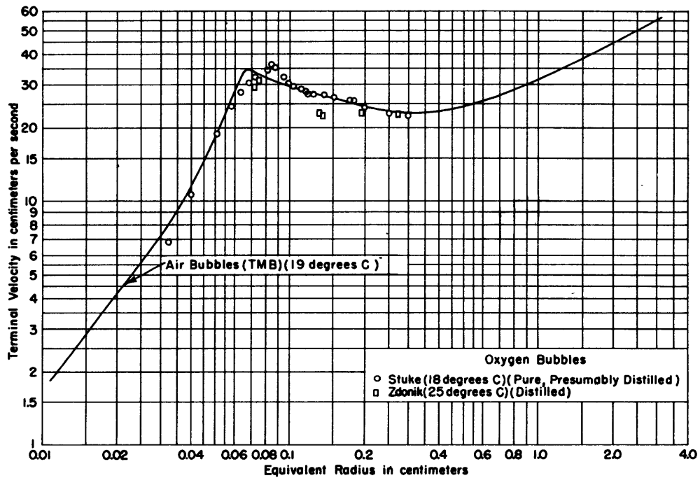
Figure 30 - Terminal Velocity of Gas Bubbles in Distilled Water as a Function of Bubble Size
