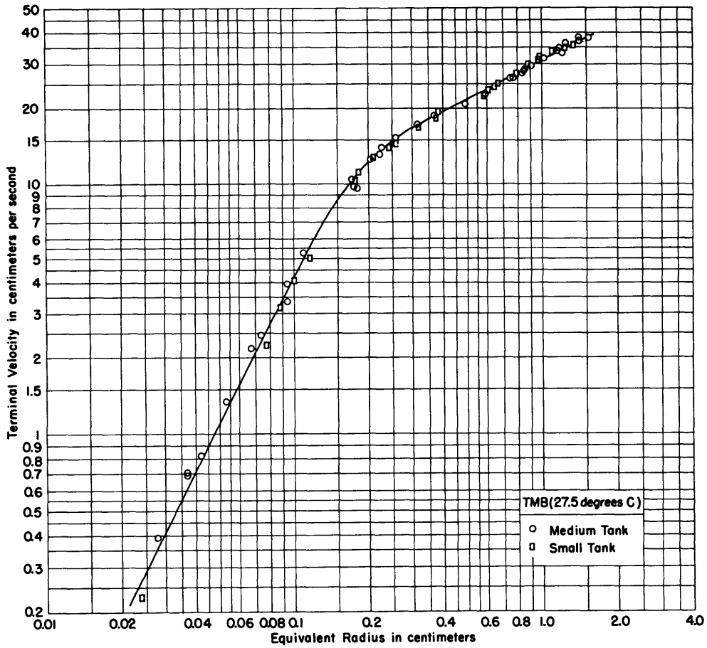
Figure 9 - Terminal Velocity of Air Bubbles in Mineral Oil as a Function of Bubble Size
