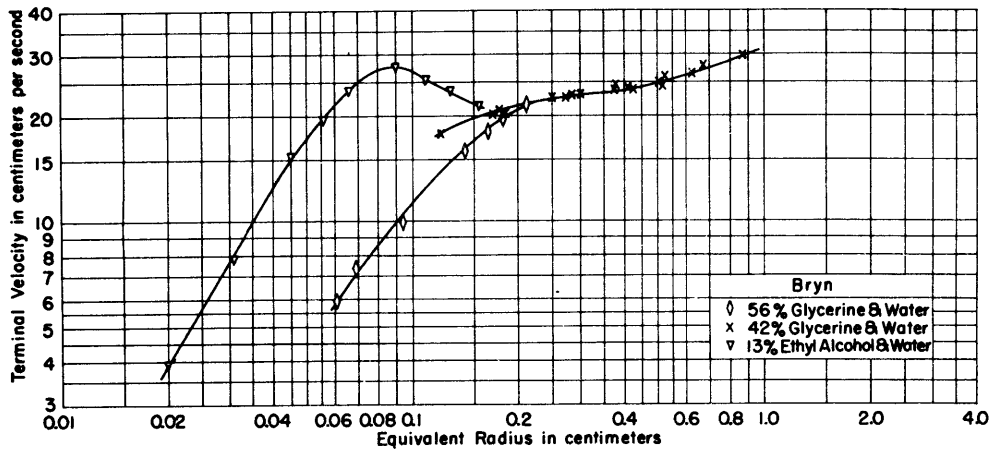
Figure 14 - Terminal Velocity of Air Bubbles in Liquids as Obtained from Bryn's Data
