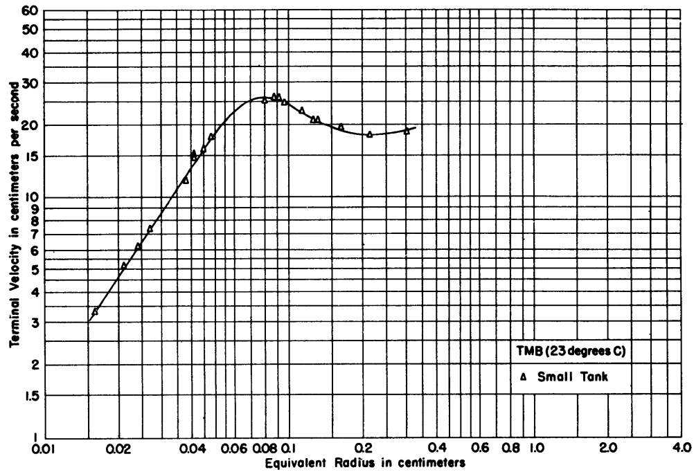
Figure 11 - Terminal Velocity of Air Bubbles in Turpentine as a Function of Bubble Size
