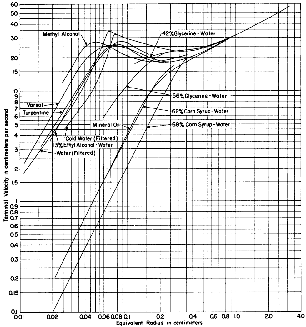
Figure 15 - Comparison of Terminal Velocities of Air Bubbles in Various Liquids
