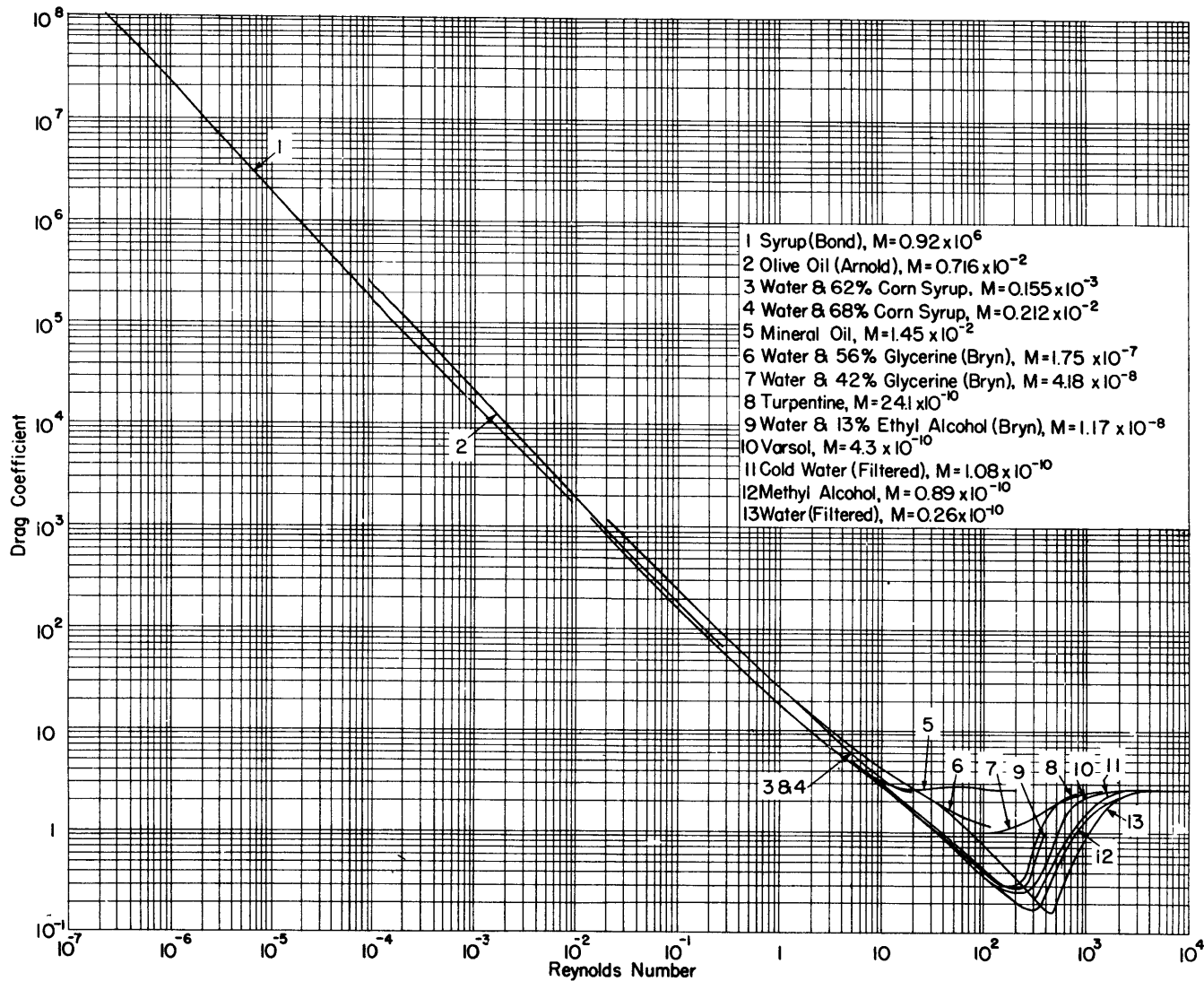
Figure 16 - Drag Coefficient as a Function of Reynolds Number for Air Bubbles Rising at Their Terminal Velocity in Various Liquids
