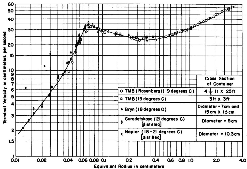
Figure 4 - Terminal Velocity of Air Bubbles in Filtered or Distilled Water as a Function of Bubble Size
