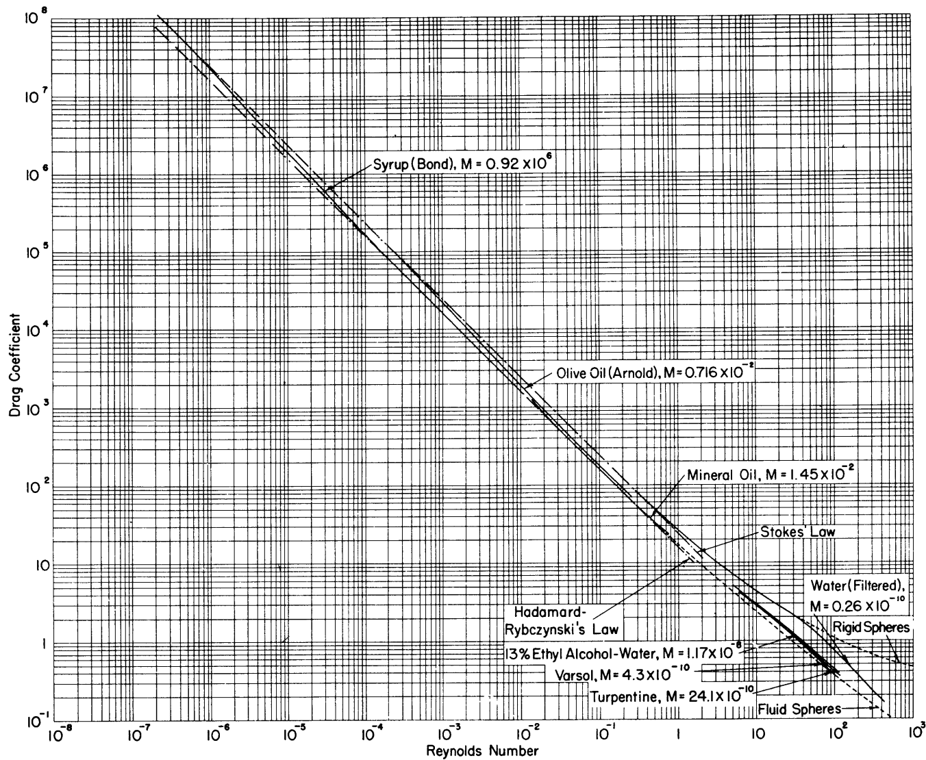
Figure 19 - Drag Coefficient as a Function of Reynolds Number for Spherical Air Bubbles Rising at Their Terminal Velocity in Various Liquids
