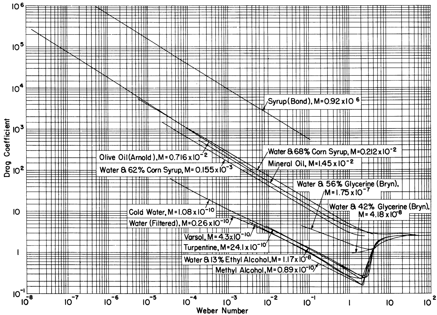
Figure 17 - Drag Coefficient as a Function of Weber Number for Air Bubbles Rising at Their Terminal Velocity in Various Liquids
