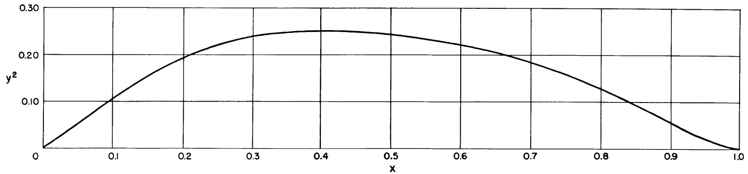
Figure 3 - Graph of a Typical Body and Sectional-Area Curve Computed from a Sixth-Degree Polynomial
