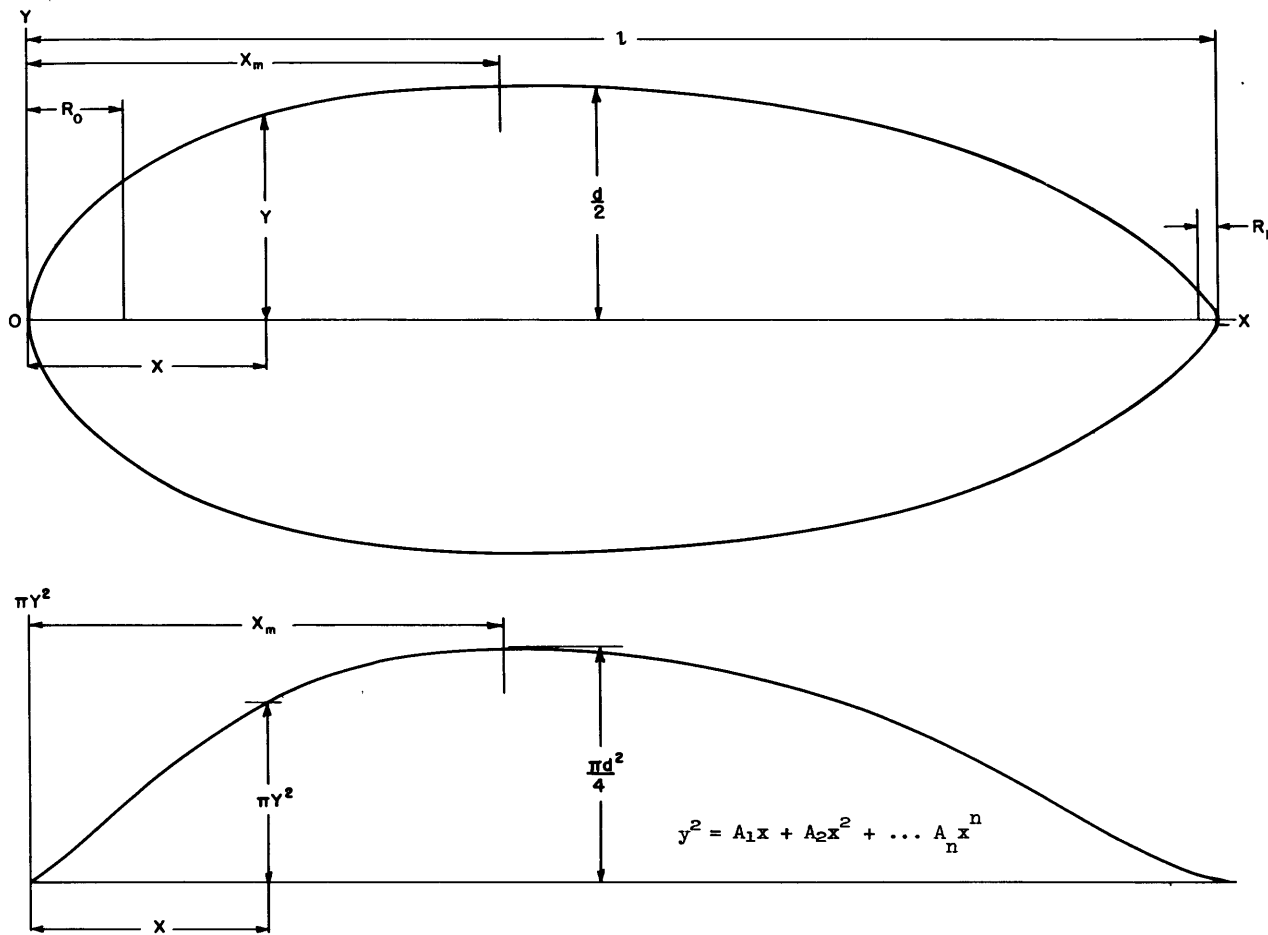
Figure 1 - Sketch Showing Principal Dimensions of a Body of Revolution and Its Sectional-Area Curve
