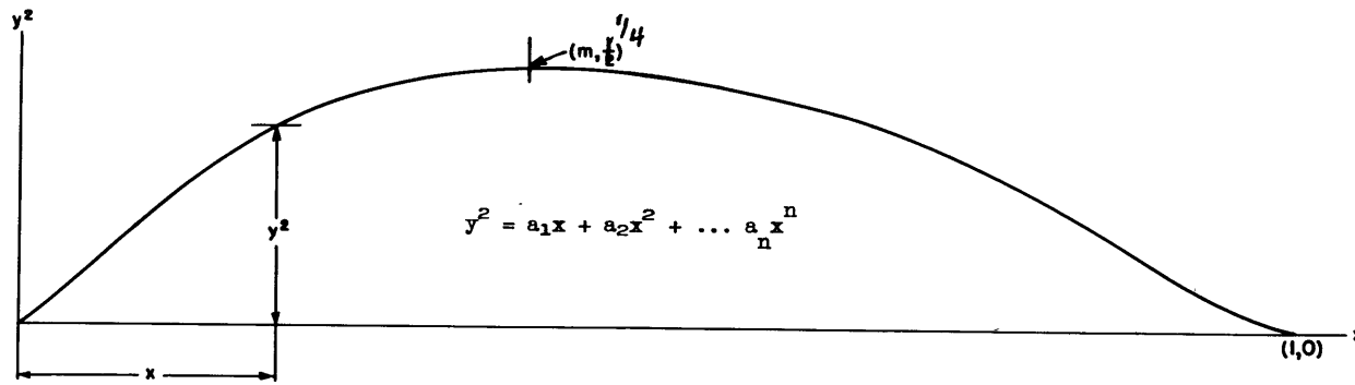
Figure 2 - Nondimensional Representation of a Sectional-Area Curve
