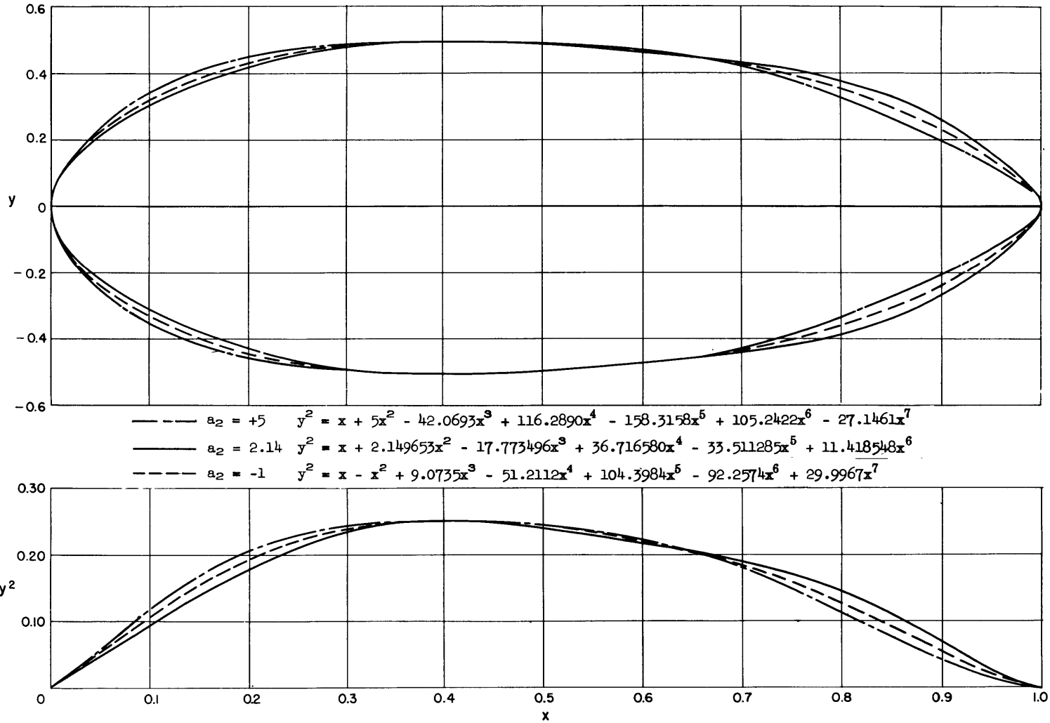
Figure 6 - Forms Derived from Seventh-Degree Polynomials Showing the Effect of Varying the Parameter a_2
