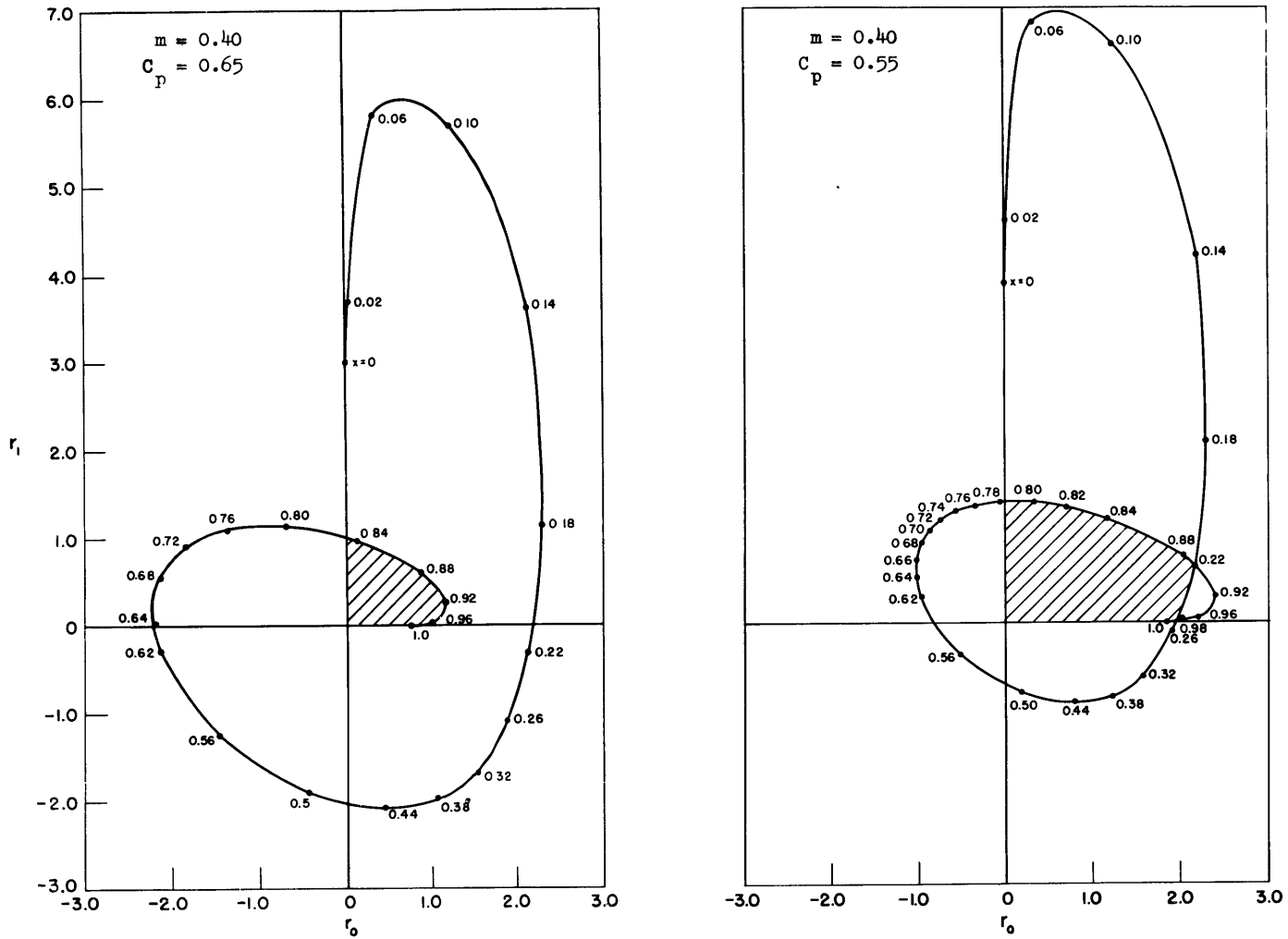
Figure 4 - Typical Envelope Curves of r_1 and r_0 Defined by the Maximum-Minimum Condition
