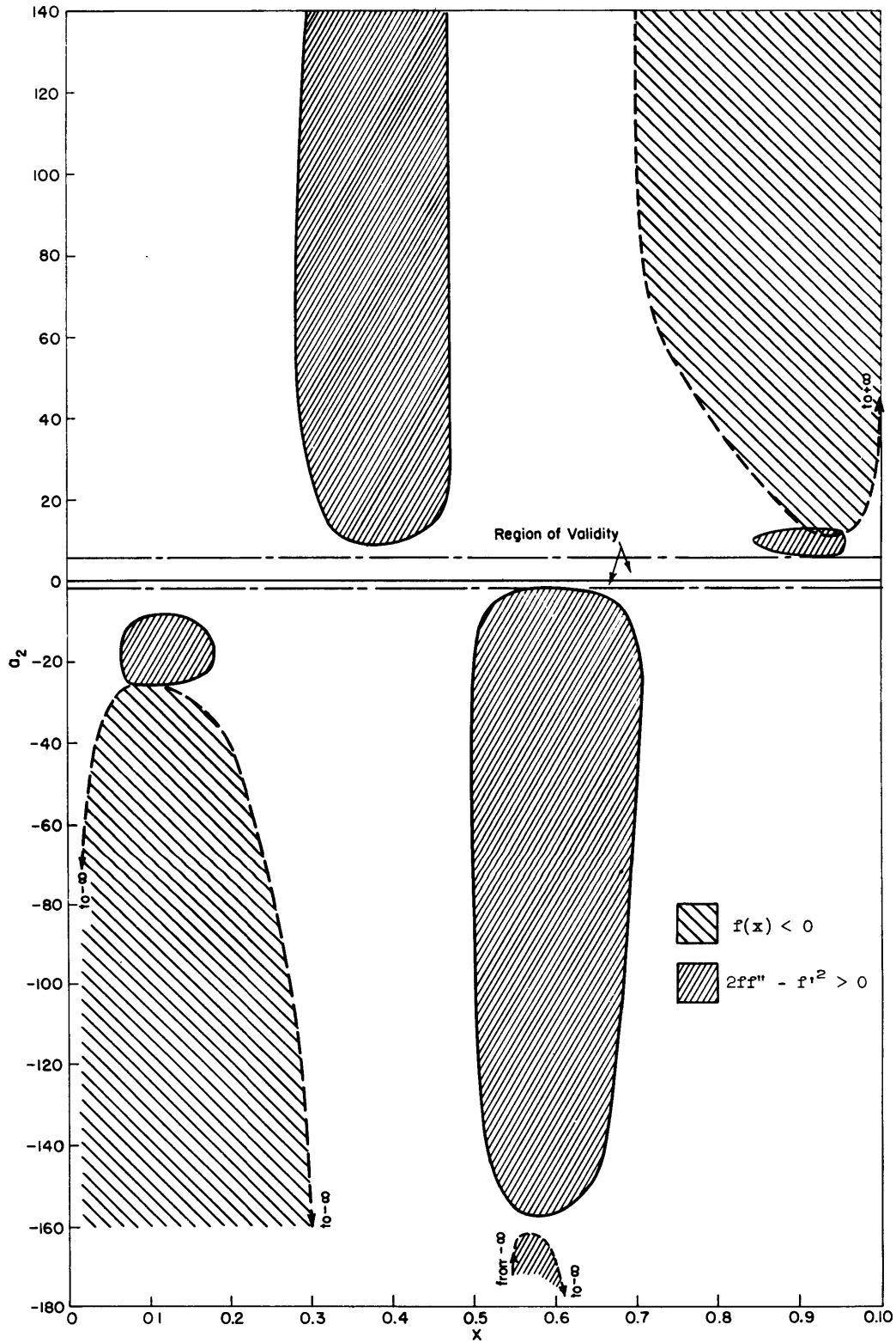
Figure 5 - Boundary Curves Defined by the No-Inflexion-Point Condition
