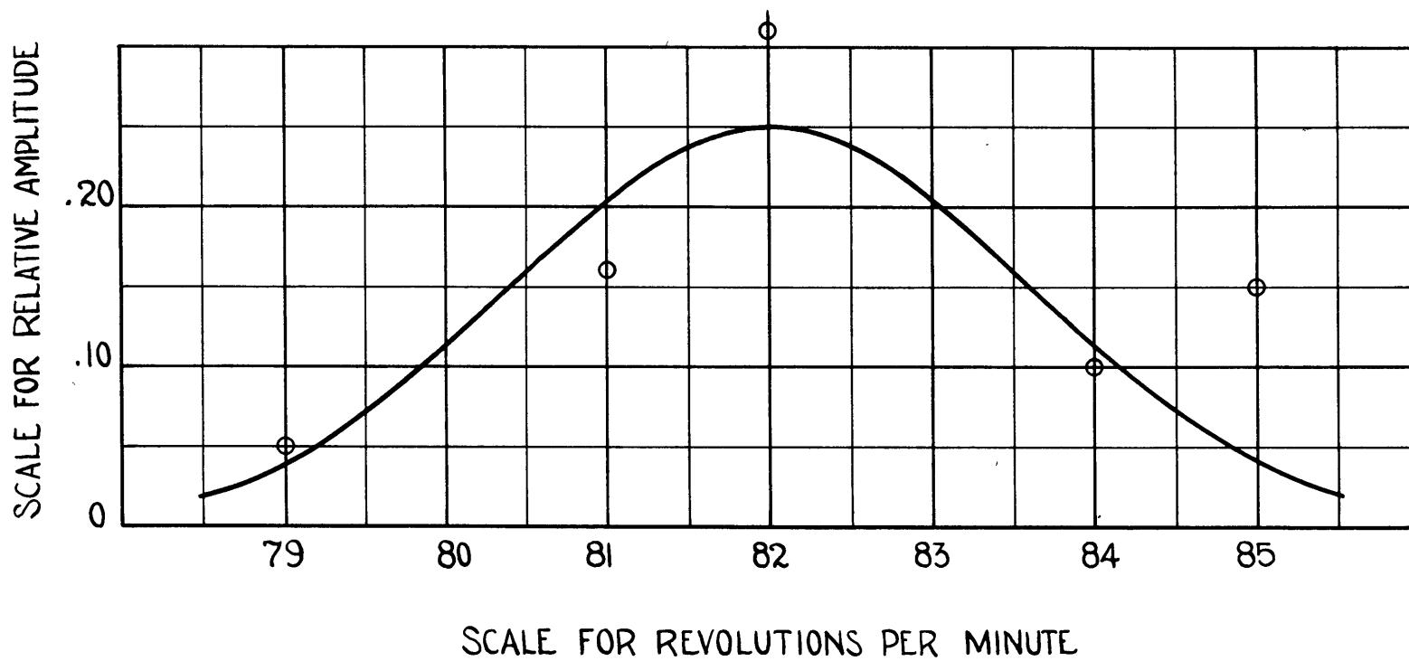
U.S.S. OKLAHOMA. RESONANCE CURVE
