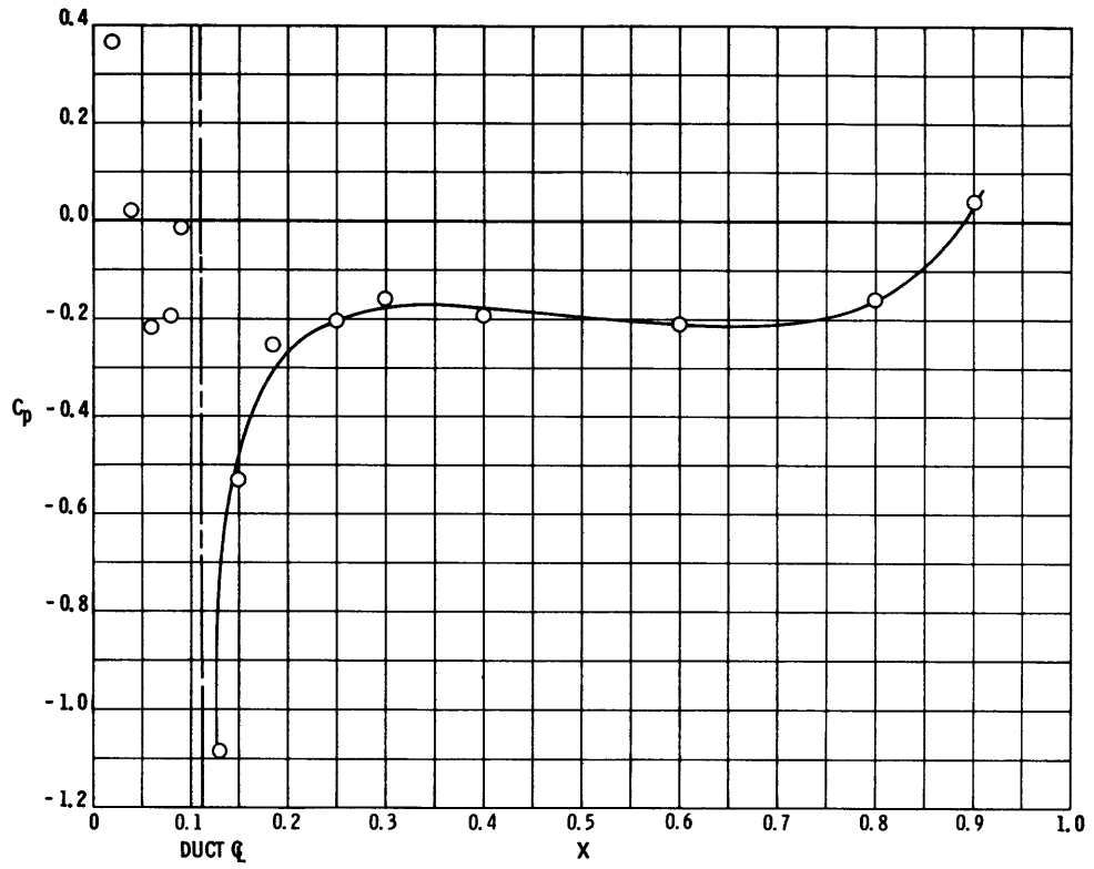
Figure 16e - At U_\infty/U_j = 1.39
