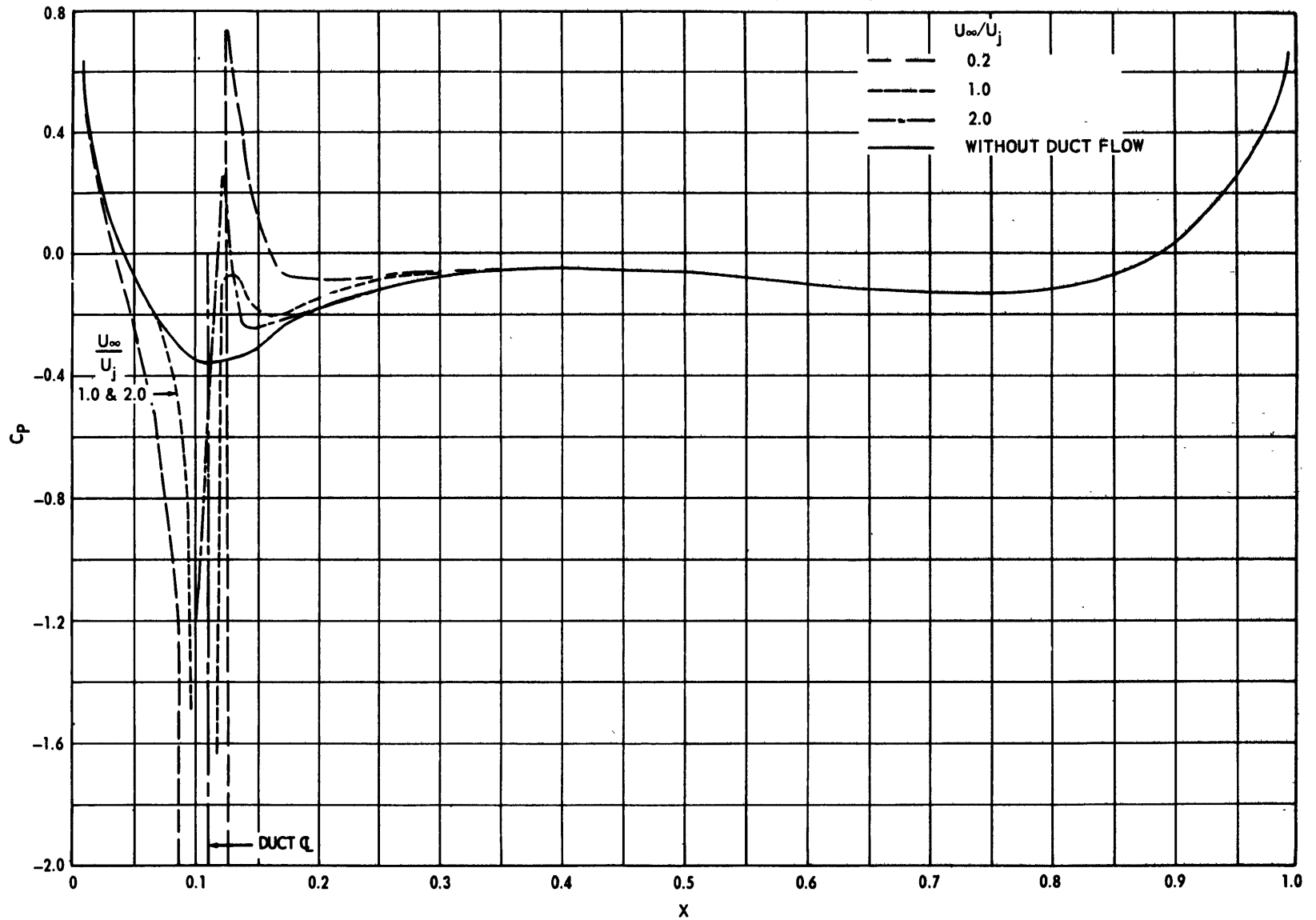
Figure 6a - Pressure Distribution
