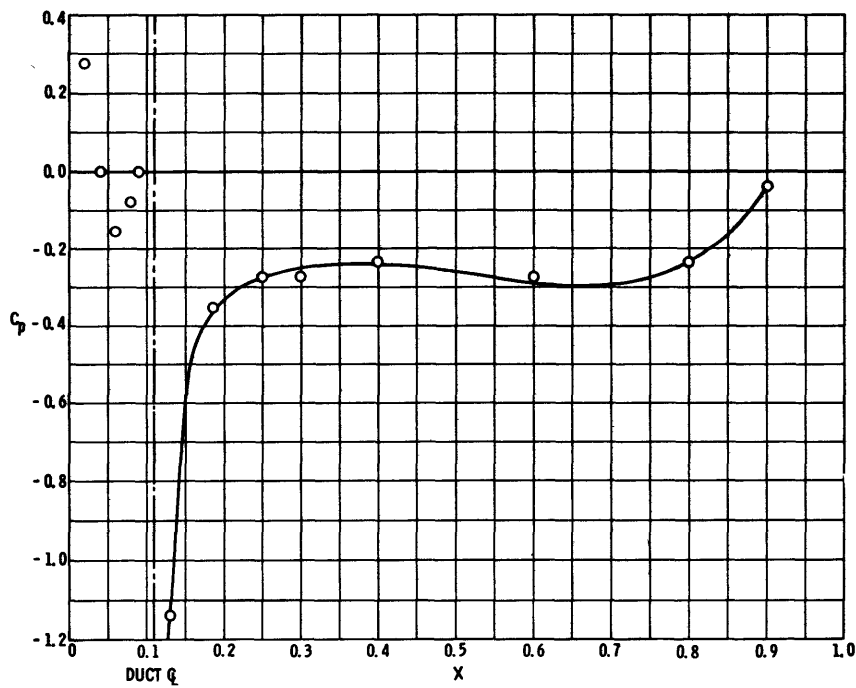
Figure 14d - At U_\infty/U_j = 0.979
