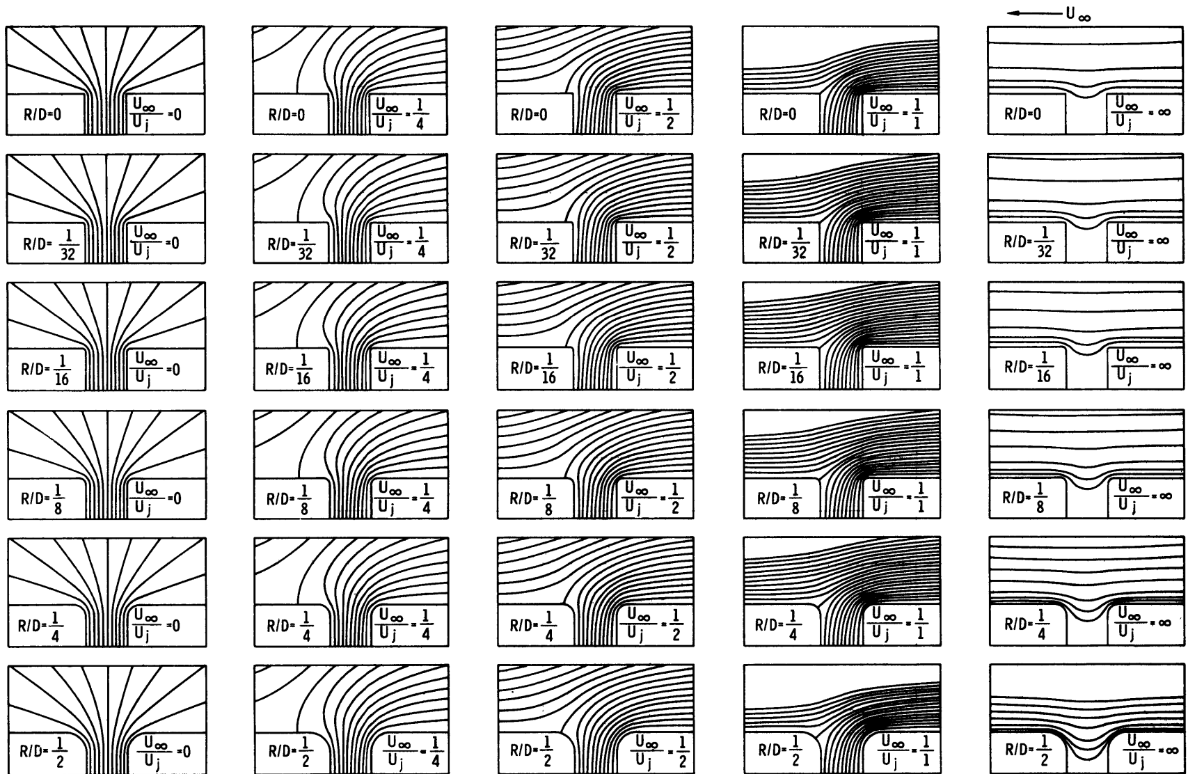
Figure 5 - Streamline Patterns, Inflow
