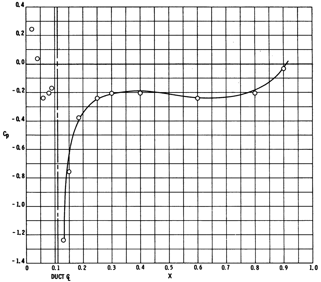
Figure 16a - At U_\infty/U_j = 0.245
