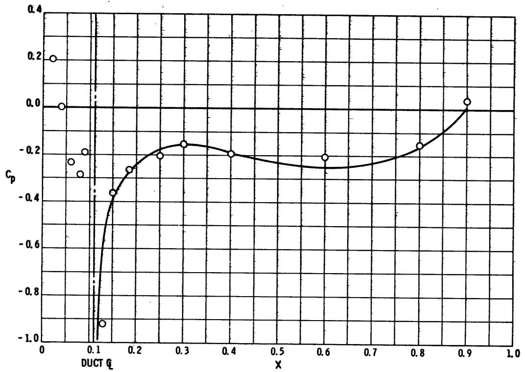
Figure 15e - At U_\infty/U_j = 0.999
