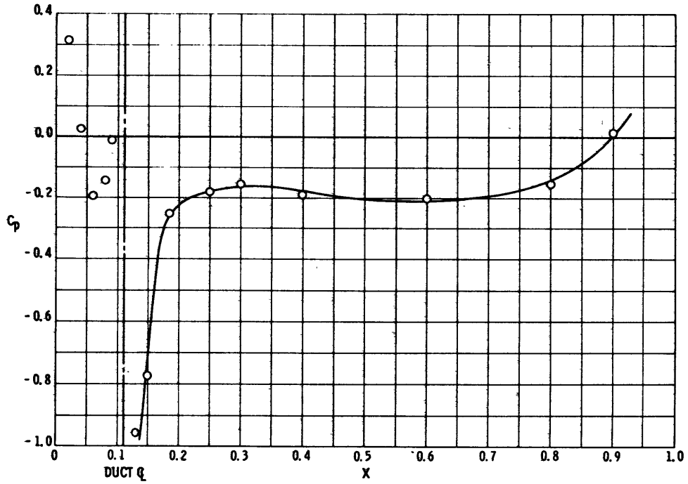
Figure 14f - At U_\infty/U_j = 1.78
