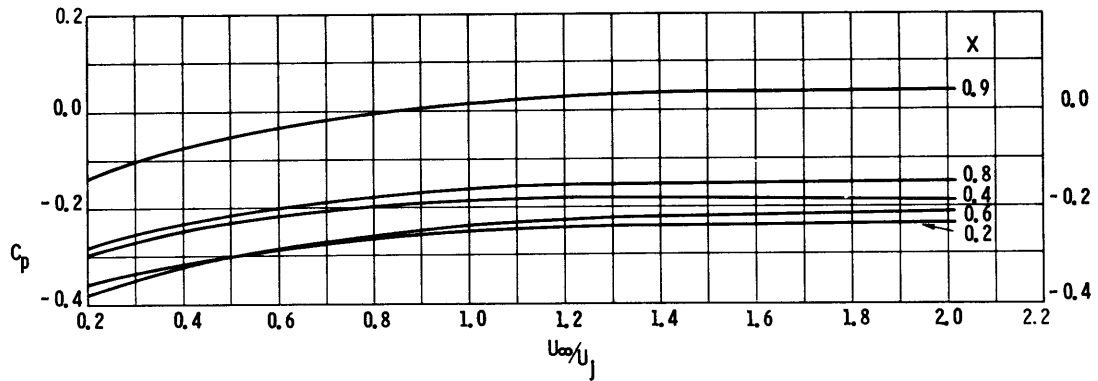
Figure 18 - Experimental Pressure Distribution for Outflow versus Velocity Ratio, 2-Inch Duct
