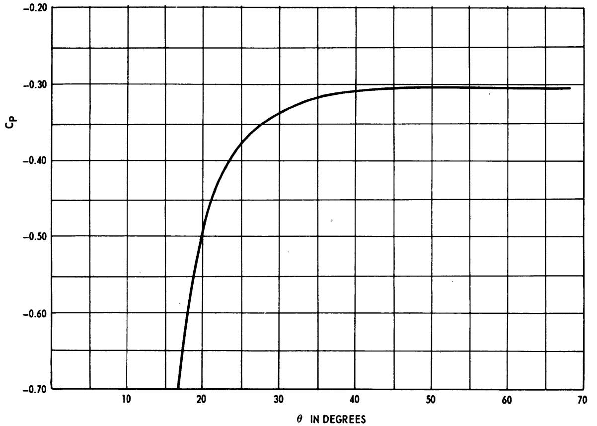
Figure 7 - Circumferential Variation for Duct Inflow of 4-Inch Duct at x = 0.107 , U_\infty/U_j = 0.2
