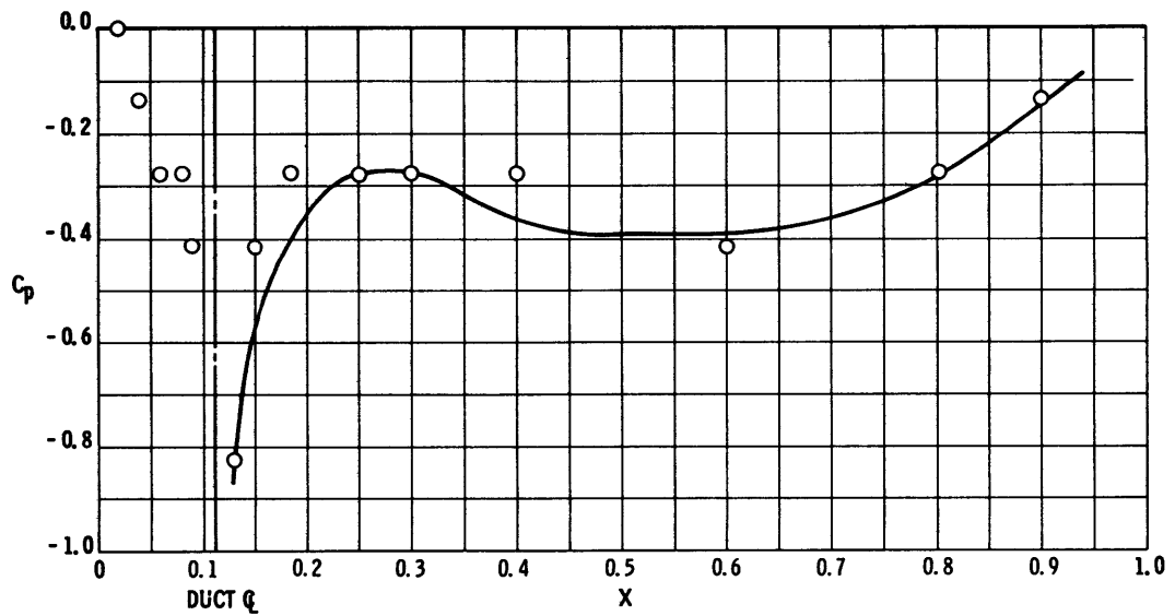
Figure 15b - At U_\infty/U_j = 0.200
