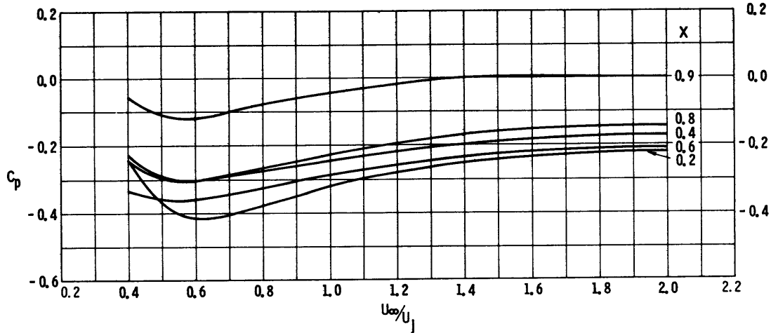
Figure 17 - Experimental Pressure Distribution for Outflow versus Velocity Ratio, 4-Inch Duct
