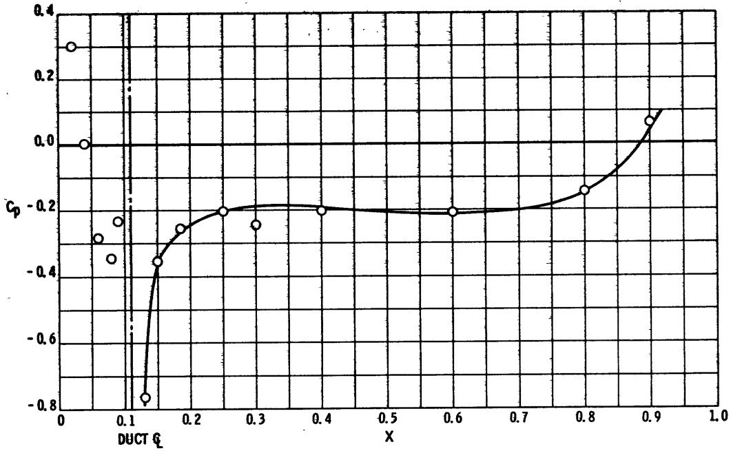
Figure 15g - At U_\infty/U_j = 1.81
