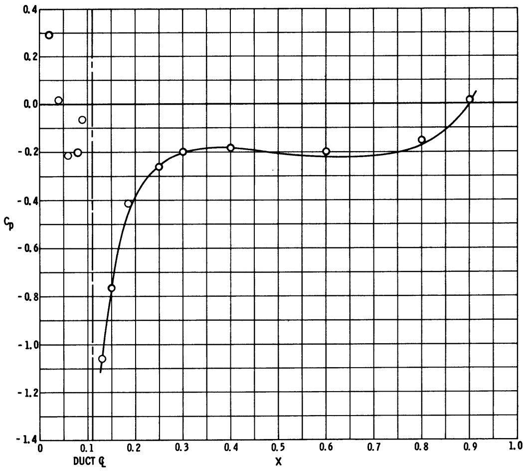
Figure 16b - At U_\infty/U_j = 0.391
