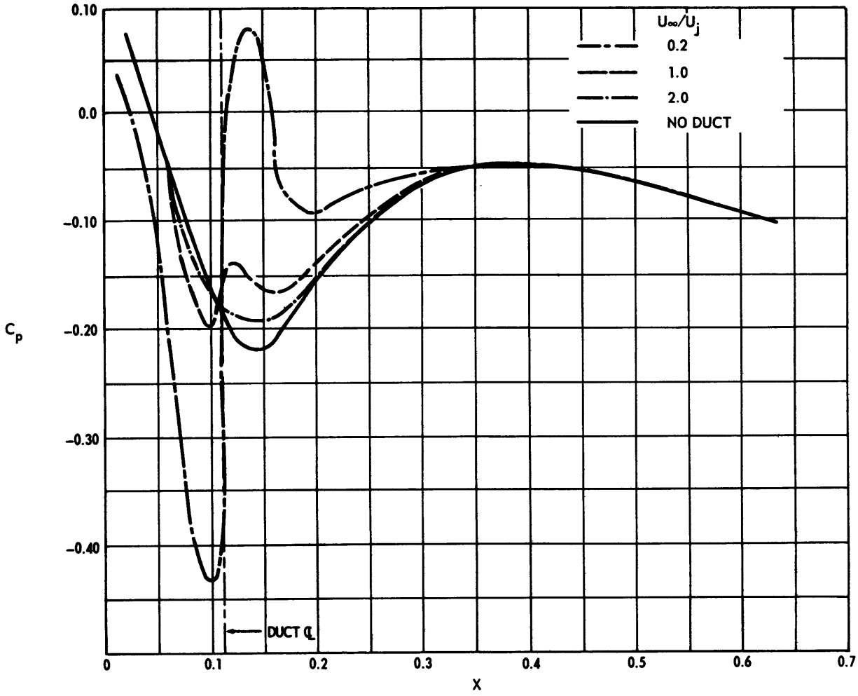
Figure 9 - Pressure Distribution off Body, Duct Entrance Flow for 4-Inch Duct at y = 0, z = 0.11
