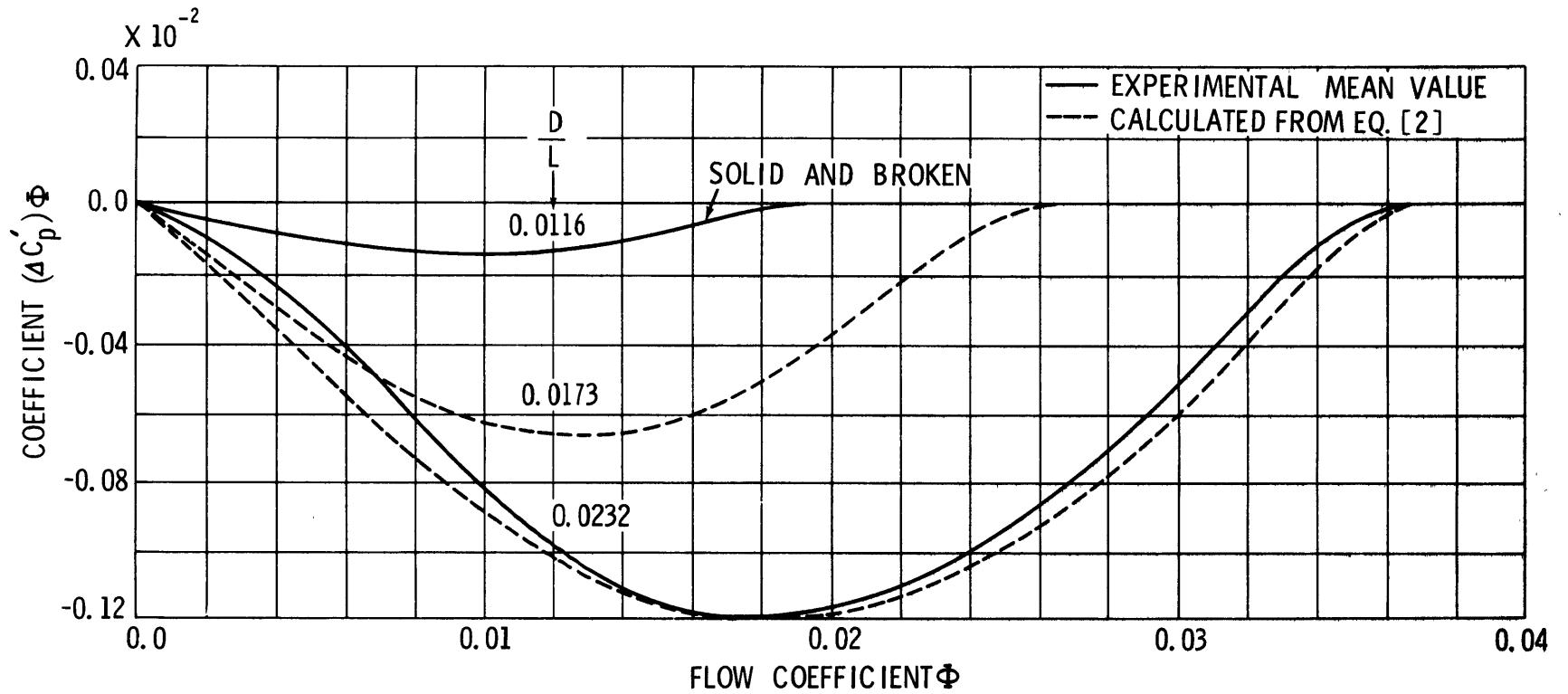
Figure 24 - Generalized Outflow Characteristics
