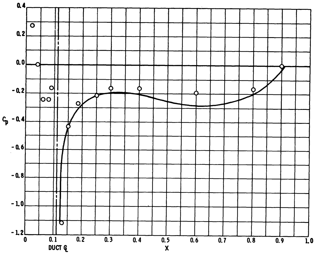
Figure 15d - At U_\infty/U_j = 0.617
