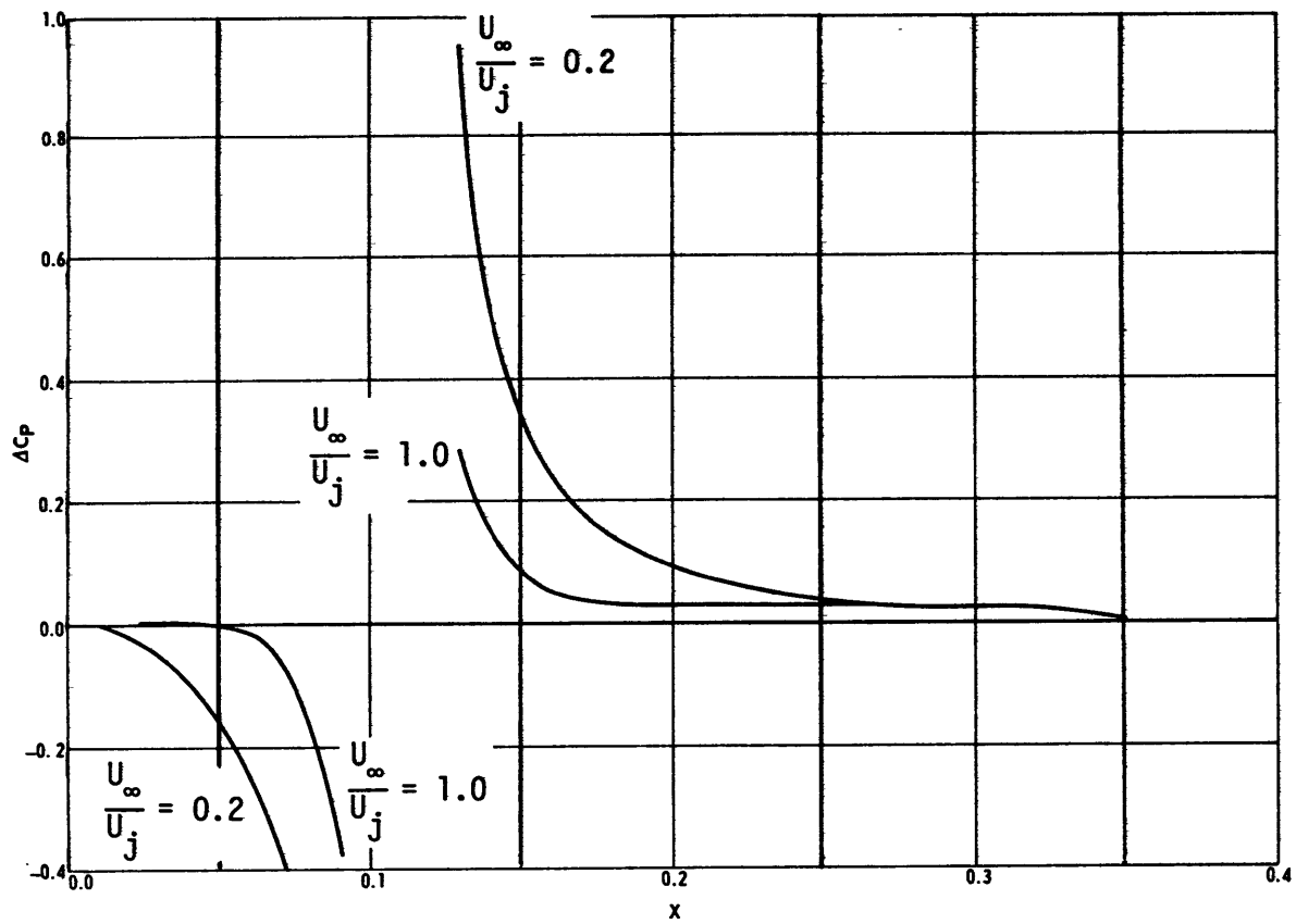
Figure 6b - Pressure Defect
