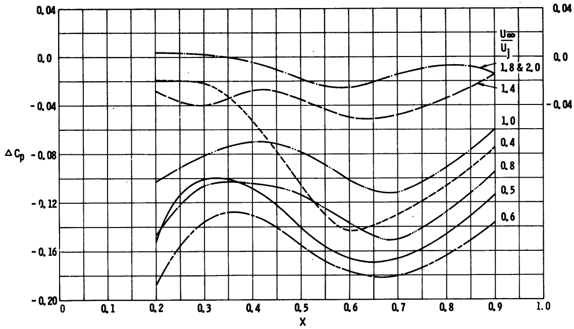
Figure 20 - Pressure Defect Associated with Outflow versus Longitudinal Position, 4-Inch Duct
