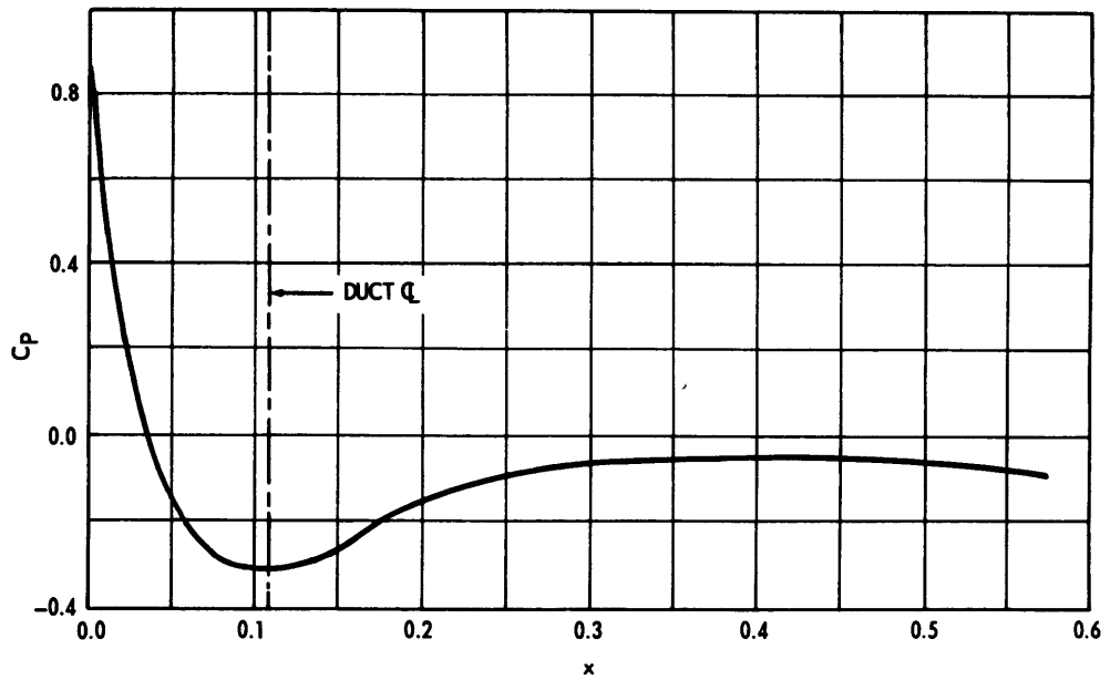
Figure 8 - Pressure Distribution along 45-Degree Meridian, Duct Entrance Flow for 4-Inch Duct at U_\infty/U_j = 0.2
