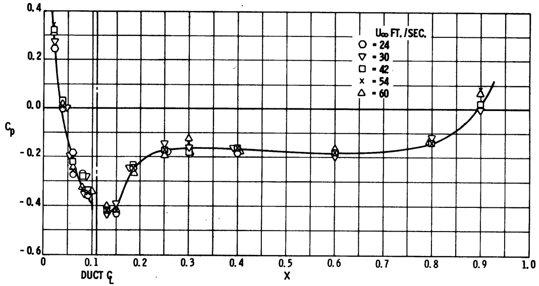
Figure 14a - At U_j = 0.0
