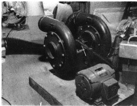
Figure 4 - Blower for Thruster-Duct Flow with Smoke Generator for Smoke Injection into Inlet
