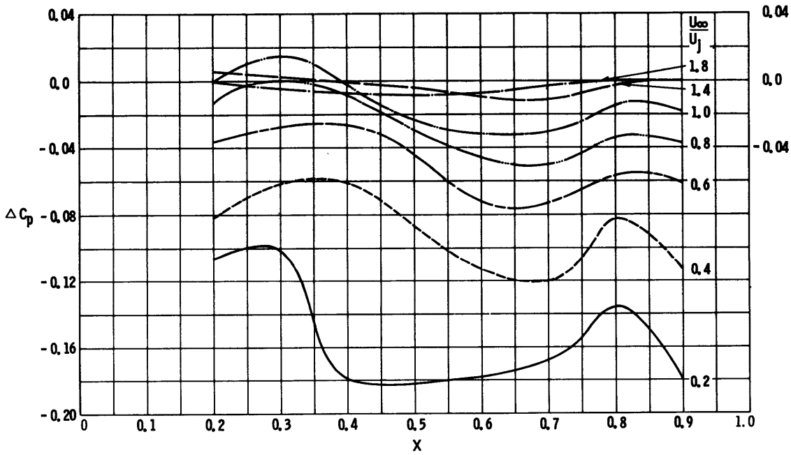
Figure 21 - Pressure Defect Associated with Outflow versus Longitudinal Position, 2-Inch Duct
