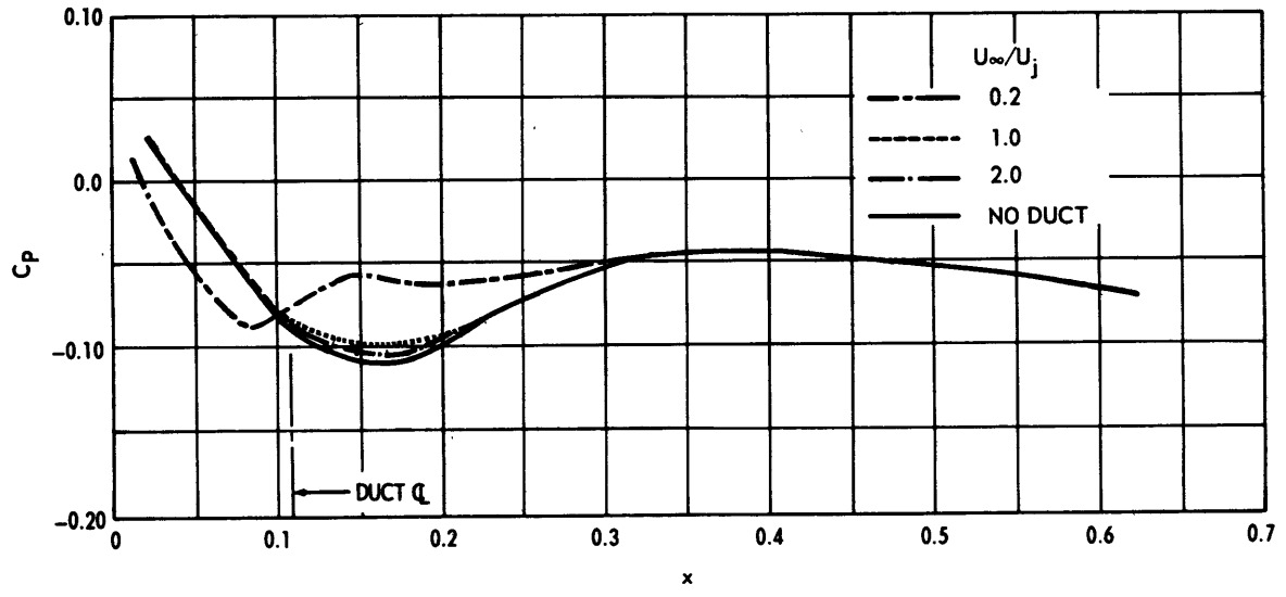
Figure 10 - Pressure Distribution off Body, Duct Entrance Flow for 4-Inch Duct at y = 0, z = 0.15
