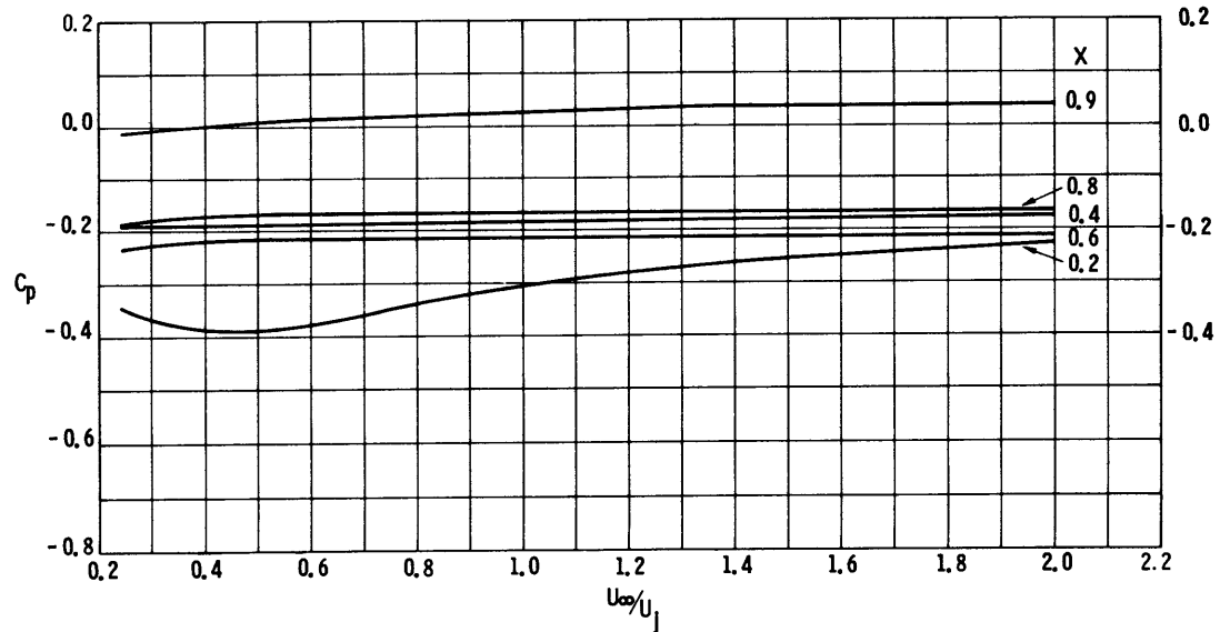
Figure 19 - Experimental Pressure Distribution for Outflow versus Velocity Ratio, 2-Inch Duct with Extension
