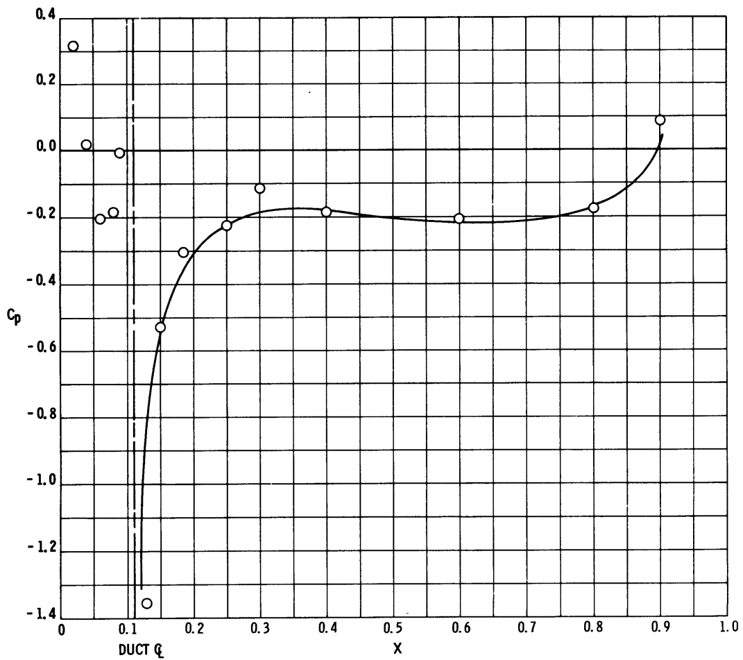
Figure 16d - At U_\infty/U_j = 0.985
