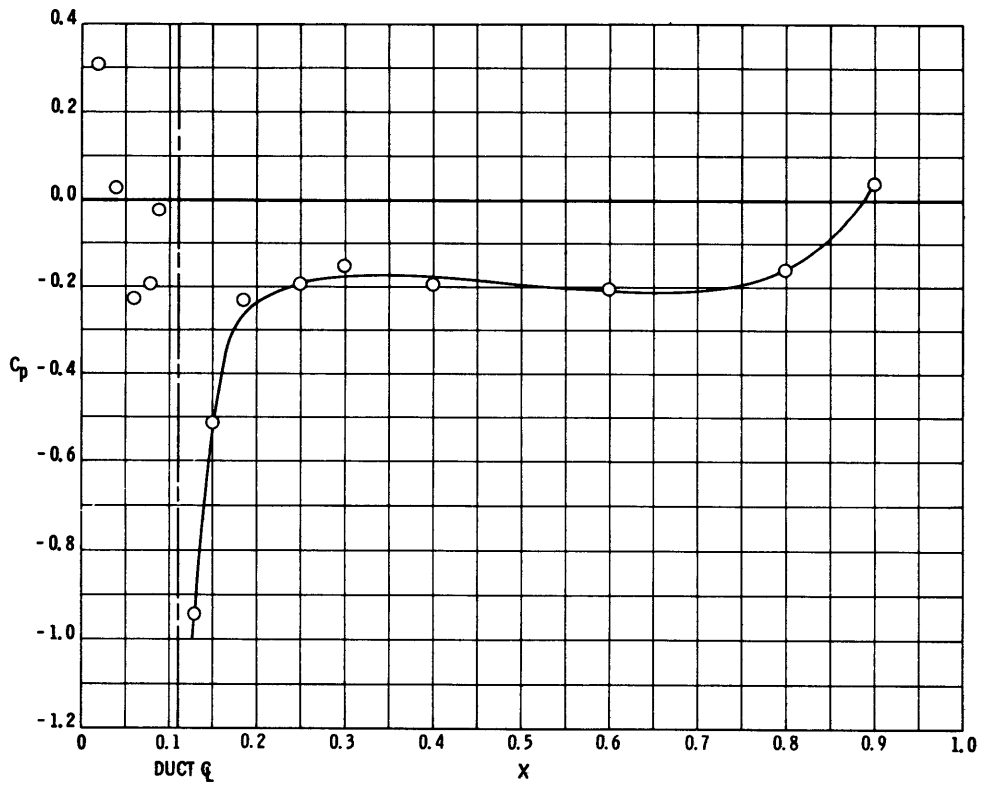
Figure 16f - At U_\infty/U_j = 1.86
