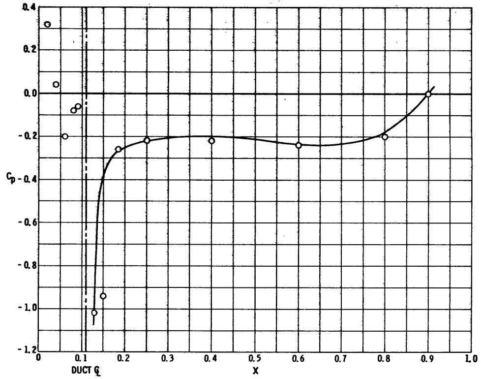
Figure 14e - At U_\infty/U_j = 1.39
