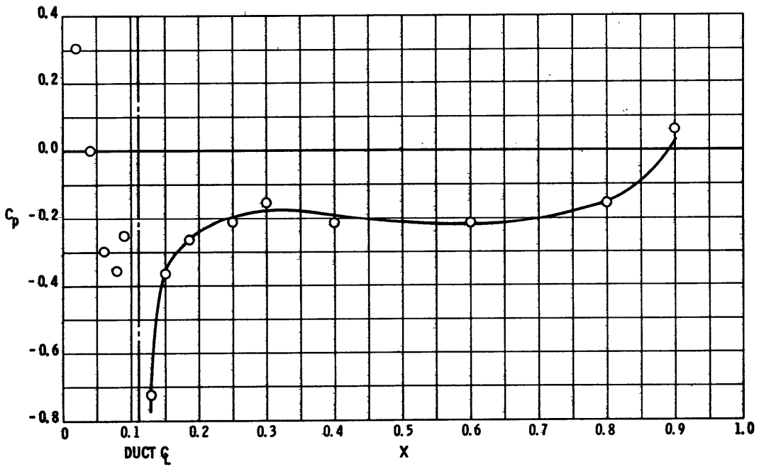
Figure 15h - At U_\infty/U_j = 2.02
