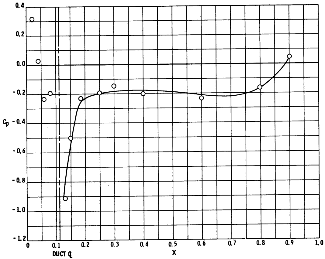
Figure 16g - At U_\infty/U_j = 2.05
