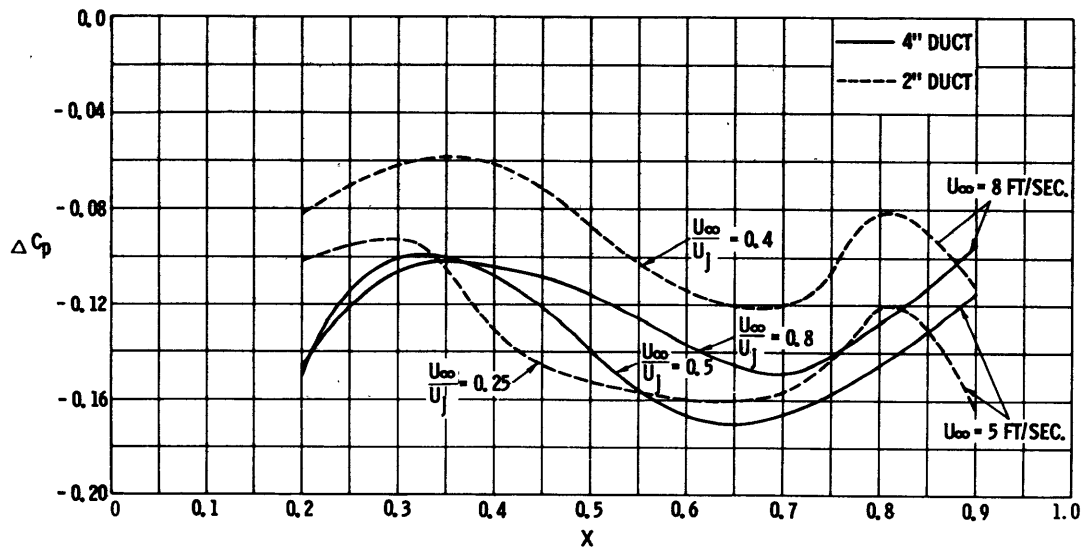
Figure 23 - Comparative Pressure Defects Associated with Outflow
