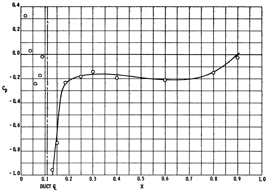
Figure 14g - At U_{\infty}/U_j = 2.00
