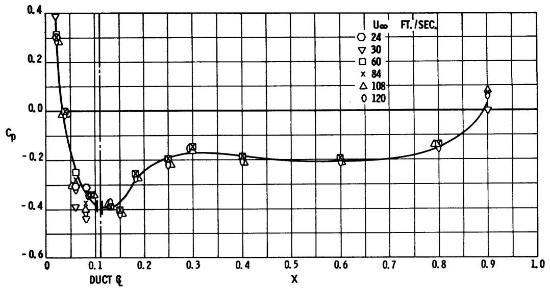
Figure 15a - At U_j = 0.0
