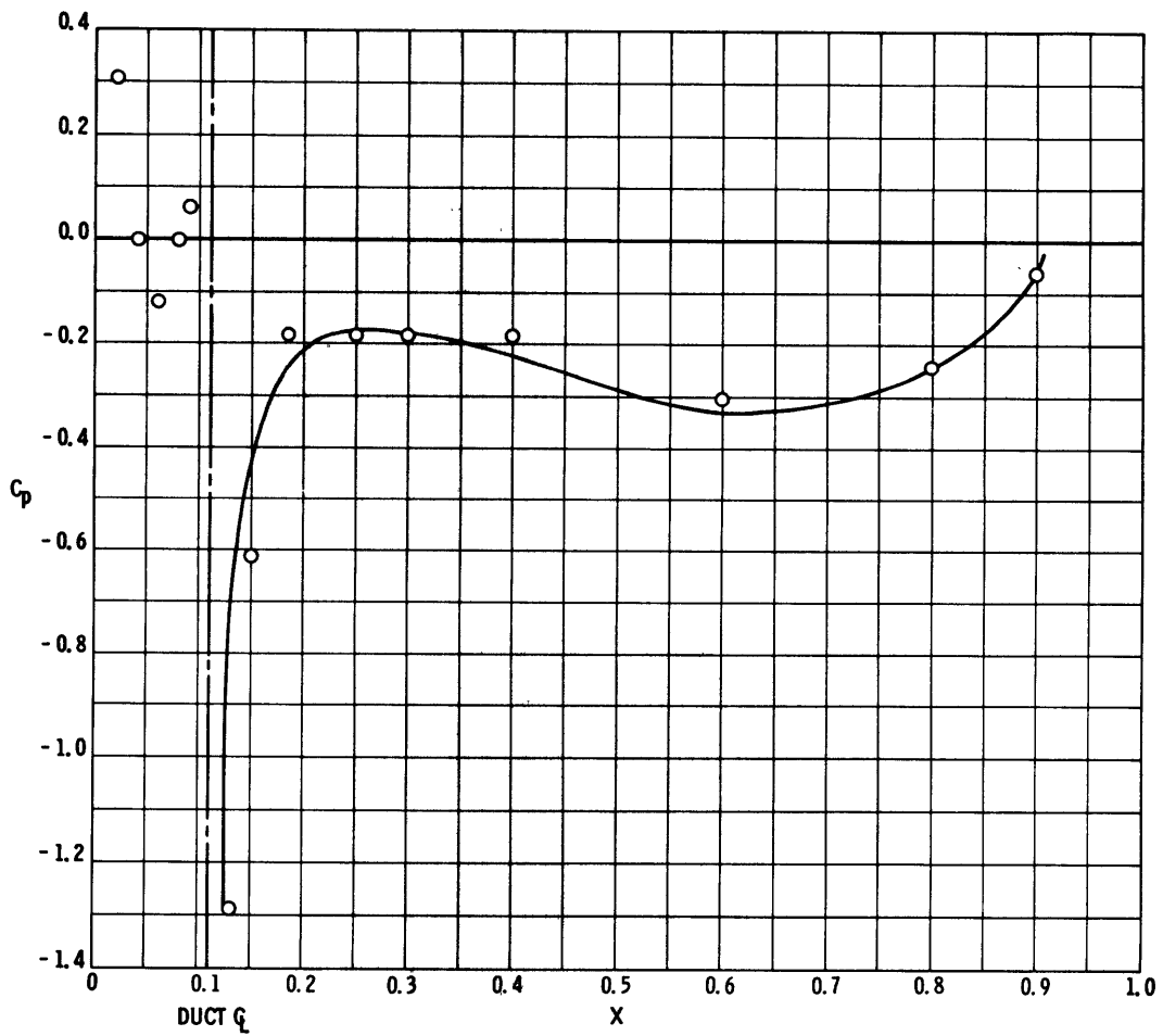
Figure 14b - At U_\infty/U_j = 0.398
