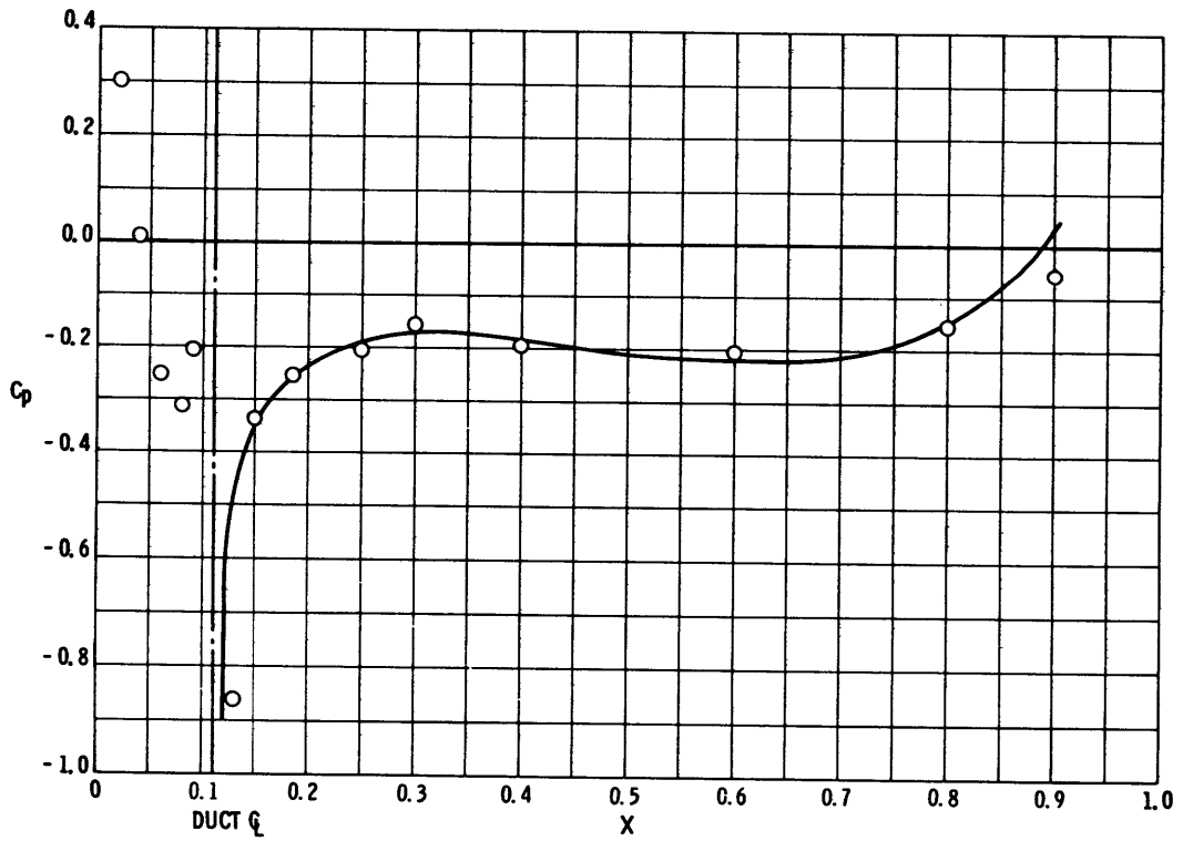
Figure 15f - At U_\infty/U_j = 1.39
