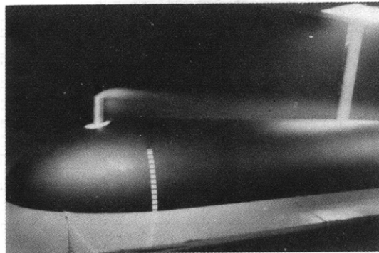
Figure 13 - Wind Tunnel Jet Flow, 2-Inch Duct with Extension
