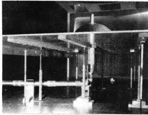
Figure 3 - Extension of Duct below Ground Board to Obtain Full Duct Length
