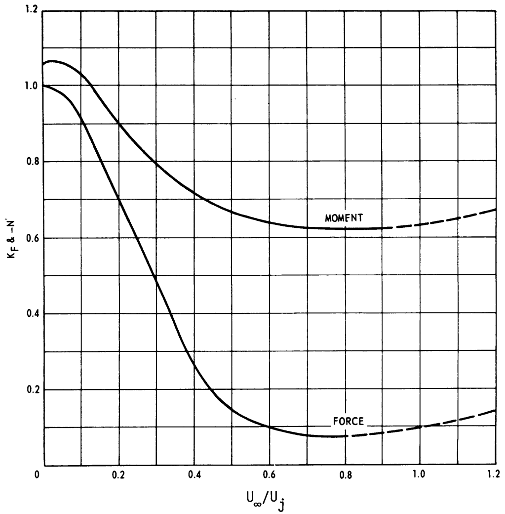
Figure 1 - Estimated Body-Force and Body-Moment Coefficients for a Submersible with a Bow Thruster
