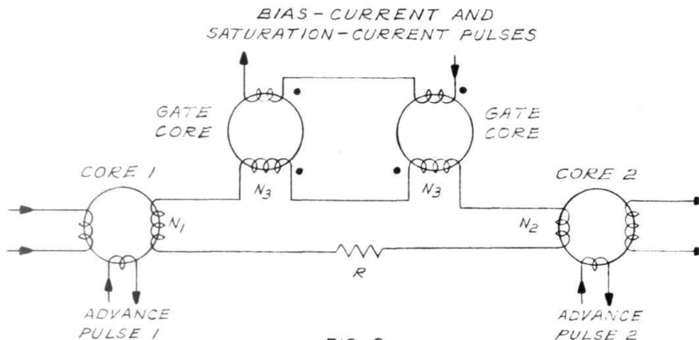
FINAL CIRCUIT OF MAGNETIC-CORE GATE IN A STEPPING REGISTER
